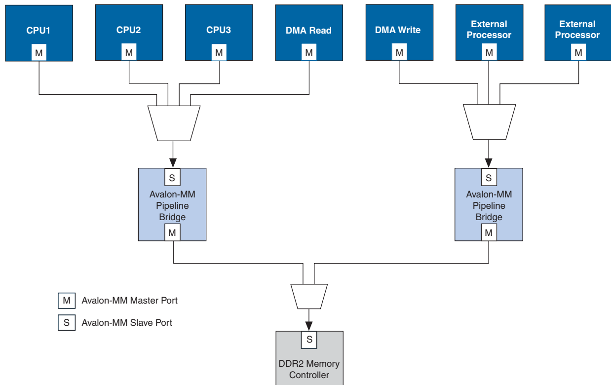
Figure 11-9. Seven Avalon-MM Masters Accessing One Avalon-MM Slave
