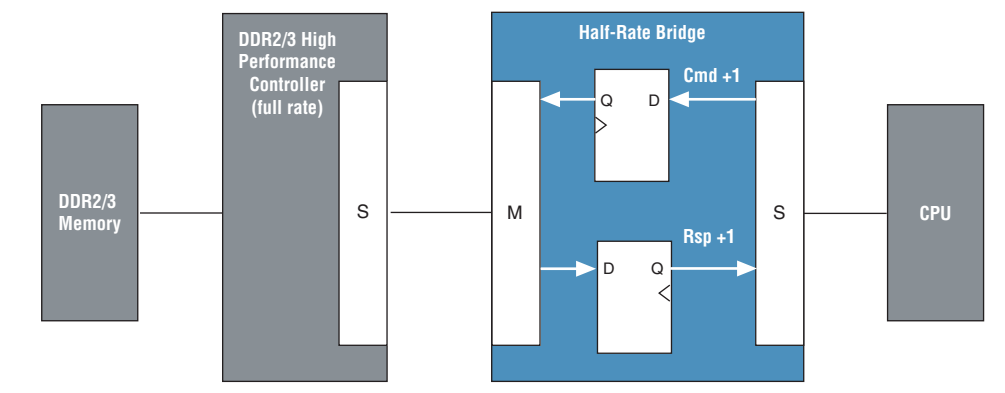
Figure 11-15. Avalon-MM DDR Memory Half-Rate Bridge Block Diagram
