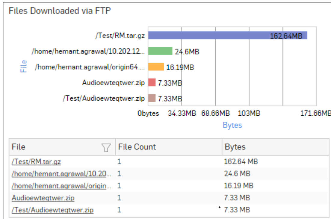
Figure 153: Files Downloaded via FTP
