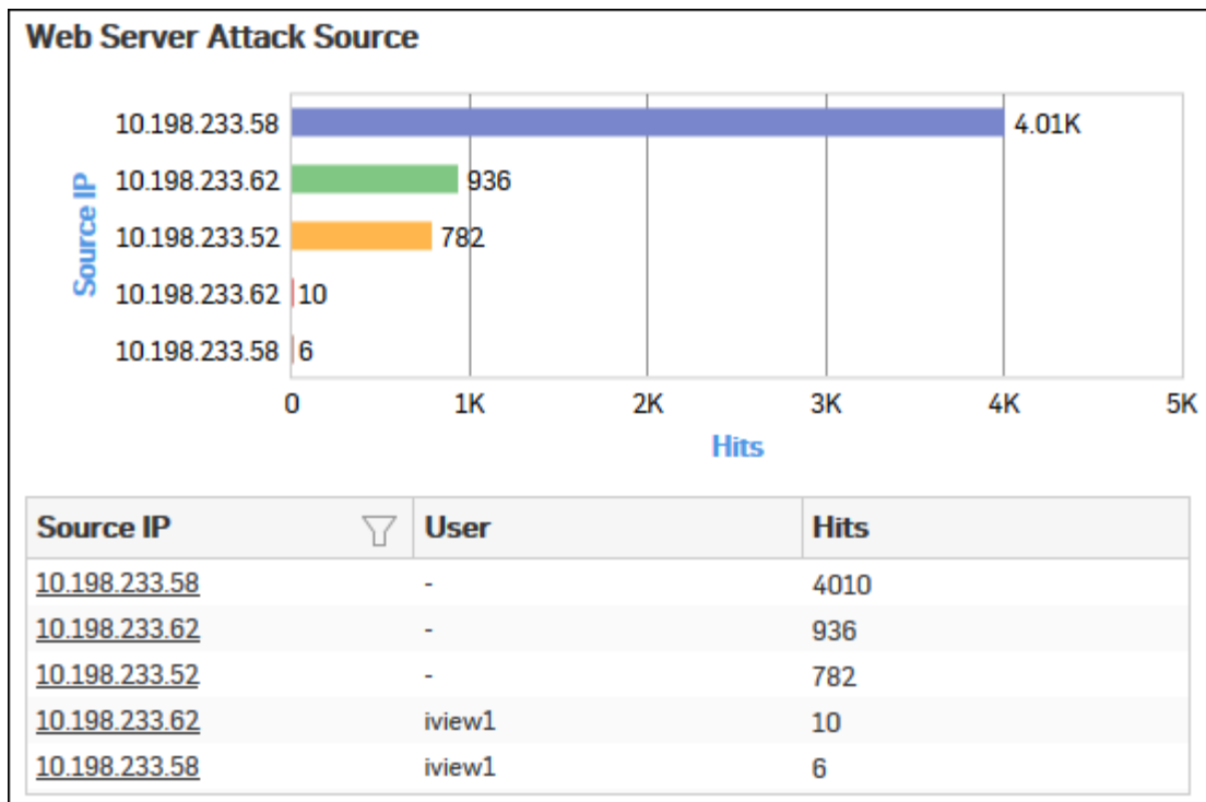
Figure 146: Web Server Attack Source
