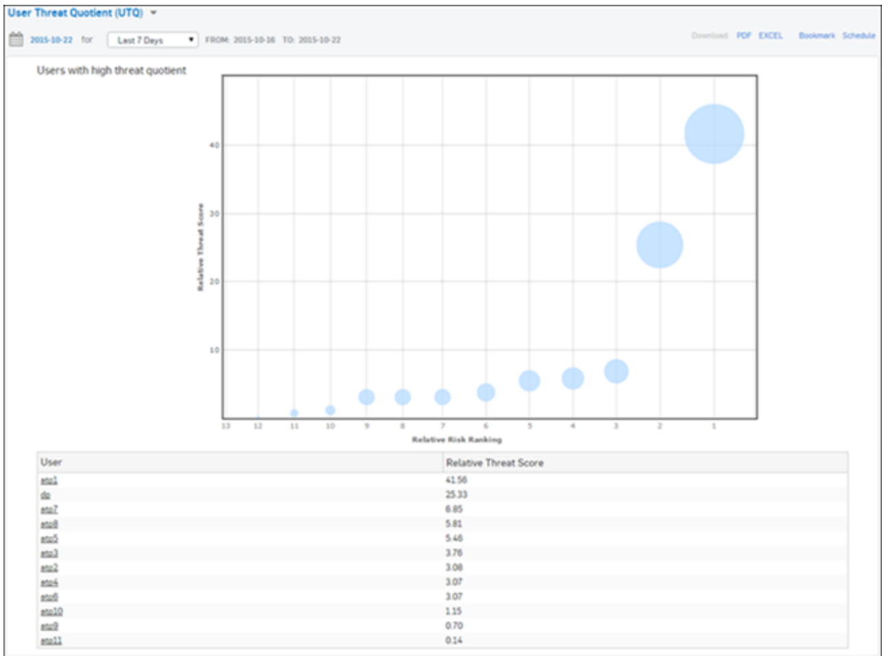
Figure 68: User Threat Quotient (UTQ)
