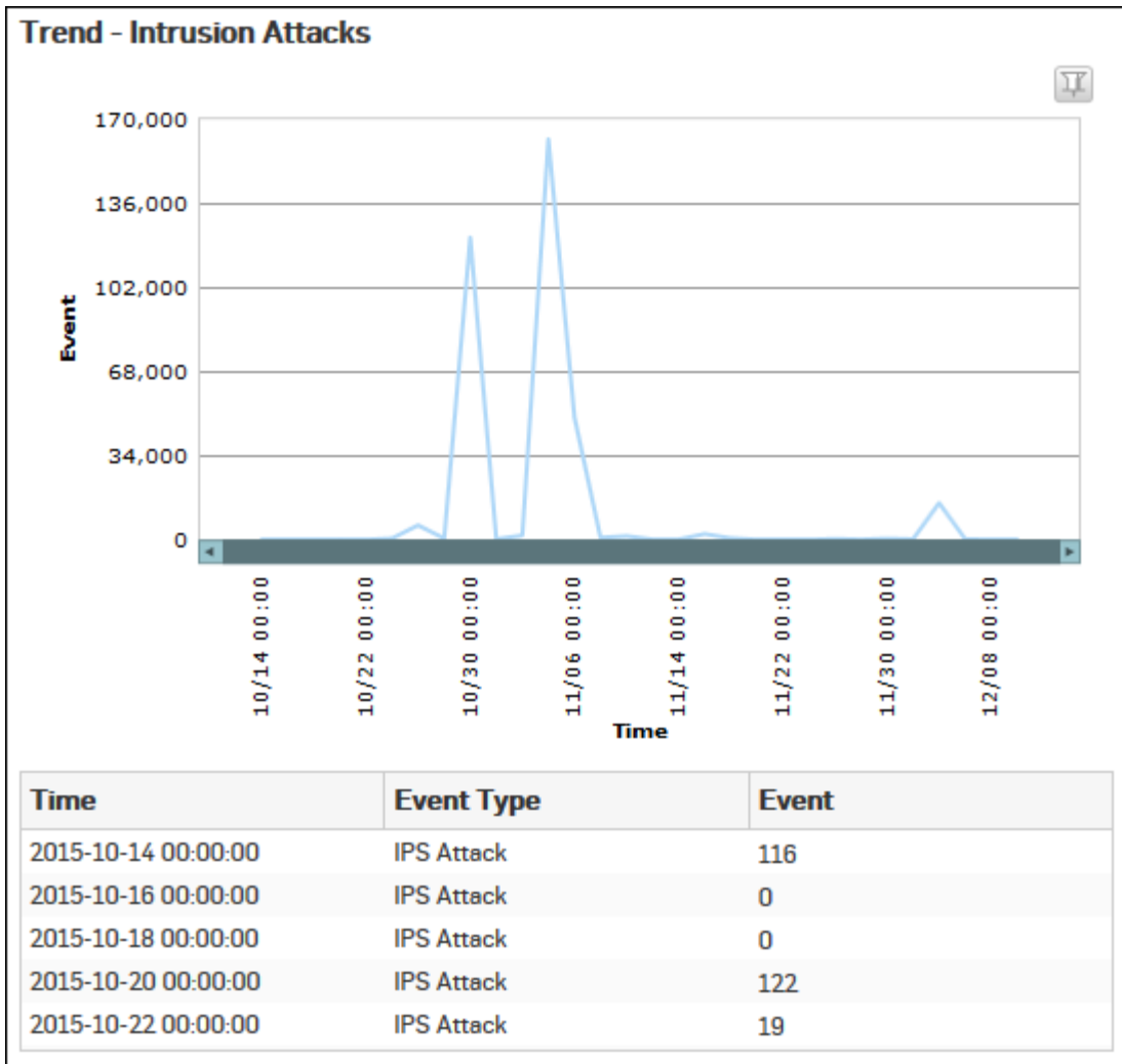
Figure 176: Trend - Intrusion Attacks
