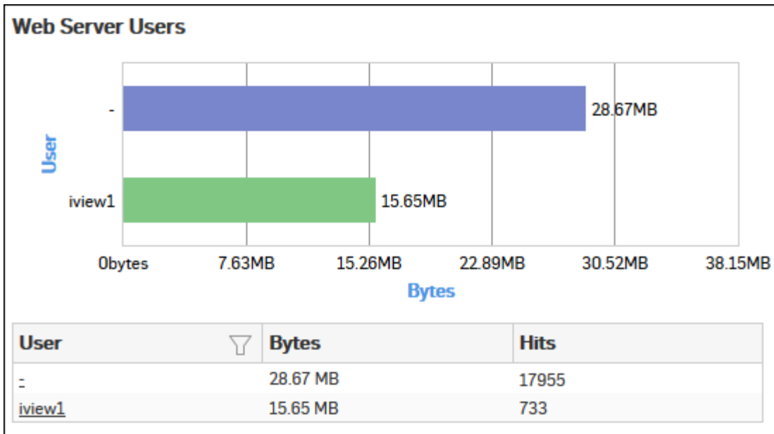
Figure 290: Web Server Users
