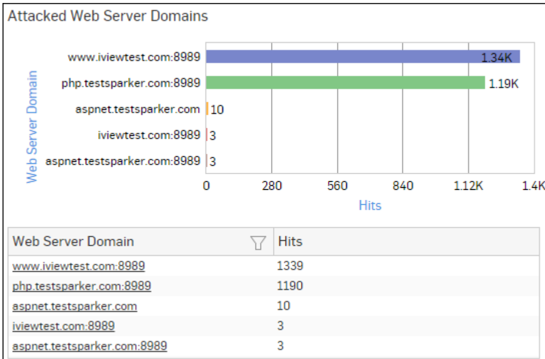
Figure 38: Attacked Web Server Domains
