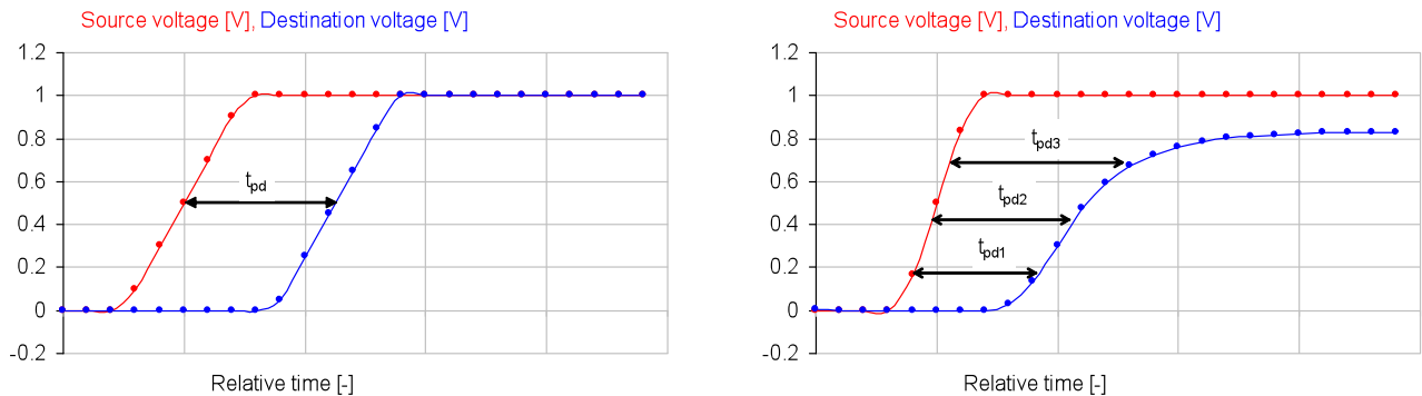
Figure 1: Illustration of delay definitions with ideal edges (on the left) and with different reference and target waveforms (on the right).
