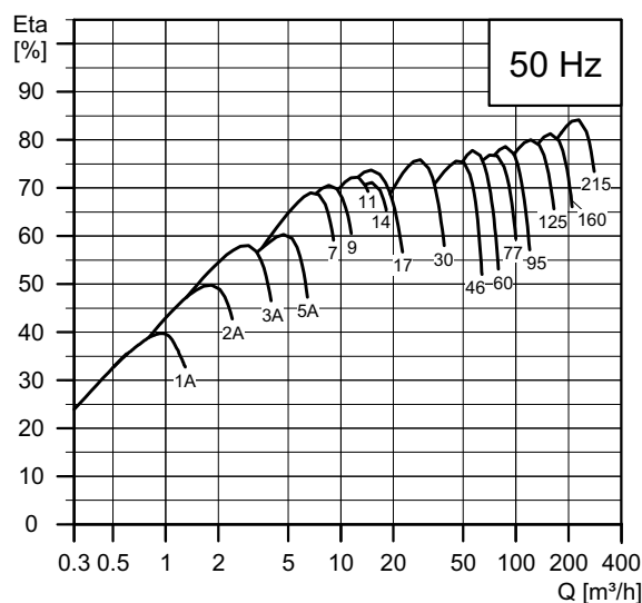
Fig. 1 Pump efficiencies in relation to flow
