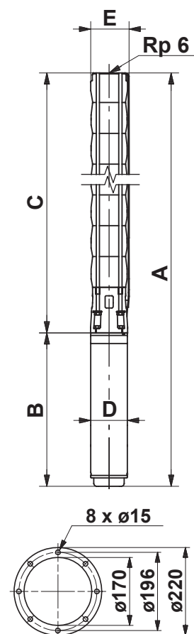
Pump with Grundfos flange
