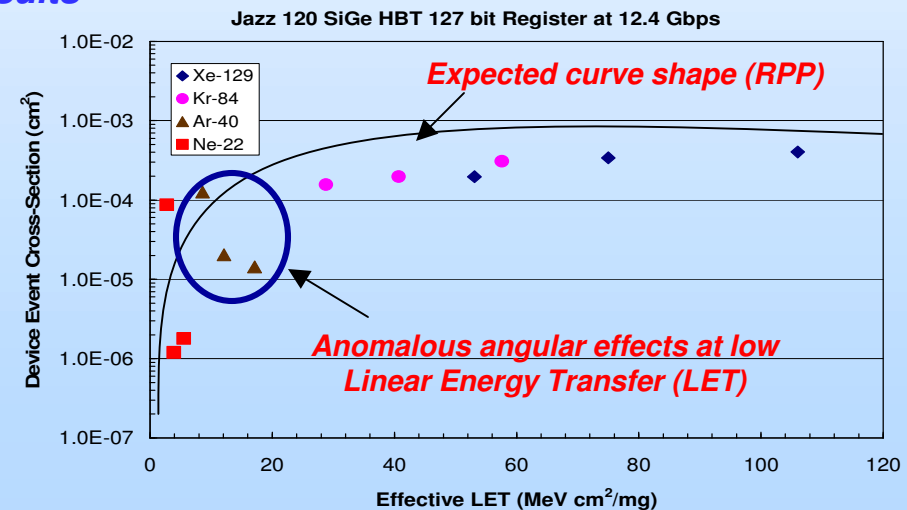
RPP model does not fit SiGe
