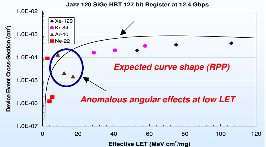
Effects of heavy ions on SiGe devices at 12 GHz speeds; Drawn line represents expected response with "standard" models.
