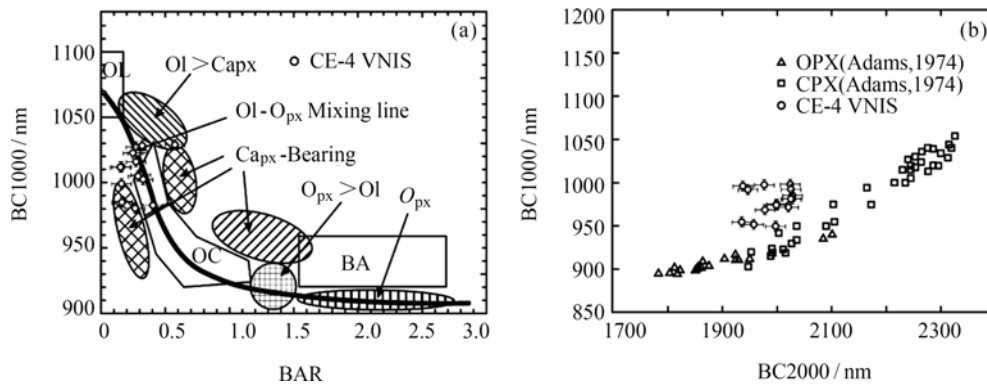
Fig. 8 Scatter plots of spectral parameters. (a) BAR–BC1000; (b) BC2000–BC1000. Reference compositional groups are from Cloutis et al. (1986) and Adams (1974), respectively. The error bars in each plot represent a first-order approximation for the uncertainty determined by the law of propagation of uncertainty. Here OC represents ordinary chondrites and BA represents pyroxene dominated basaltic achondrites
