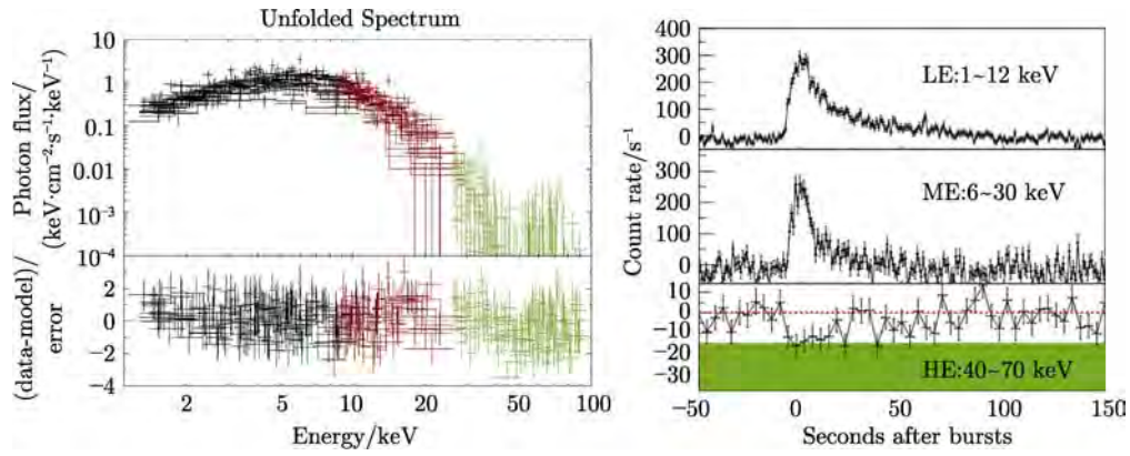
Fig. 9 Spectrum and light curves of Type-I X-ray burst of 4U 1636-536 [11] .
