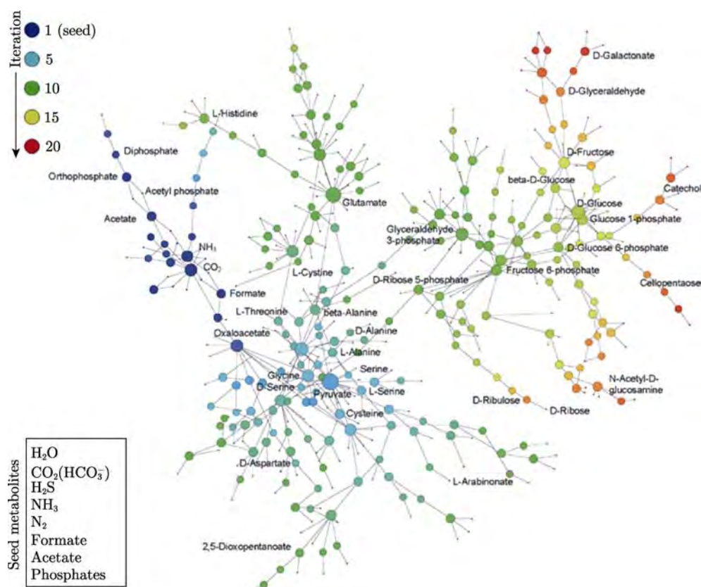
Fig. 3 Construction of phosphorus-dependent metabolic network. Network expansion simulation was executed using a set of defined seed compounds and all balanced reactions in the background metabolism pool derived from the updated KEGG reactions. The figure displays the obtained phosphorus-dependent network in which metabolites are linked if they have a reactant-product relationship during the expansion. The metabolites generated at different iteration steps during the network expansion process are represented by nodes in different colors. The size of node represents the degree of the node, i.e. , the number of reactions added in the subsequent iteration
