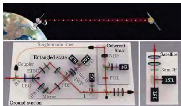
Fig. 2 Experimental test of gravitationally induced quantum decoherence
