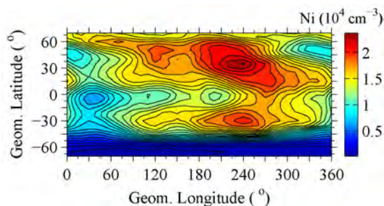
Fig. 7 Geomagnetic longitude and latitude variations of the ion density at 840 km measured by the DMSP F12 satellite at nightside 21:30 LT around the June solstice of 1996 (after Chen et al. [19] )
