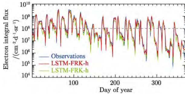
Fig. 9 Comparison among forecasting results of two categories of forecasting models and observations in 2008. The daily >2 MeV electron integral flux of 10^8 \text{ cm}^{-2} \cdot \text{d}^{-1} \cdot \text{sr}^{-1} over the entire time of each year is shown as a dark gray dashed curve. LSTM represents Long Short-Term Memory [14]
