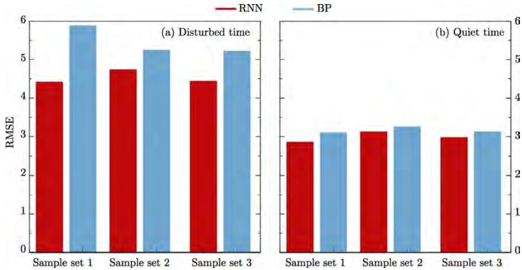
Fig. 7 Forecasting RMSE of TEC during magnetic disturbed time (a) and magnetic quiet time (b) in Beijing. Inputs are F_{10.7} , TEC and A_p for sample set 1, F_{10.7} , TEC, A_p , solar wind speed and IMF B_z for sample set 2 and F_{10.7} , TEC, solar wind speed and IMF B_z for sample set 3 [12]
