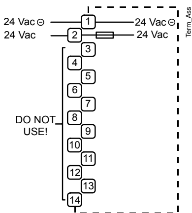
Fig. 4. Terminal block assignment
