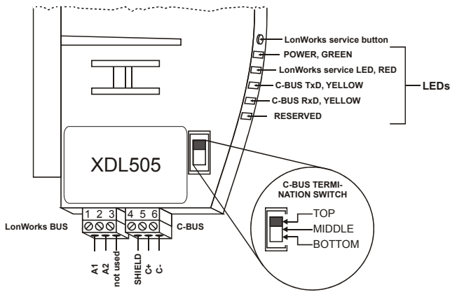
Fig. 2. XDL505 Application module LEDs and ports
