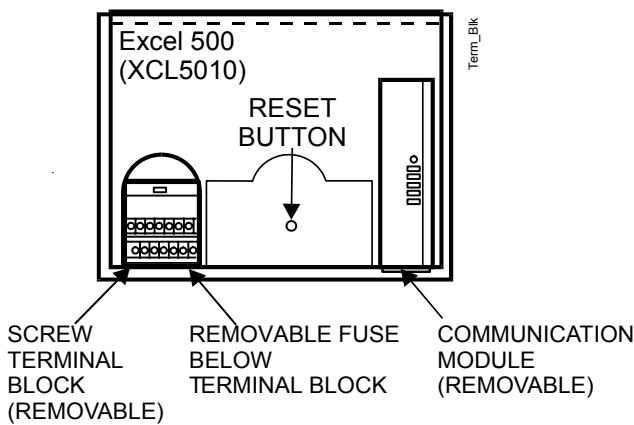
Fig. 3. Rear view of housing
