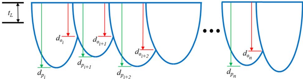
FIGURE 3. Top surface melt-pool geometry measurements
