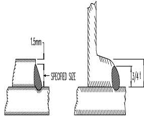
FILLET WELD APPLIED TO SQUARE EDGE OF PLATE OR ROUND TOP OF ROLLED SECTION
