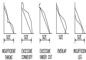
DEFECTIVE FILLET WELD PROFILE
