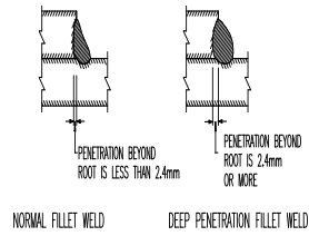
TYPES OF FILLET WELD
