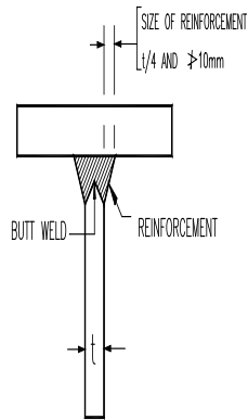
BUTT WELDED T JOINT
