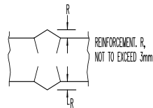
ACCEPTABLE BUTT WELD PROFILE
