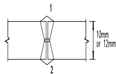
Sketch showing sequence of square butt welding
