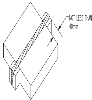
BUTT WELDED JOINT WITH RUN-ON AND RUN-OFF PLATES
