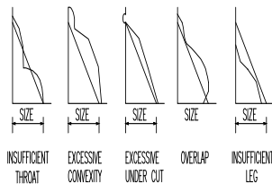
DEFECTIVE FILLET WELD PROFILE
