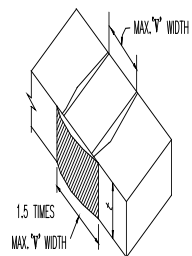
BUTT WELD END REINFORCEMENT
