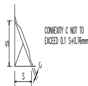
ACCEPTABLE FILLET WELD PROFILE
