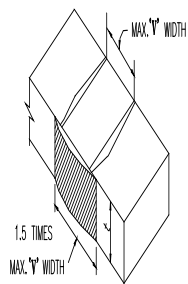
BUTT WELD END REINFORCEMENT
