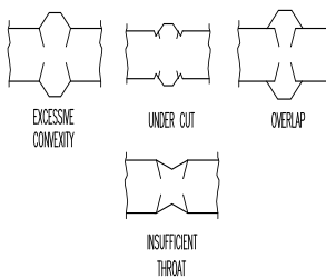
DEFECTIVE BUTT WELD PROFILES
