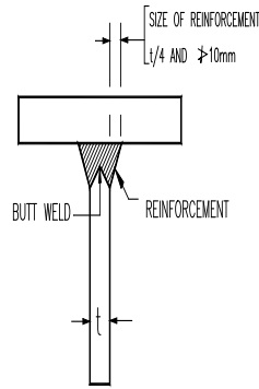
BUTT WELDED T JOINT
