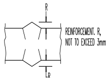
ACCEPTABLE BUTT WELD PROFILE
