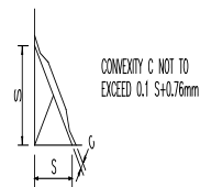
ACCEPTABLE FILLET WELD PROFILE
