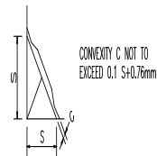
ACCEPTABLE FILLET WELD PROFILE
