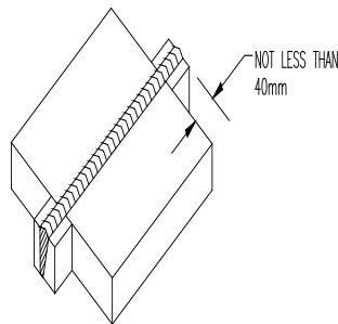
BUTT WELDED JOINT WITH RUN-ON AND RUN-OFF PLATES
