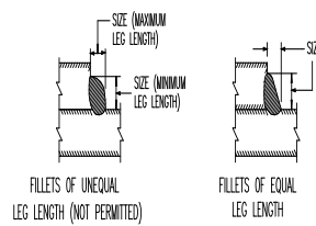
SIZE OF NORMAL FILLET WELDS
