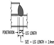
SIZE OF DEEP PENETRATION FILLET WELD
