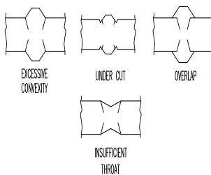
DEFECTIVE BUTT WELD PROFILES
