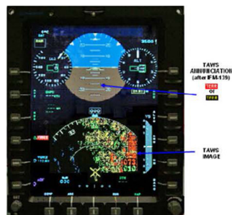
TAWS displayed as HSI underlay on PFD
