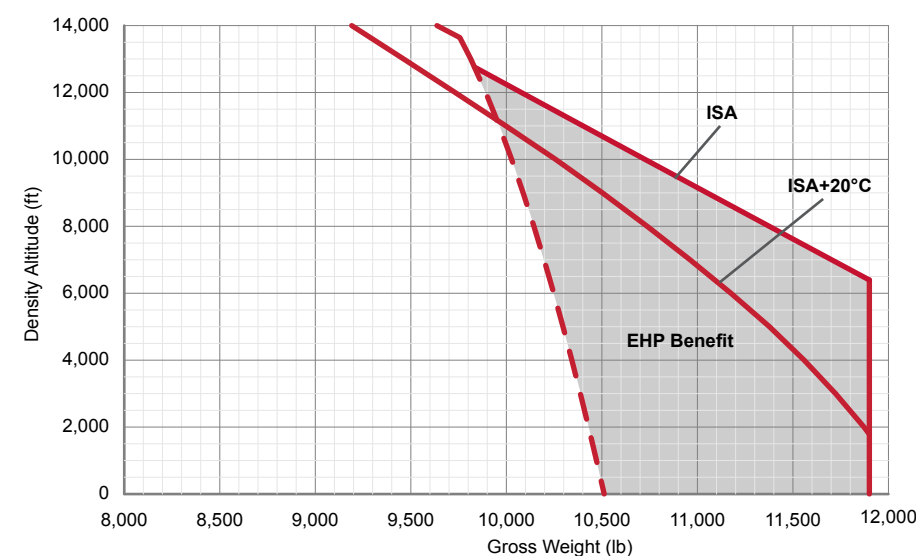
OGE Hover Capability at Maximum Continuous Power
