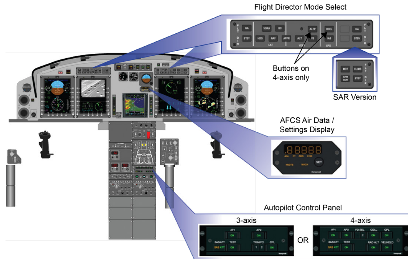
The Bell 412EPI standard flight director modes for the 3-axis AFCS include airspeed hold, altitude hold, VS hold, heading hold, coupled navigation modes, coupled approach modes, and go around.
