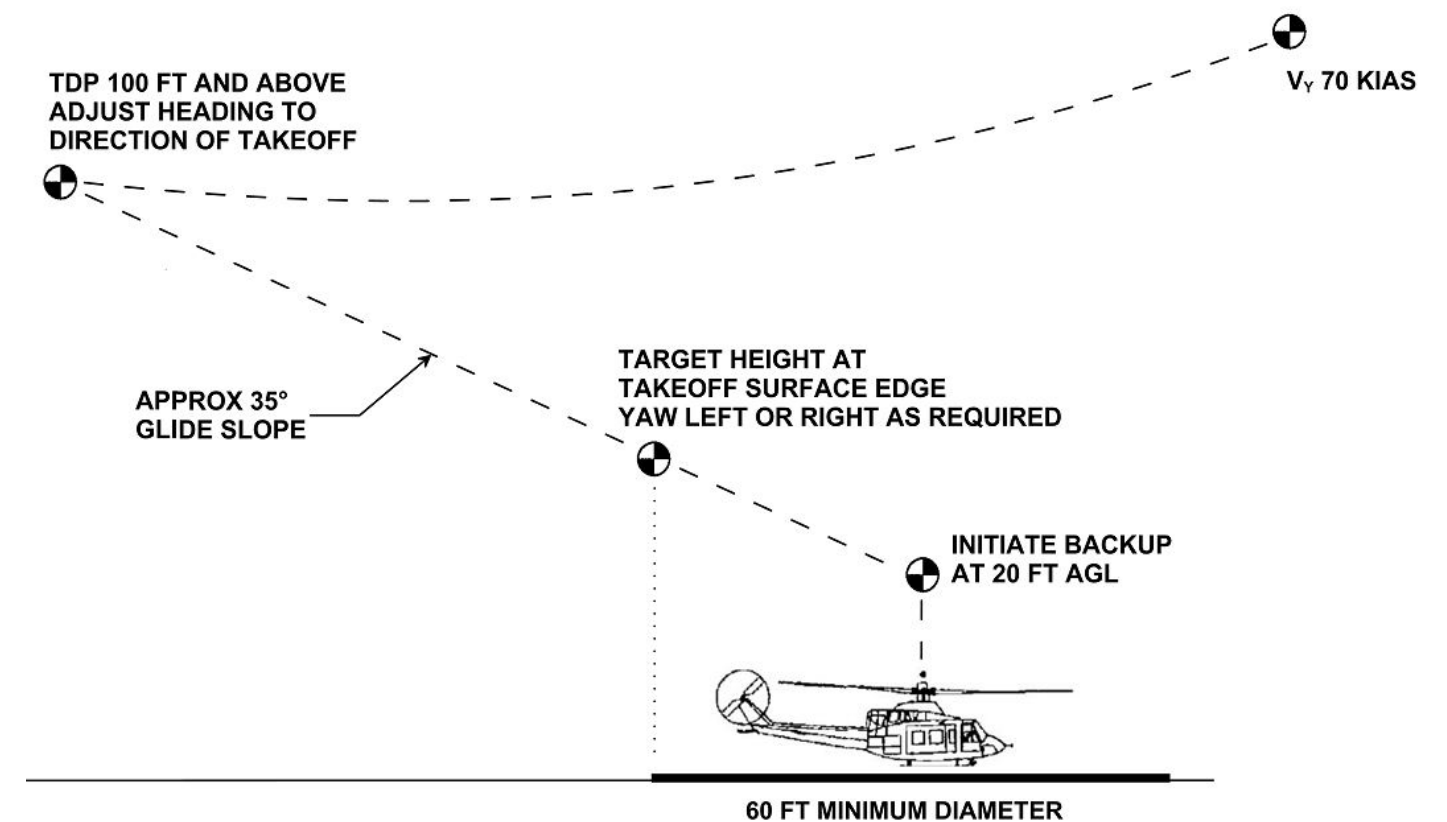
Normal takeoff (AEO) with all engines operating.
