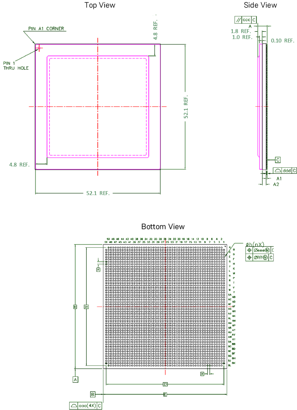
Figure 11: 2597-Pin FBGA Package
