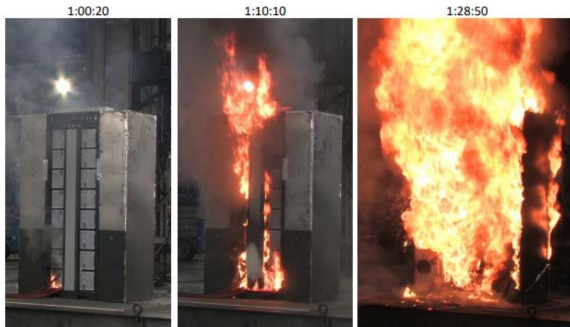
Photos of LNO/LMO fire development during large-scale free burn test: near time of ignition (left), near time of predicted sprinkler operation (middle), peak heat release rate (right).
