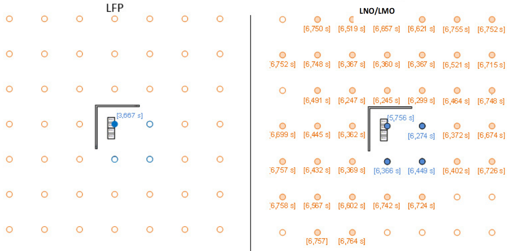
Sprinkler operation overview for LFP (left) and LNO/LMO (right) tests. Sprinklers that operated are shown as solid circles. Blue circles represent active sprinklers that could discharge water and orange circles represent indicator sprinklers that could not.
