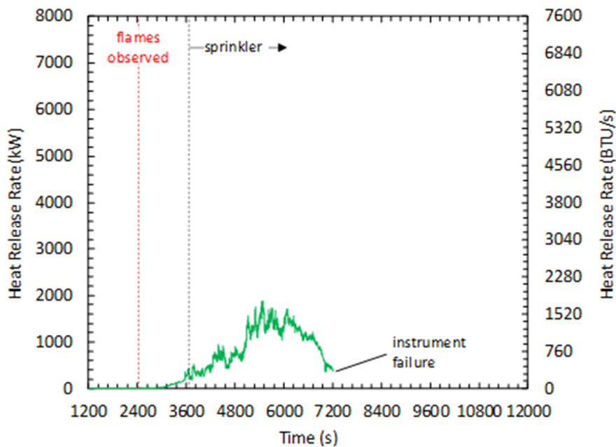
Figure 14. LFP large-scale sprinklered test HRR curve. Courtesy of FM Global.
