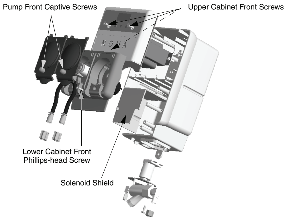
Figure 8-1 Sprite Cabinet Assembly
