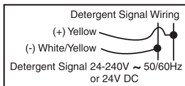
Figure 3-1 Detergent Signal Wiring Diagram—Probe or Probeless Mode
