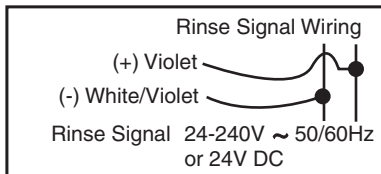
Figure 3-2 Rinse Signal Wiring Diagram
