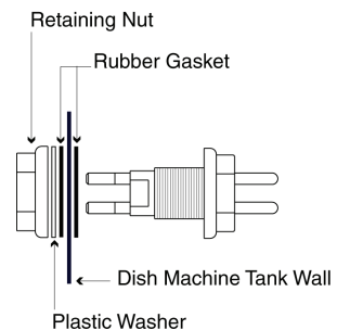
Figure 2-3 Probe Mounting
