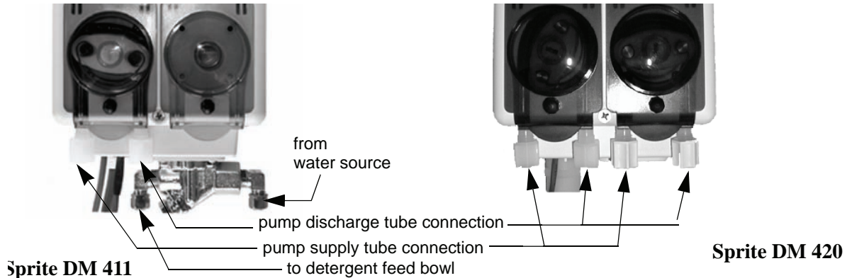
Figure 2-6 Dispensing System
