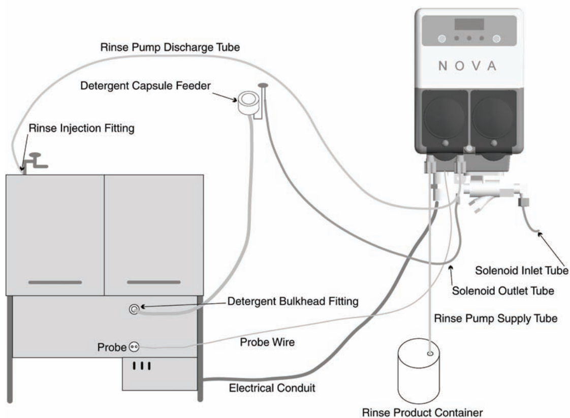
Figure 2-1 System Diagram
