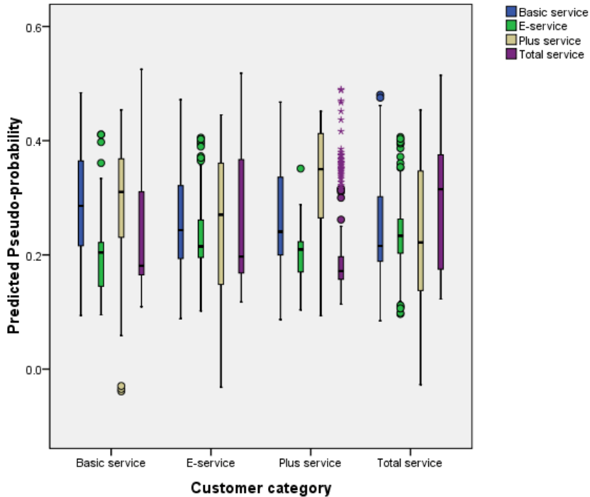
Figure 5-10 Predicted-by-observed chart
