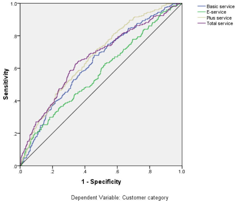
Figure 5-11 ROC curve
