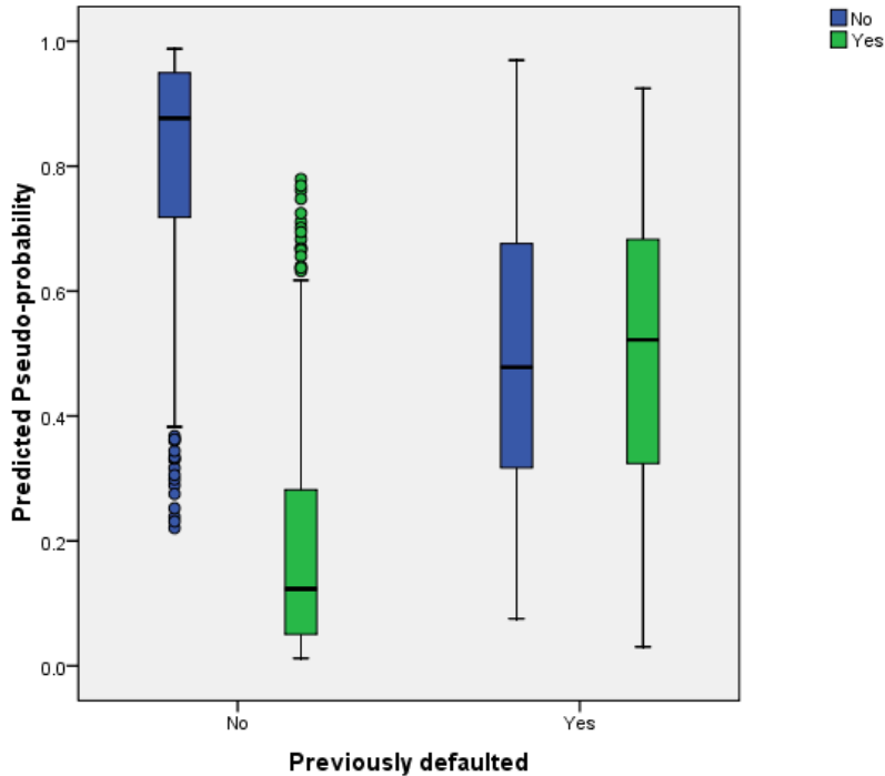
Figure 4-18 Predicted-by-observed chart
