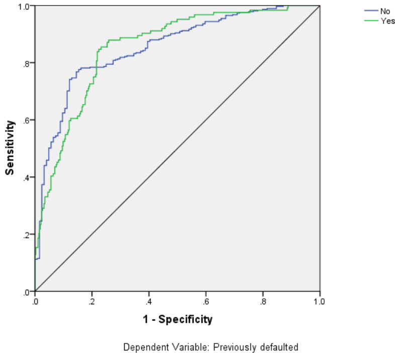
Figure 4-16 ROC curve
