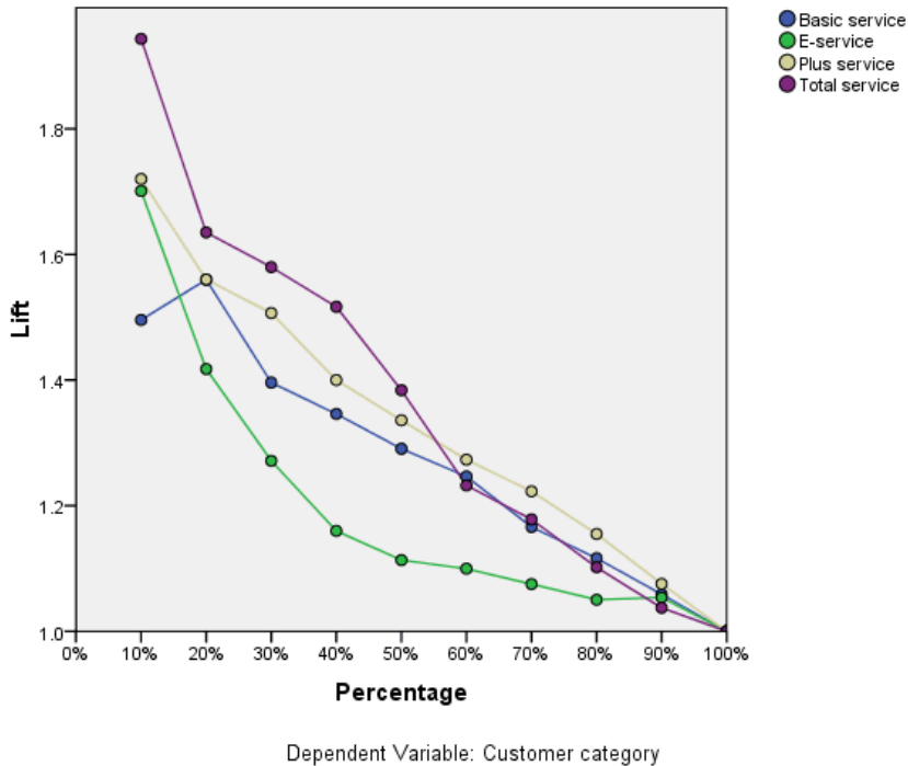
Figure 5-14 Lift chart
