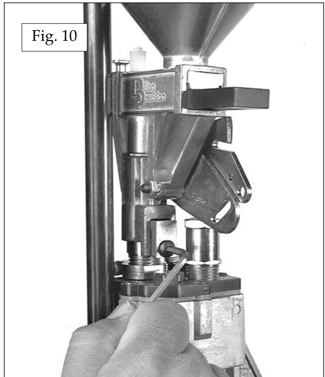
Fig. 10 – The powder measure is held in place by the powder die clamp (#13986). Tighten in place, but do not over tighten.
