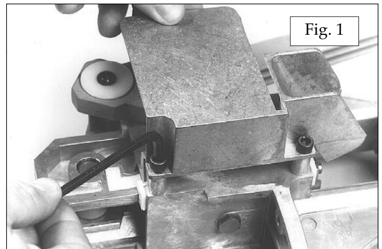
Fig. 1 – Install the ejected cartridge chute bracket (#13659) with two large screws (#13976) from the parts bag.
