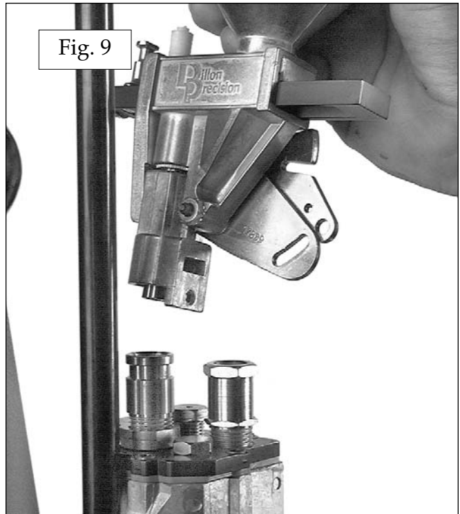
Fig. 9 – With the cap removed and the expander/powder funnel in position, you are now ready to install the powder measure. Place the powder measure on top of the powder die.
