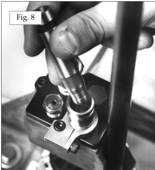
Fig. 8 – Make sure the expander/powder funnel is free to move in the powder die and reinsert it as shown.
