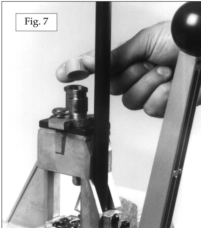
Fig. 7 – Remove the cap from the top of the powder die (#13865). The cap retains the expander/powder funnel during shipping.
