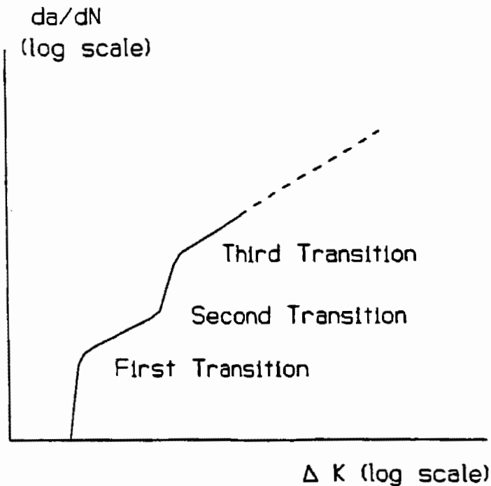
Figure 6-3 Schematic Diagram of Multi-Linear Segments of da/dN for Aluminum.
