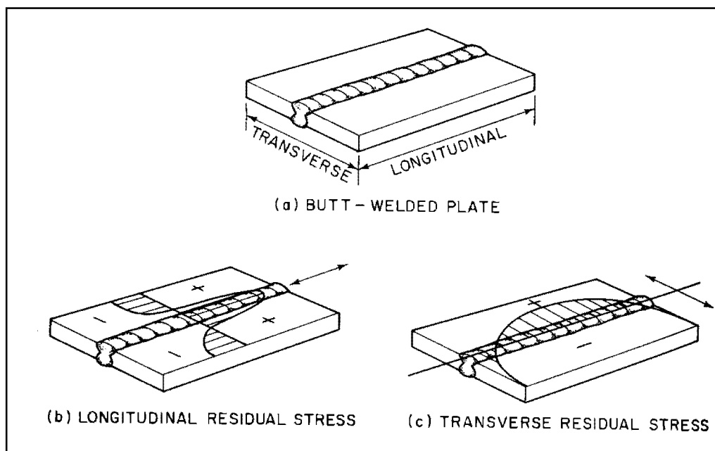
Figure 3-17 Residual Stresses For Butt-Welded Plate
