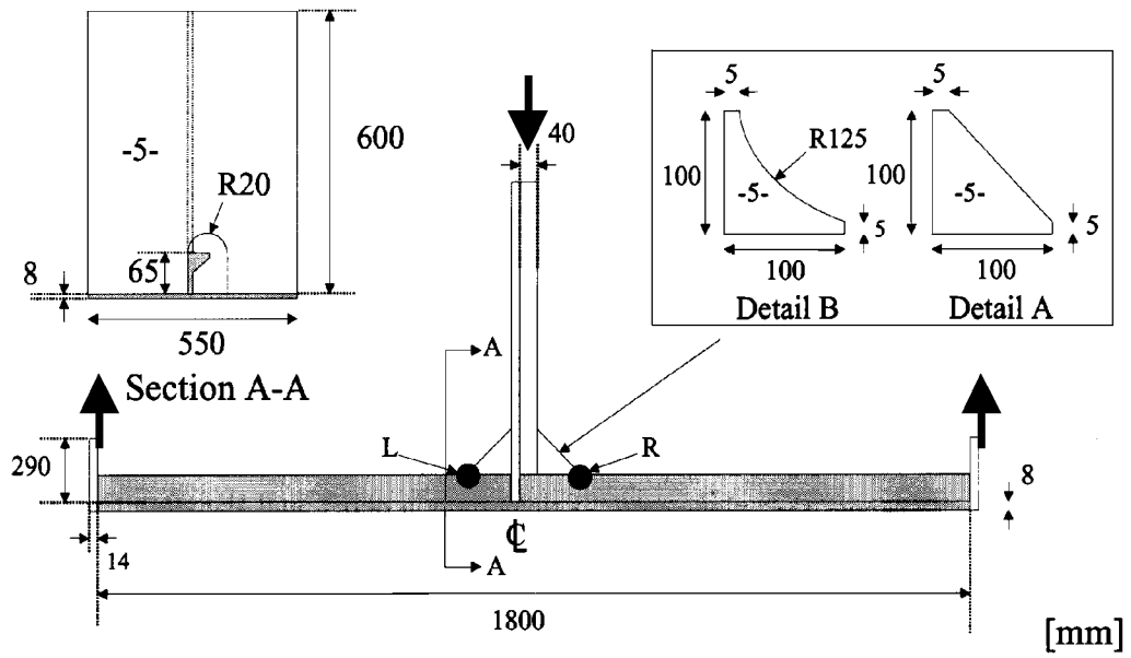
Figure 4-12 Detail 26 – Bulb Stiffener/Deep Frame Connection – Bending In Air.
