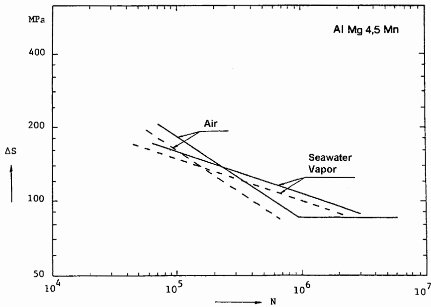
Figure E-10; Transversally welded plate with V-connection; Alloy AlMg4.5Mn; R = 0.1;
