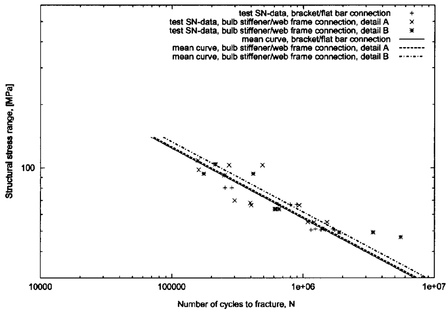
Figure E-18; Flatbar/bracket connection (Joint 25) and the longitudinal stiffener/web frame connection (Joint 26); Structural stress range; Alloy 5083; R = 0.44; Tension;
