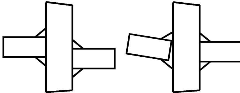
Figure 4-9 Typical Misalignment Problems During Fabrication
