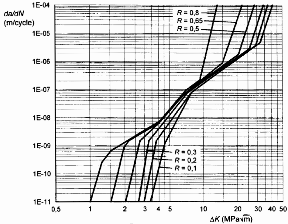
a) R = \text{constant} ( k_{min}/k_{max} ) various R -ratios
