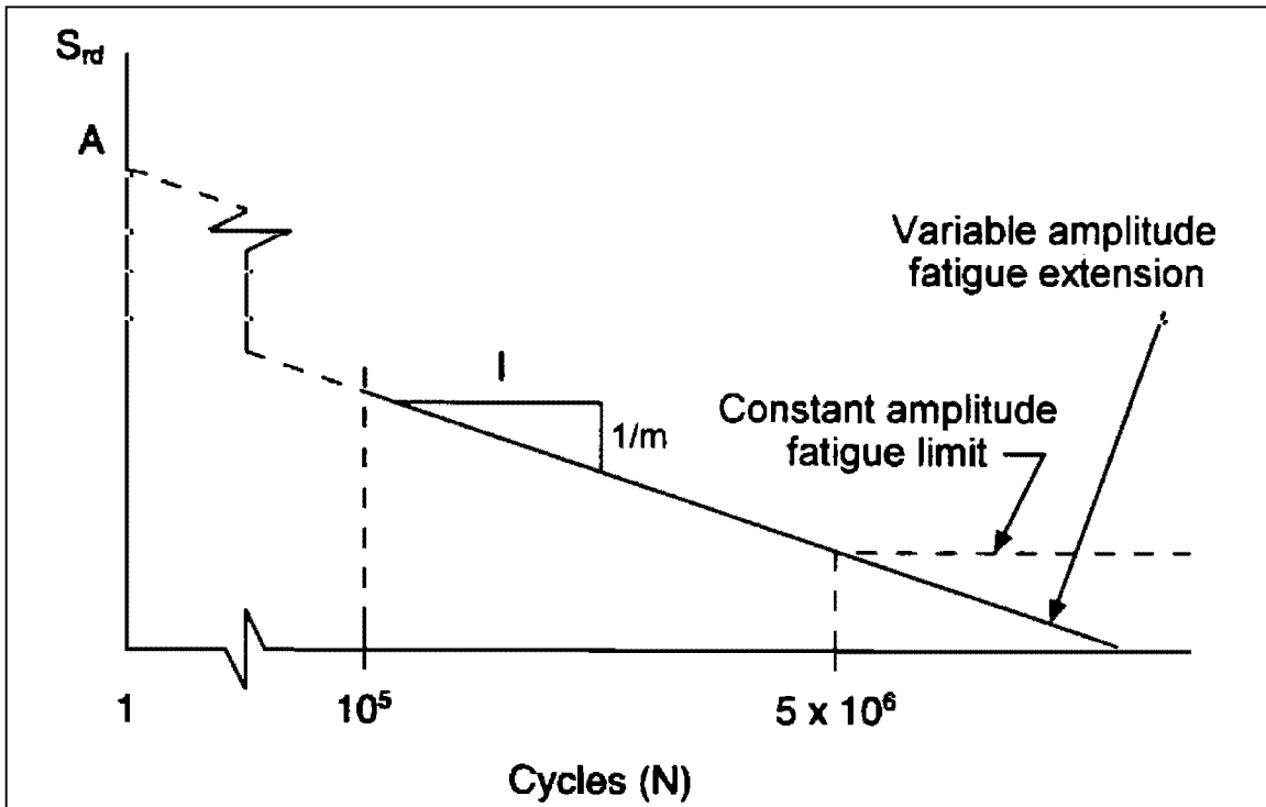
Figure 5-1 Copy of Figure 4.8.1-1 From the Aluminum Design Manual
