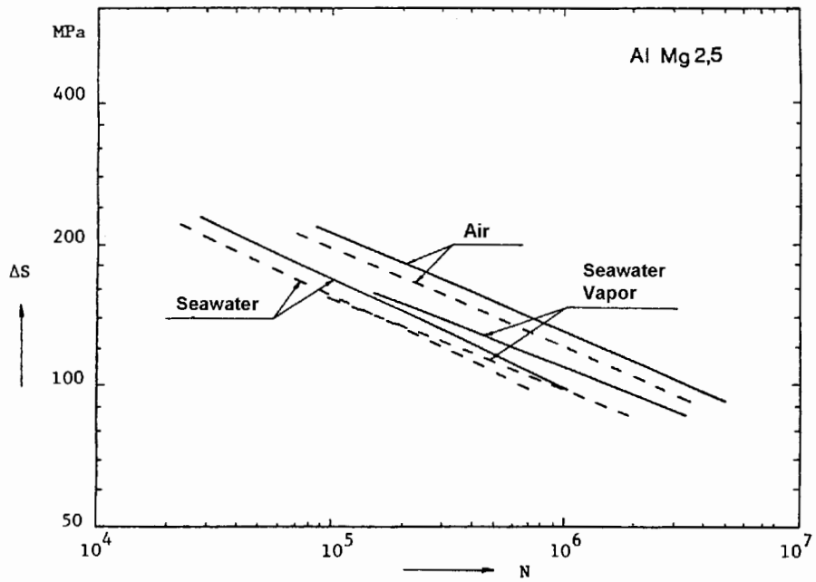
Figure E-4; Transversely welded plate; Alloy AlMg2.5; R-ratio = 0.1;
