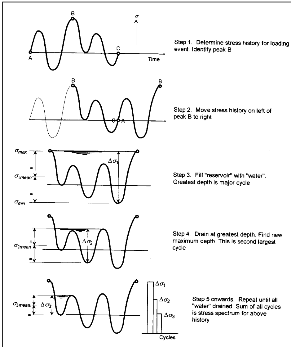
Figure 4-5 Procedure for Conducting The Reservoir Cycle Counting Method
