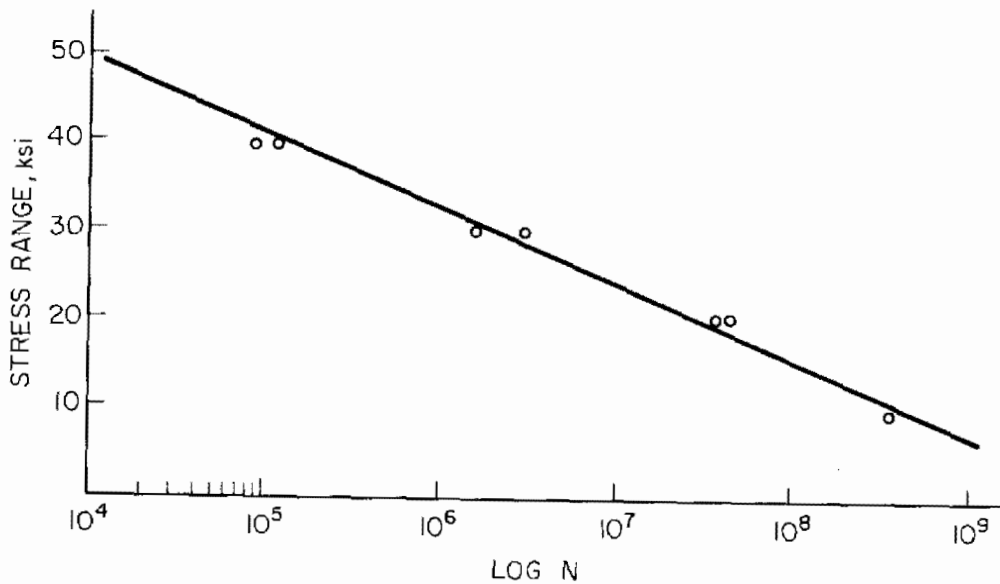
Figure 3-4 Long Life Fatigue for Aluminum
