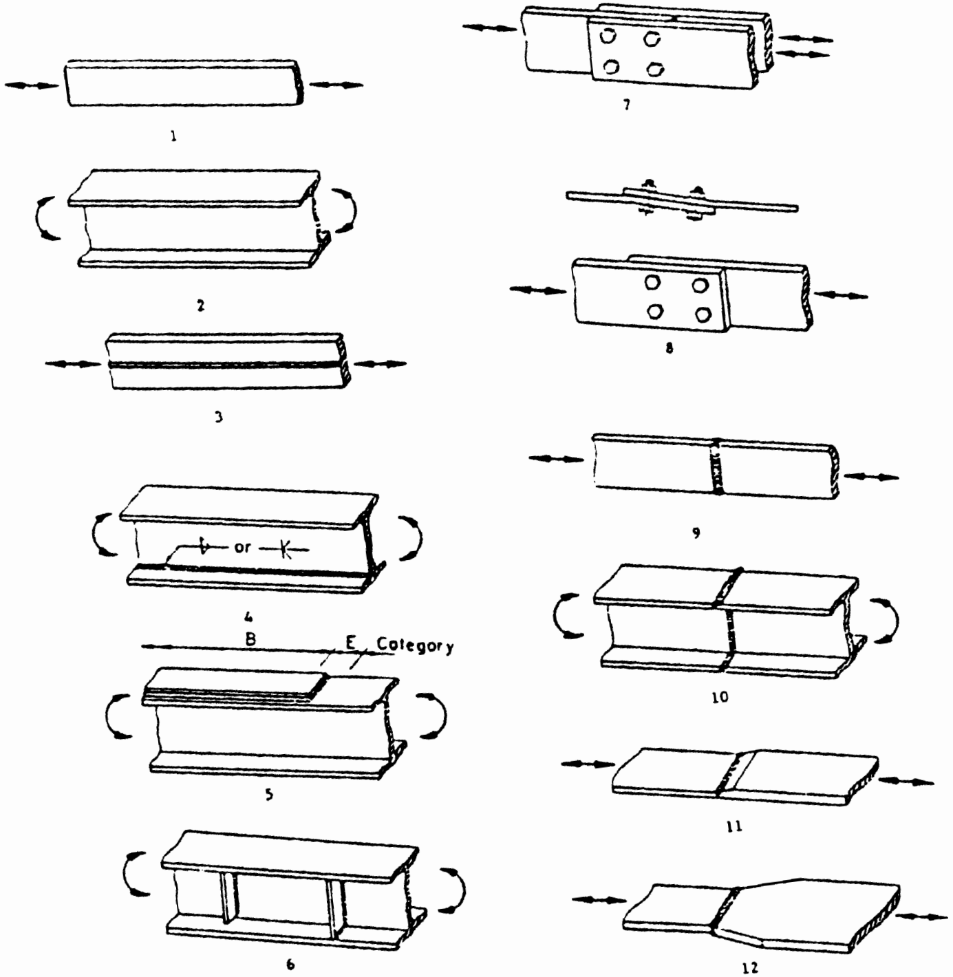
Figure 4.8-1 FATIGUE DESIGN DETAILS
