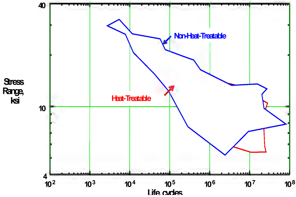
Figure 3-9 Axially Loaded, Transverse Butt-Welded 3/8 inch Aluminum Plate
