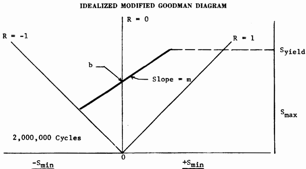
Figure 5-2 Copy of Modified Goodman Diagram from AAR
