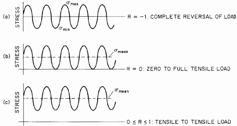
Figure 3-2 Range of Variations in the Stress Ratio, R.
