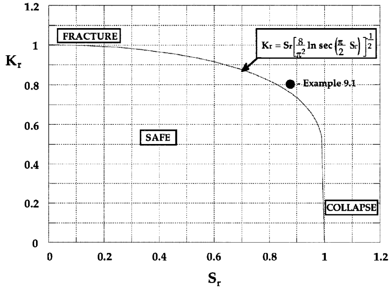
Figure 6-8 Typical Failure Assessment Diagram, FAD
