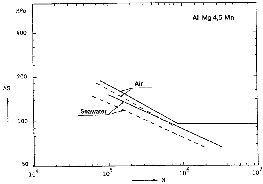
Figure E-5; T-Joint connection; Alloy AlMg4.5Mn; R = 0.1;
