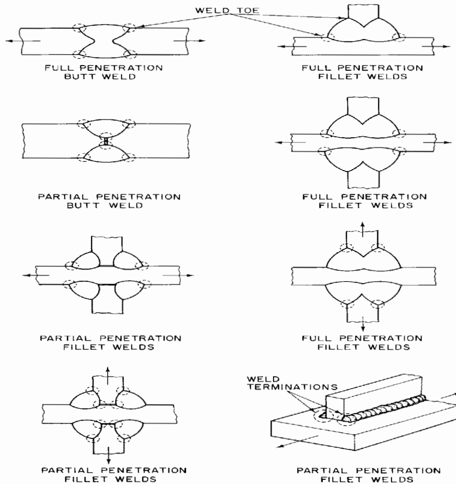
Figure 3-19 Stress Concentration Locations In Typical Welded Joints
