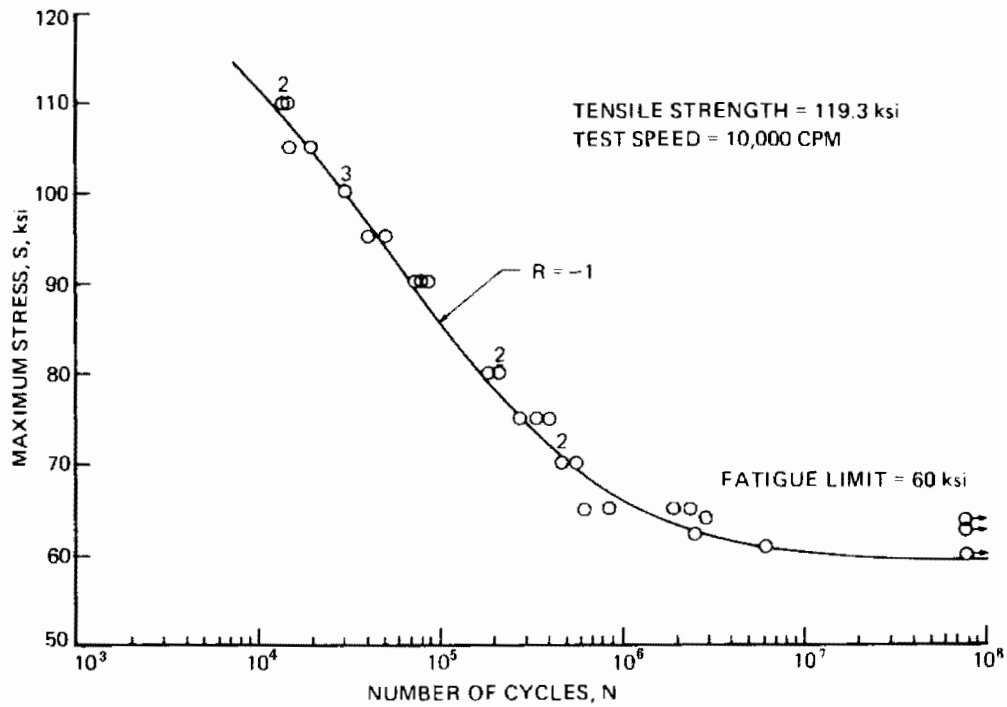
Figure 3-3 Typical S/N Diagram For Steel
