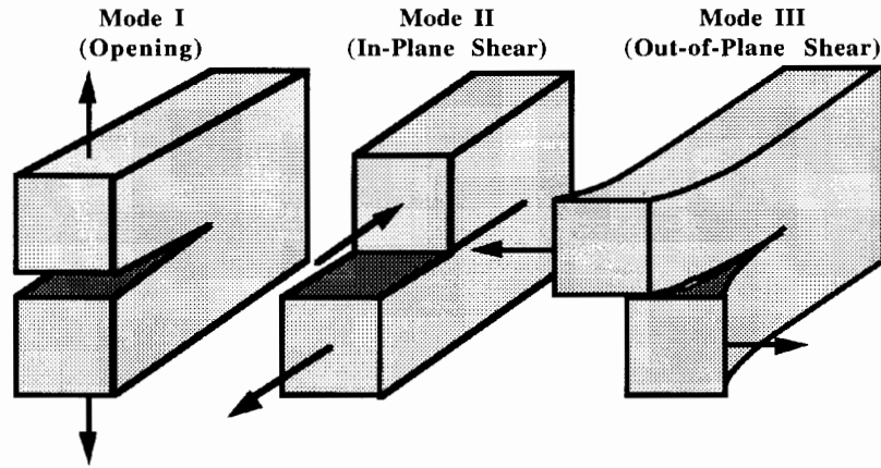
Figure 6-10 Three Modes of Loading for Crack Propagation
