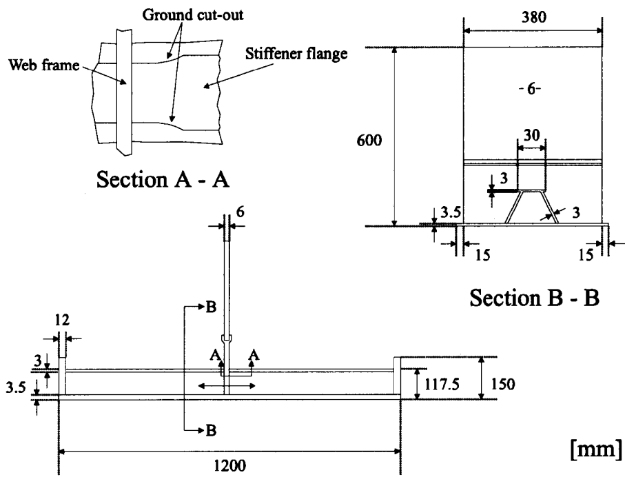
Figure 4-14 Detail 28 Box Stiffener/Deep Frame Connection – Bending In Air.
