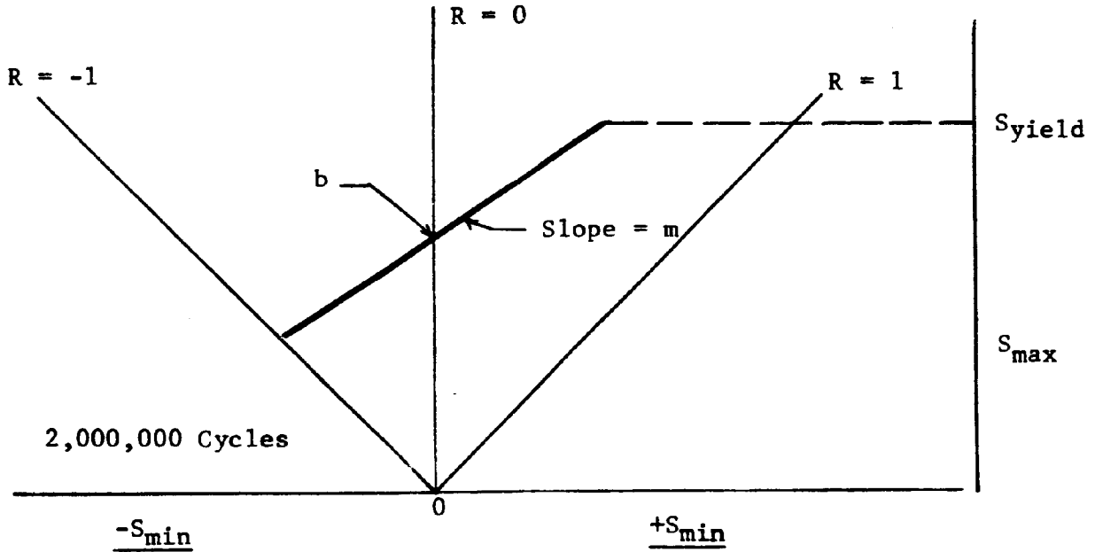
IDEALIZED MODIFIED GOODMAN DIAGRAM
