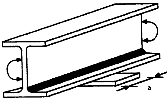
3.2.9 & 10(A) — LATERAL PLATE ATTACHMENT TO FLANGE OF EXTRUDED OR FABRICATED BEAM (FLEXURAL LOADING) 3.2.9(A): a < 2" 3.2.10(A): a \leq 4"
