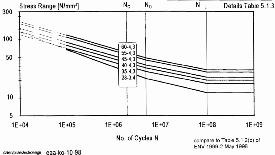
Fig. 5.2.3* Design Curves \Delta\sigma -N for members with welded attachments / longitudinal welds
