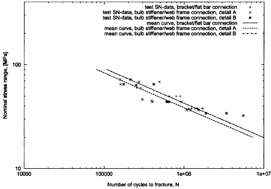
Figure E-17 Flatbar/bracket (Joint 25) connection and bulb stiffener/web frame connection (Joint 26); Nominal stress range; Alloy 5083; R = 0.44; Tension;
