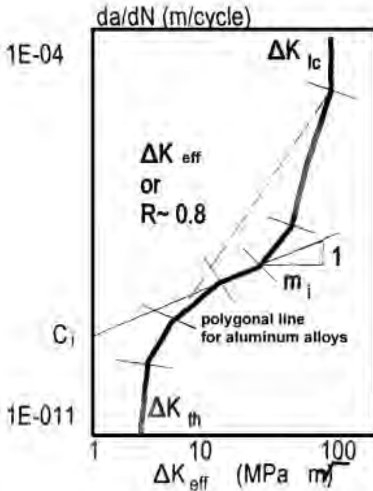
Figure 6-4 Polygonal da/dN curve for aluminum
