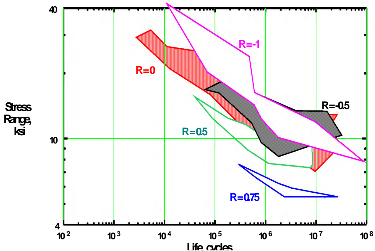
Figure 3-6 Effect of Stress Ratio on Fatigue Life of Aluminum
