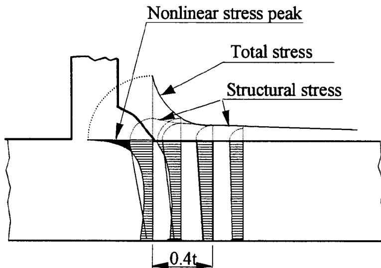
Figure 4-8 Local Stress Concentrations in Fillet Weld
