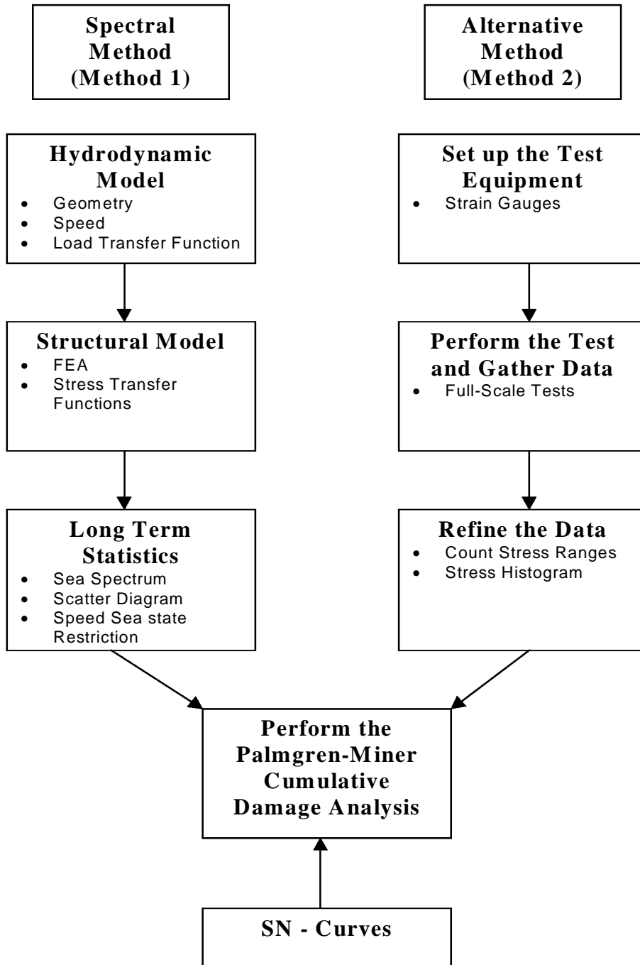
Figure 2-1 Flow Chart For Load Prediction
