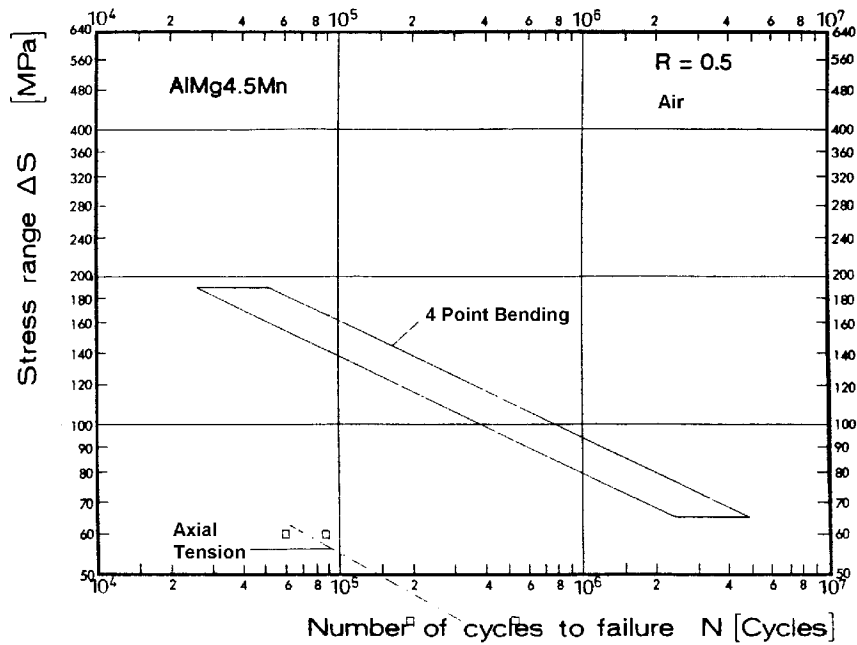
Figure E-14; T-Joint connection; Alloy AlMg4.5Mn; R = 0.5;
