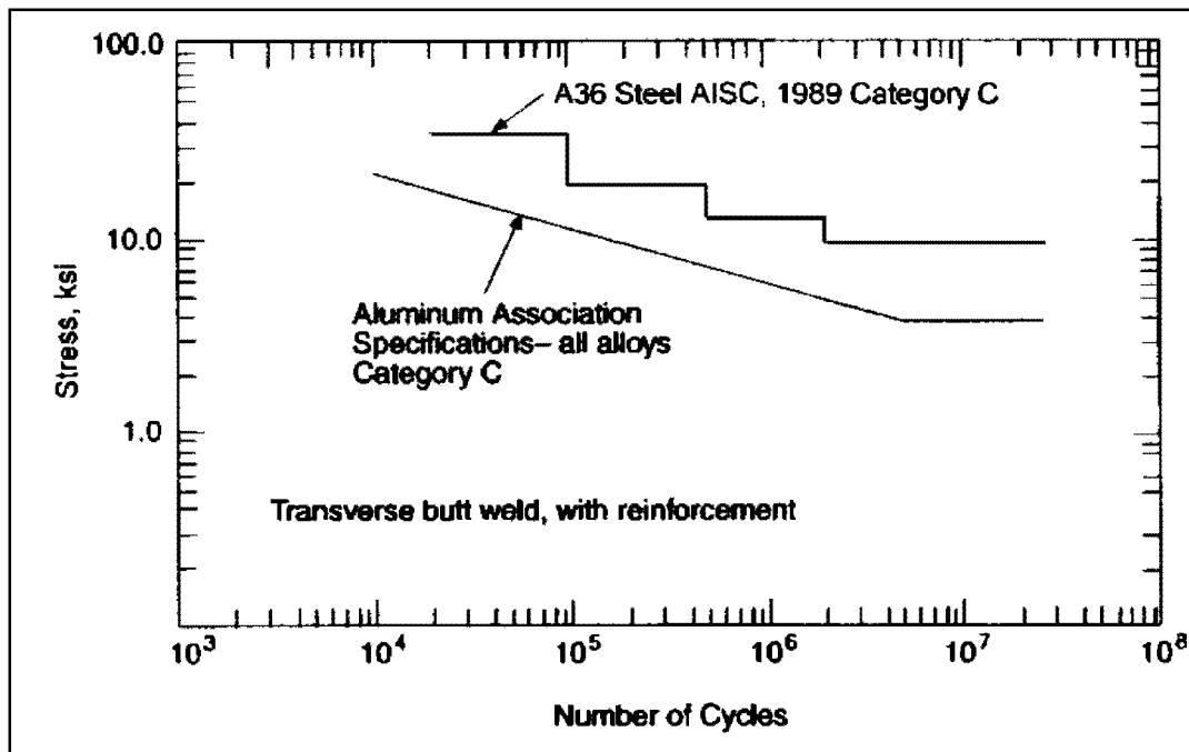
Figure 4.0-1 FATIGUE DESIGN CURVES FOR ALUMINUM AND STEEL
