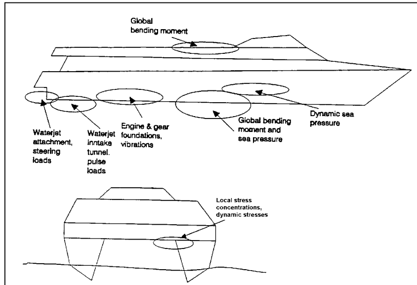
Figure 2-2 Critical areas for fatigue consideration of high-speed catamarans.
