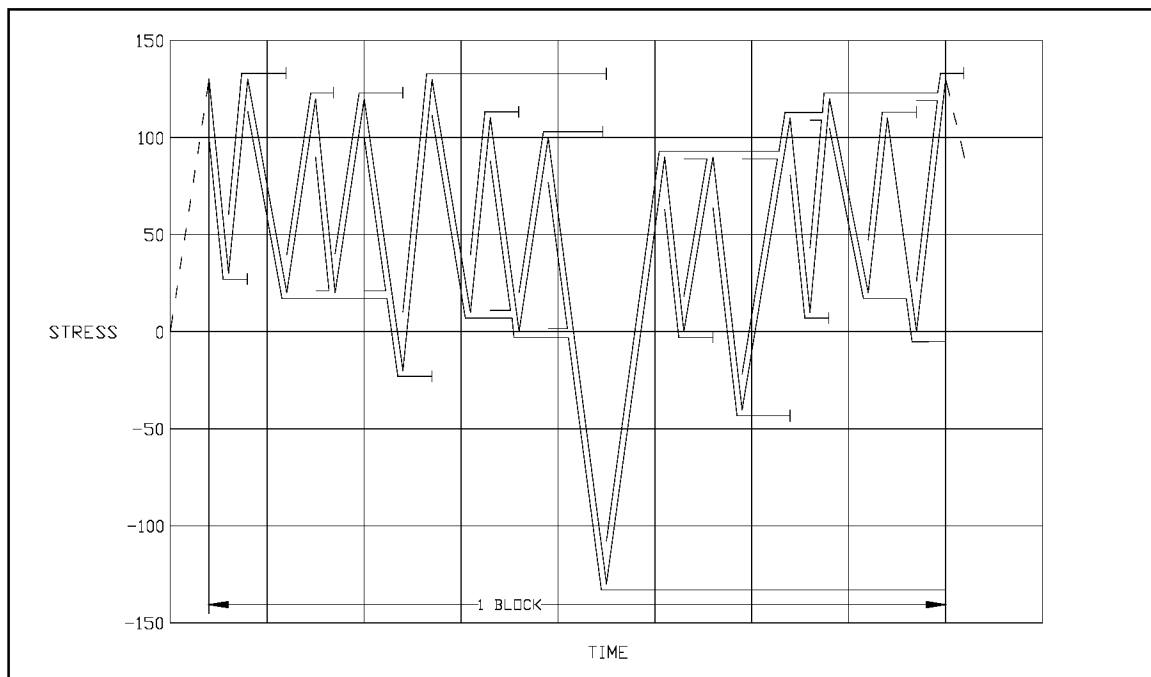
Figure 4-4 Rainflow Cycle Counting
