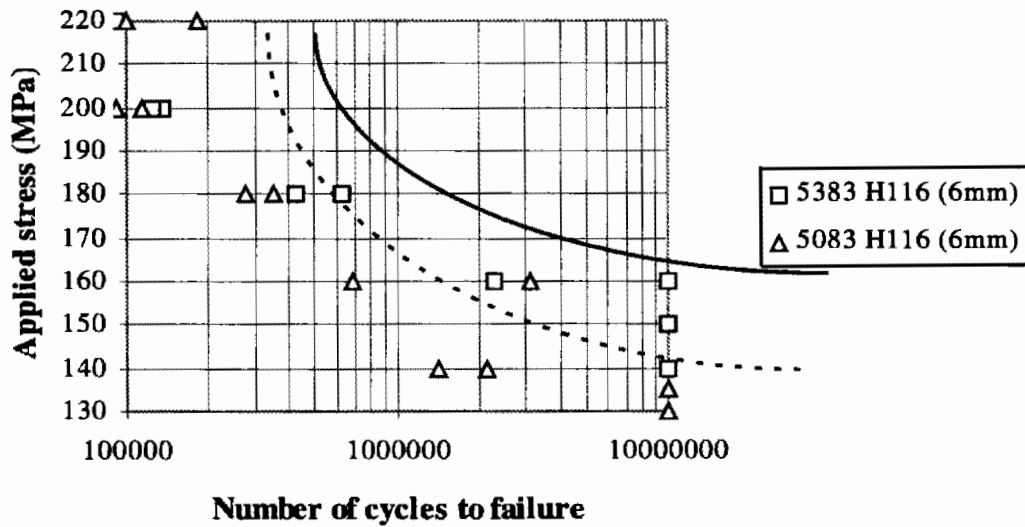
Figure 3-21 Fatigue Tests on 5083 and 5383 conducted at laboratory
