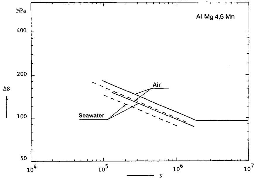
Figure E-13; Cruciform Joint; Alloy AlMg4.5Mn; R = 0.1;
