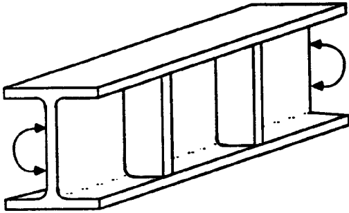
3.1.7(A) — STIFFENERS ON EXTRUDED OR FABRICATED BEAM (FLEXURAL LOADING)
