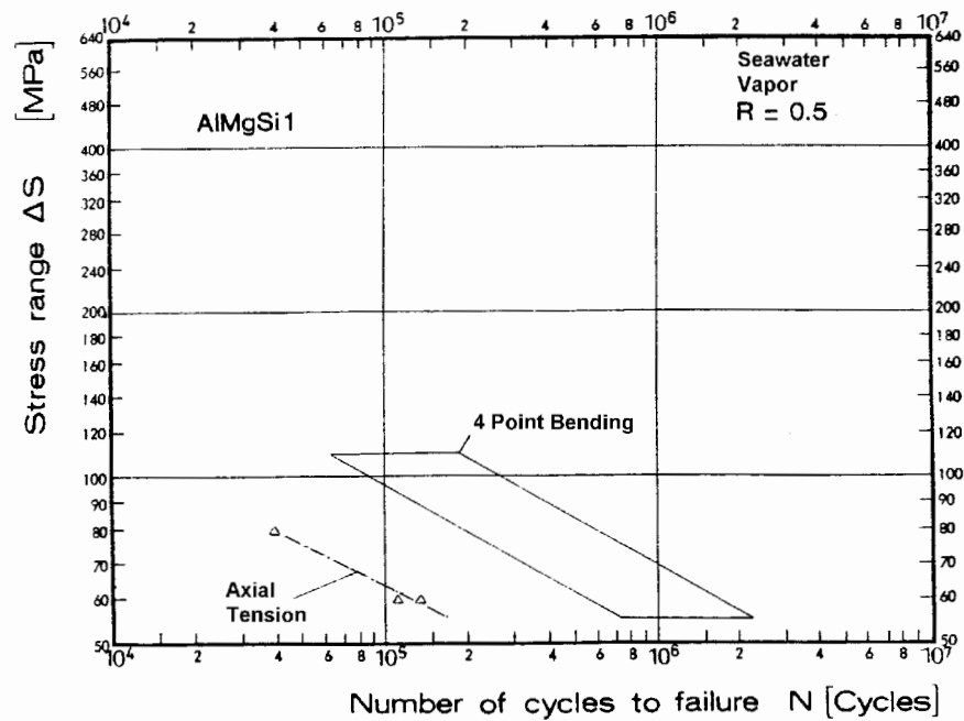
Figure E-16; T-Joint; Alloy AlMgSi1; R = 0.5 ;
