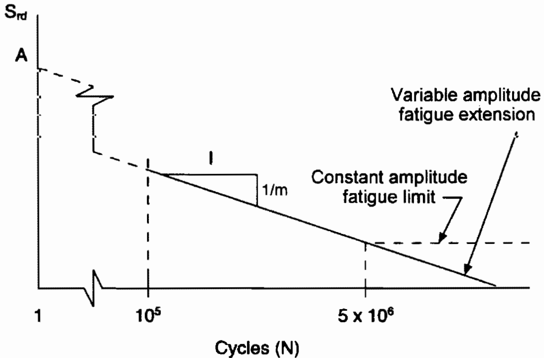
Figure 4.8.1-1 SCHEMATIC FATIGUE CURVE
