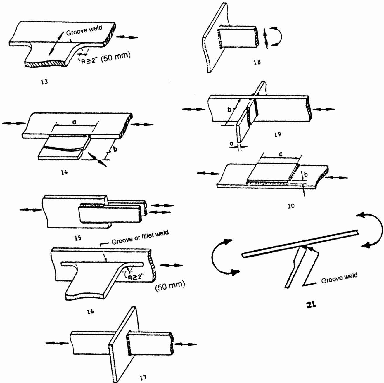
Figure 4.8-1 FATIGUE DESIGN DETAILS (Continued)
