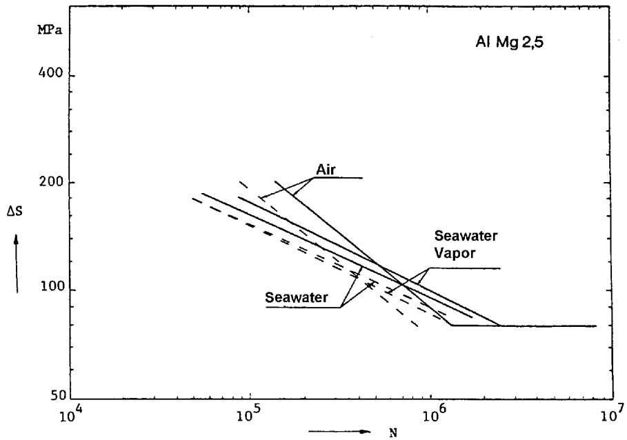
Figure E-6; T-Joint connection; Alloy AlMg2.5; R = 0.1; g);
