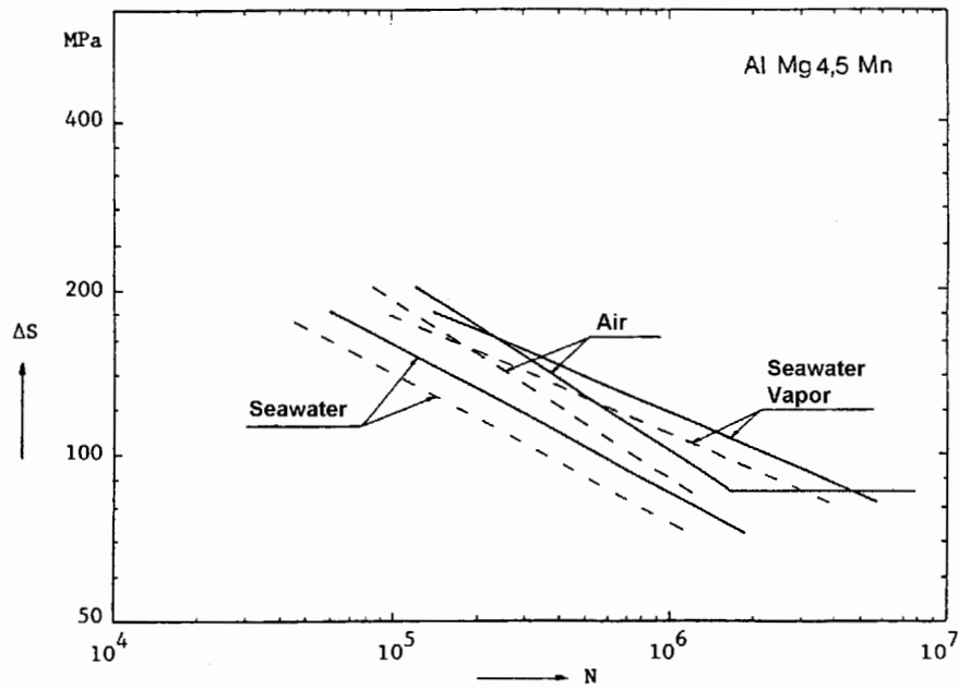
Figure E-3; Transversely welded plate; Alloy AlMg4.5Mn; R = 0.1; Error! Reference source not found.
