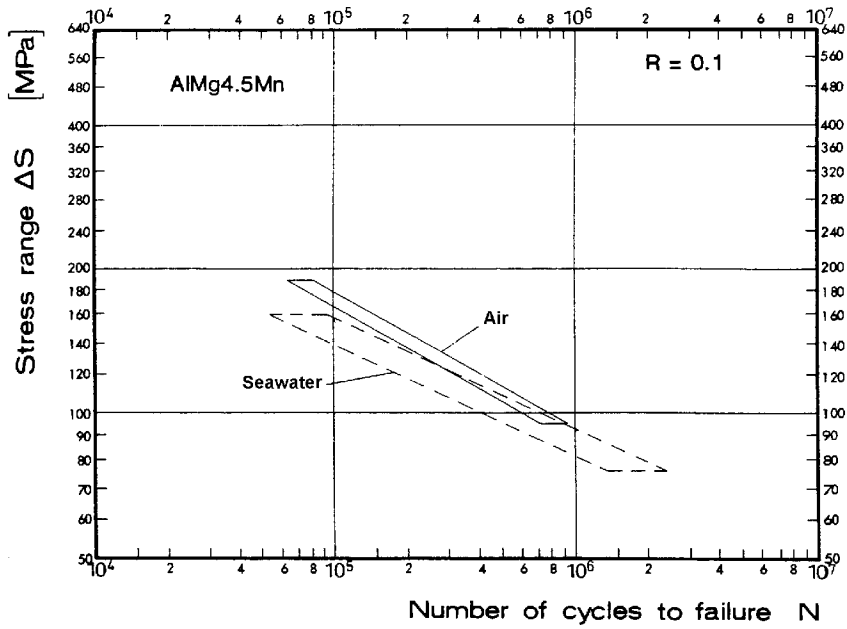
Figure E-8; T-Joint connection; Alloy 5083; R = 0.1 ;
