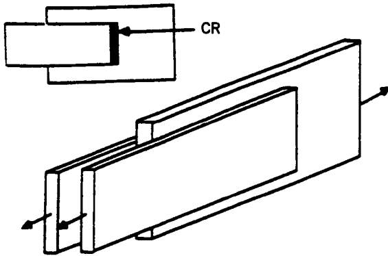
4.2.2(A) — LAP WELDED JOINT — WITH TRANSVERSE WELD ONLY (AXIAL LOAD)
