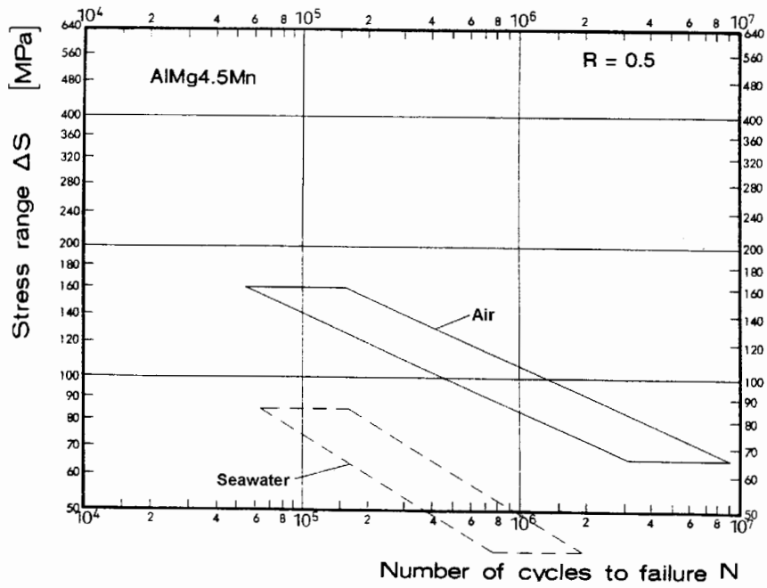
Figure E-11; T-Joint connection; Alloy AlMg4.5Mn; R = 0.5 ;
