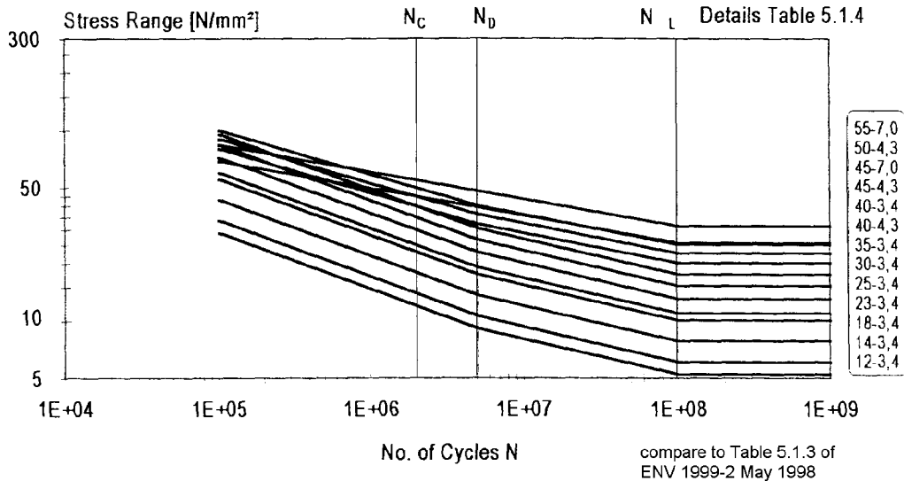
Fig. 5.2.4* Design Curves \Delta\sigma -N for welded joints between members
