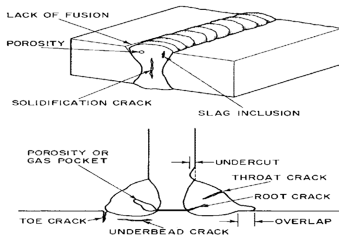
Figure 3-18 Potential Weld Flaws as a Result of Improper Welding
