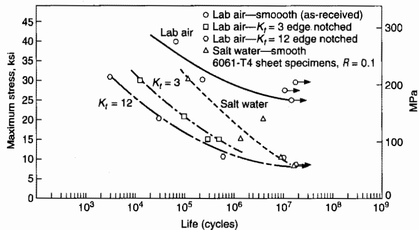
Figure 3-5 Effect of Seawater on Aluminum Fatigue Tests
