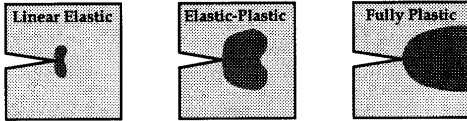
Figure 6-1 Relative Size of Plastic Zone at Crack Tip
