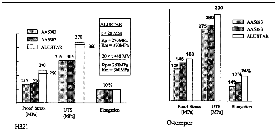
Figure 3-23 Comparison of Material Strength for 5083, 5383 and 5059
