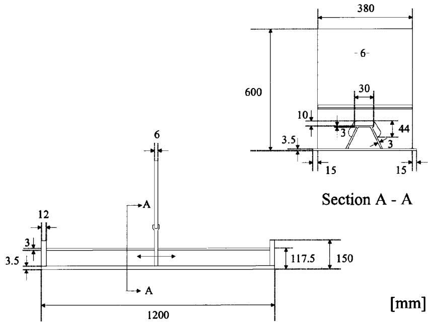
Figure 4-13 Detail 27 – Box Stiffener/Deep Frame Connection – Bending In Air.
