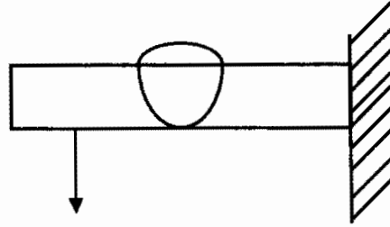
Figure 3-20 Small Specimen for 5383 Fatigue Tests
