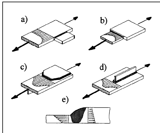
Figure 4-6 Geometric Stress Concentration Profiles
