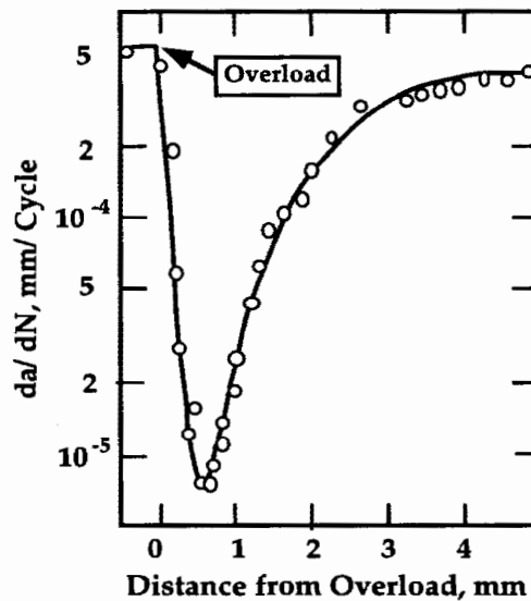
Figure 6-6 Crack Retardation as a Result of Peak Overload
