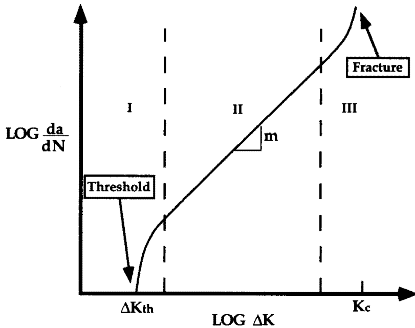
Figure 6-2 Typical FCGR Curve
