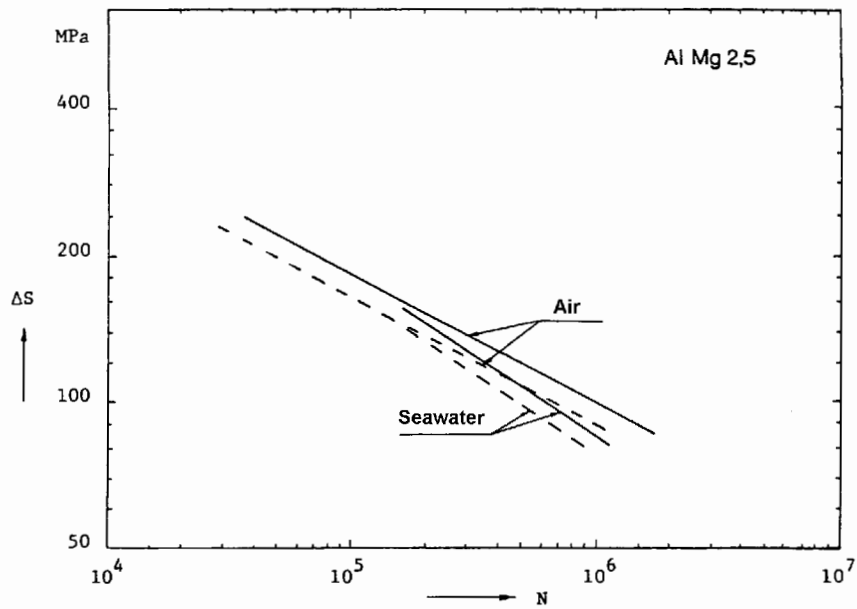
Figure E-9; Transversely welded plate with V- connection; Alloy AlMg2.5; R = 0.1;
