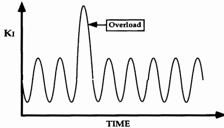
Figure 6-5 Peak Overload in Constant Amplitude Field
