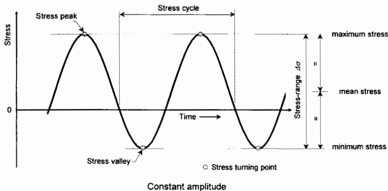
Figure 4-3 Constant Amplitude Curve
