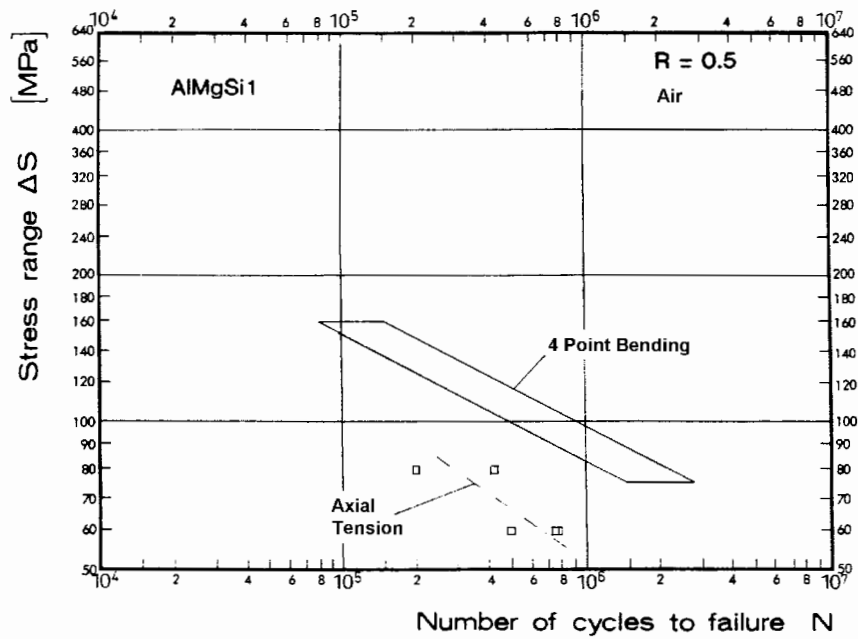
Figure E-15; T-Joint; Alloy AlMgSi1; R = 0.5 ;
