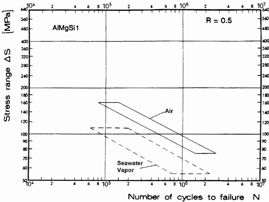
Figure E-12; T-Joint connection; Alloy AlMgSi1; R = 0.5 ;
