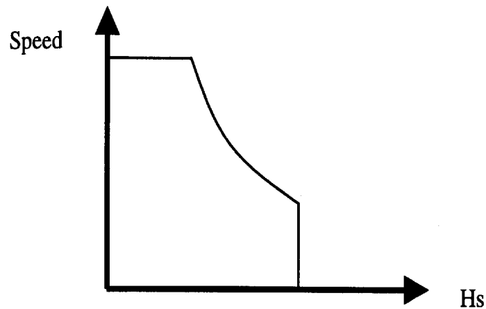
Figure 2-3 Speed/Wave Height Restriction Curve for High-Speed Craft
