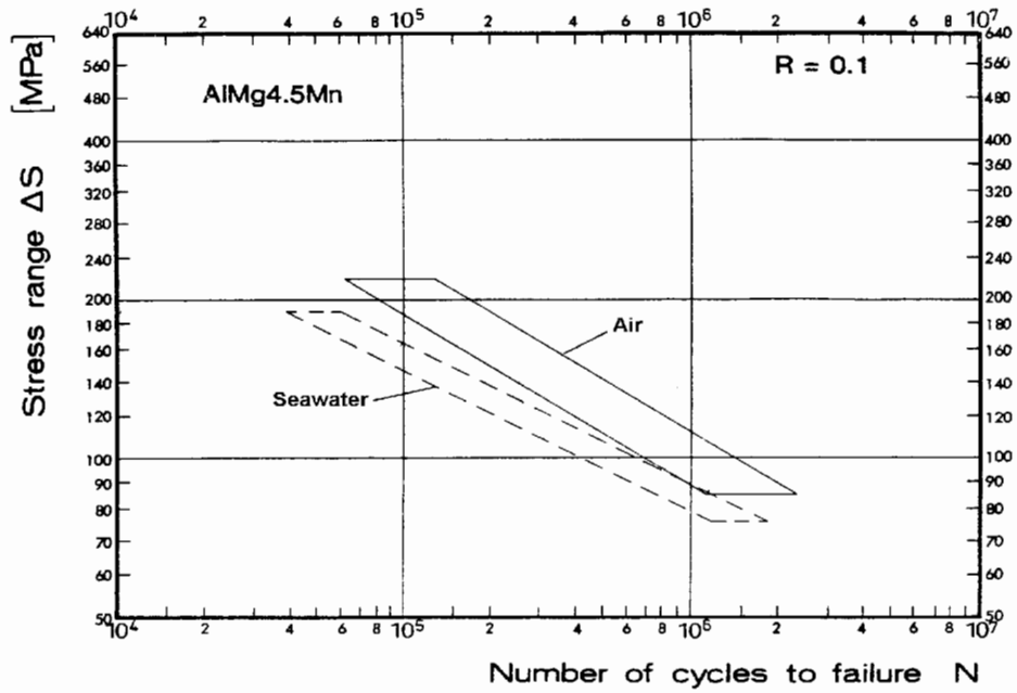
Figure E-1; Transversely welded plate; Alloy AlMg4.5Mn; R = 0.1;
