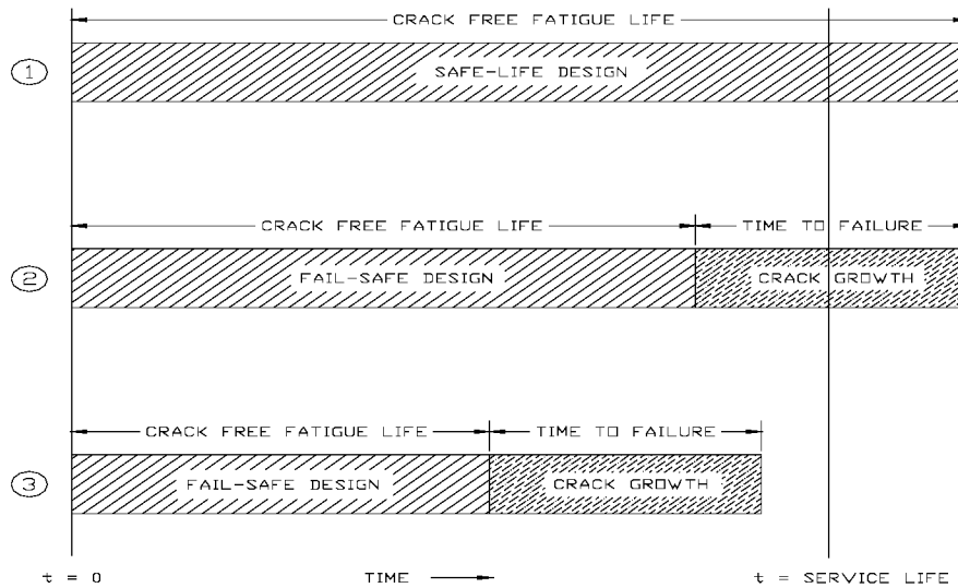
Figure 3-16 Schematic Representation of Fatigue Life to Service Life
