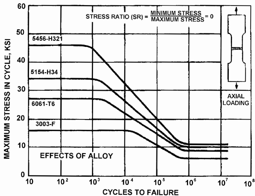
Figure 3-10 The Effect of Alloy on the Fatigue Life of Aluminum
