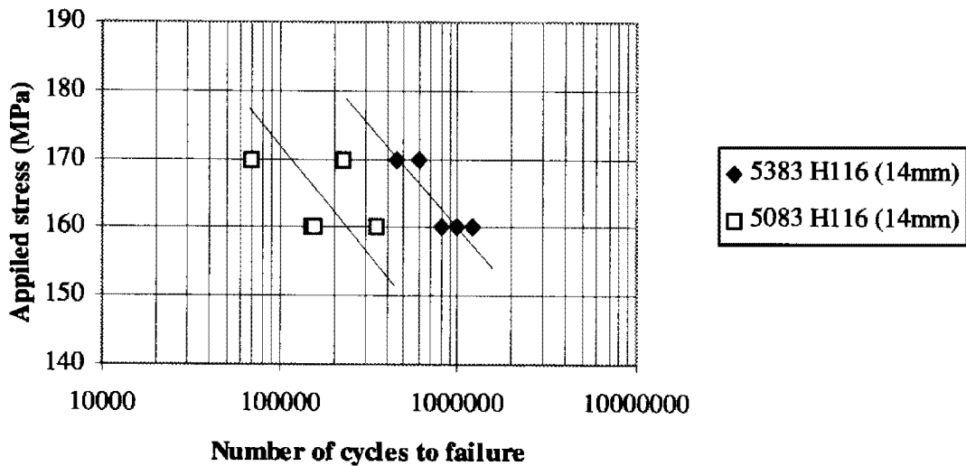
Figure 3-22 Fatigue Tests on 5083 and 5383 details built at shipyard
