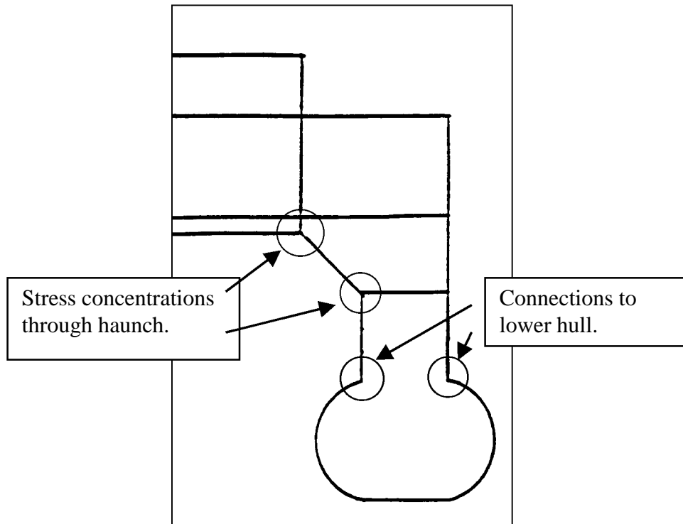
Figure 4-2 Typical Problem Areas On A SWATH
