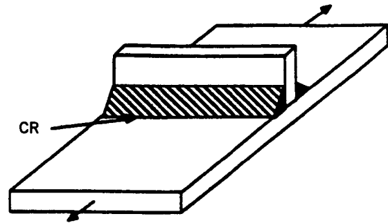
5.2.1.1(A) — PLATE WITH TRANSVERSE FILLET WELDED RIB — ONE SIDE (AXIAL LOAD)
