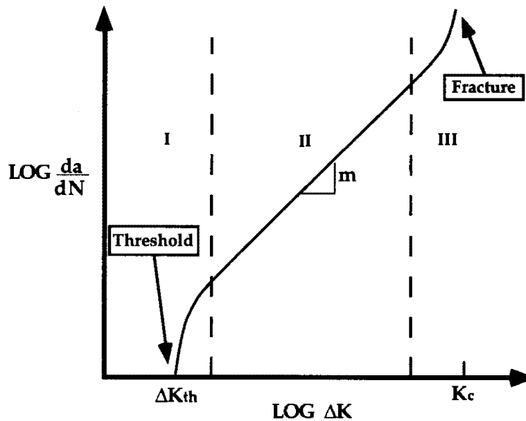
Figure 3-14 Typical Fatigue Crack Growth Rate, FCGR Curve
