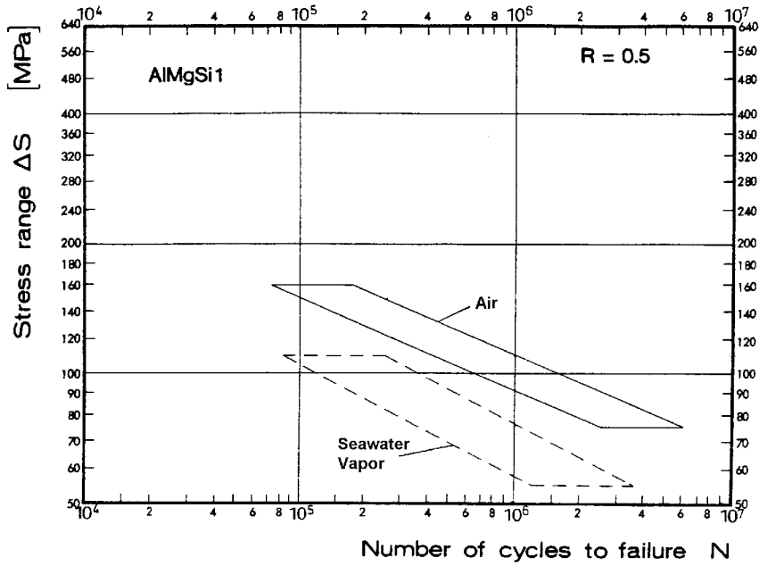
Figure E-7 Transversely welded plate; Alloy AlMgSi1; R = 0.5 ;
