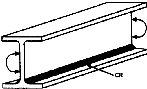
3.2.1(A) — FABRICATED BEAM (FLEXURAL LOADING)
