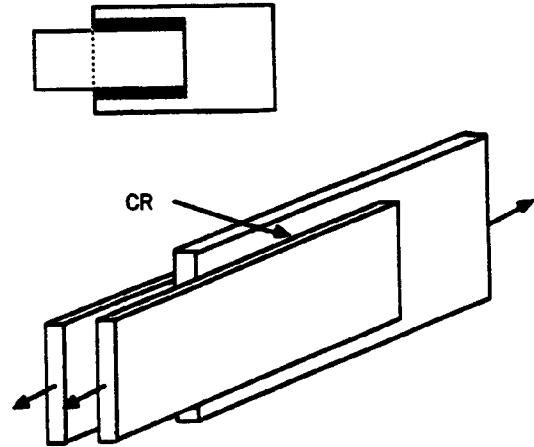
4.1.1(A) — LAP WELDED JOINT — WELD STRESS CRITICAL (AXIAL LOAD)
