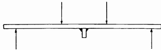
Detail 23 T – intersection fillet welded.
