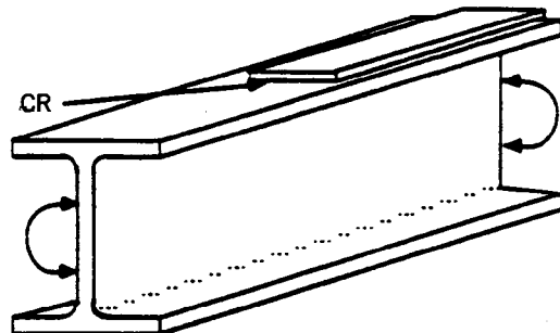
3.1.5(A) — PARTIAL LENGTH COVER PLATES ON EXTRUDED OR FABRICATED BEAM (FLEXURAL LOADING)
