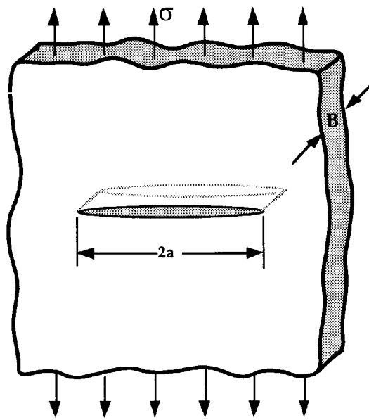
Figure 6-7 Crack Length and Thickness in Typical Specimen
