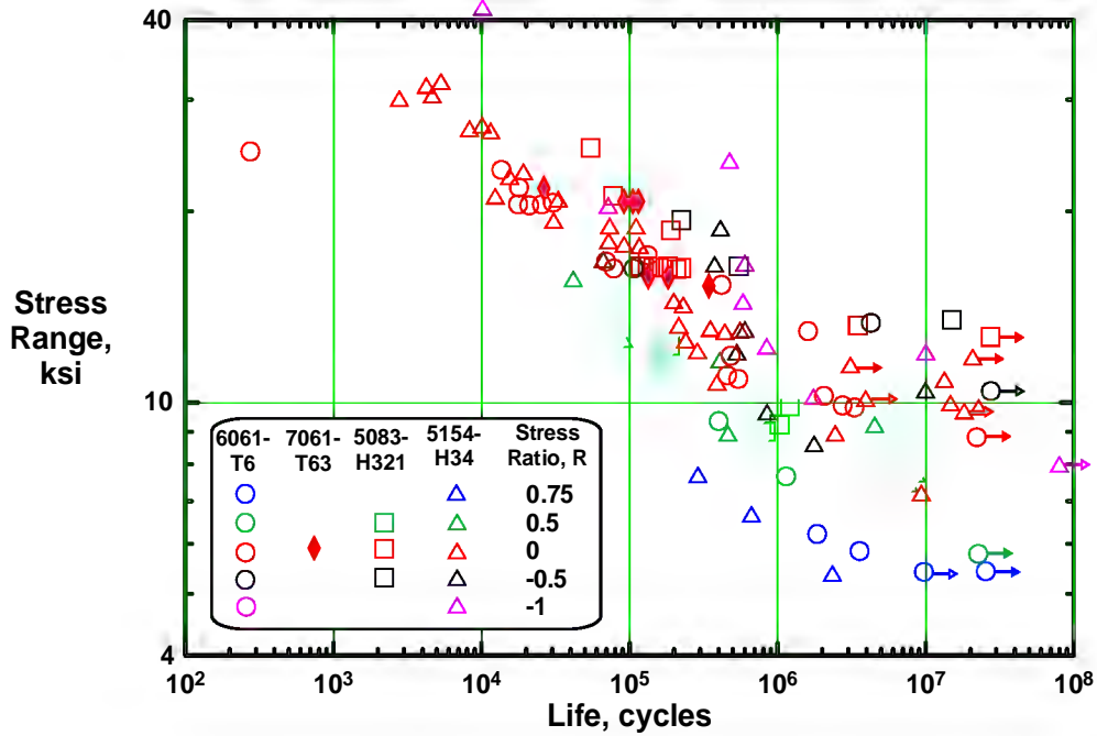
Figure 3-8 Axially Loaded, Transverse Butt-Welded 3/8 inch Aluminum Plate
