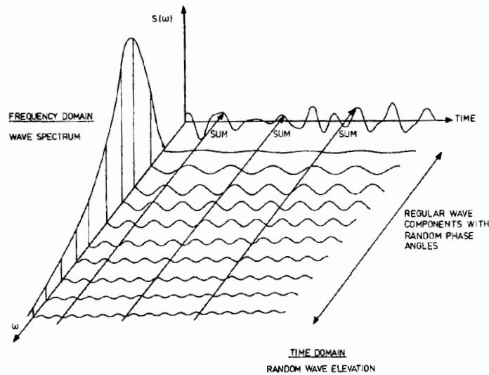
Figure 2-4. A schematic description of a sea spectrum.
