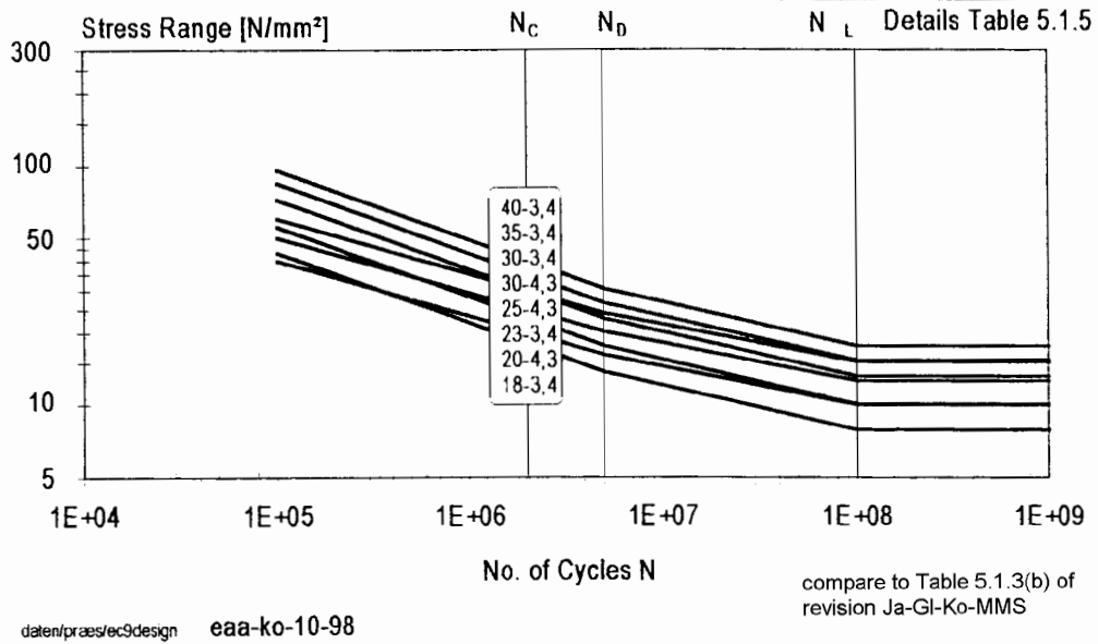
Fig. 5.2.5* Design Curves \Delta\sigma -N for crossing welds and built-up beams
