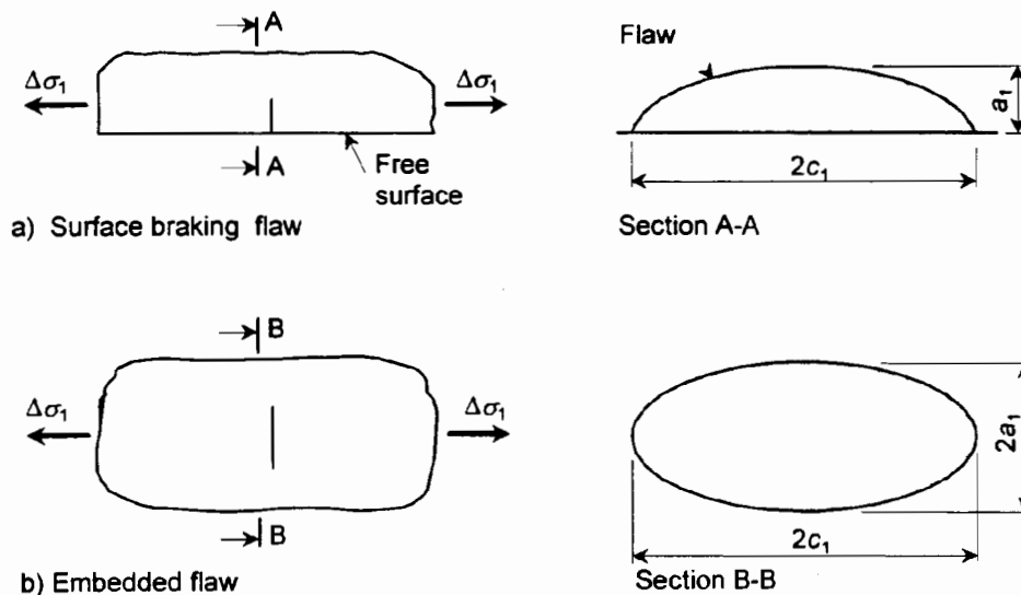
Figure B.2.1 Pre-existing planar flaws
