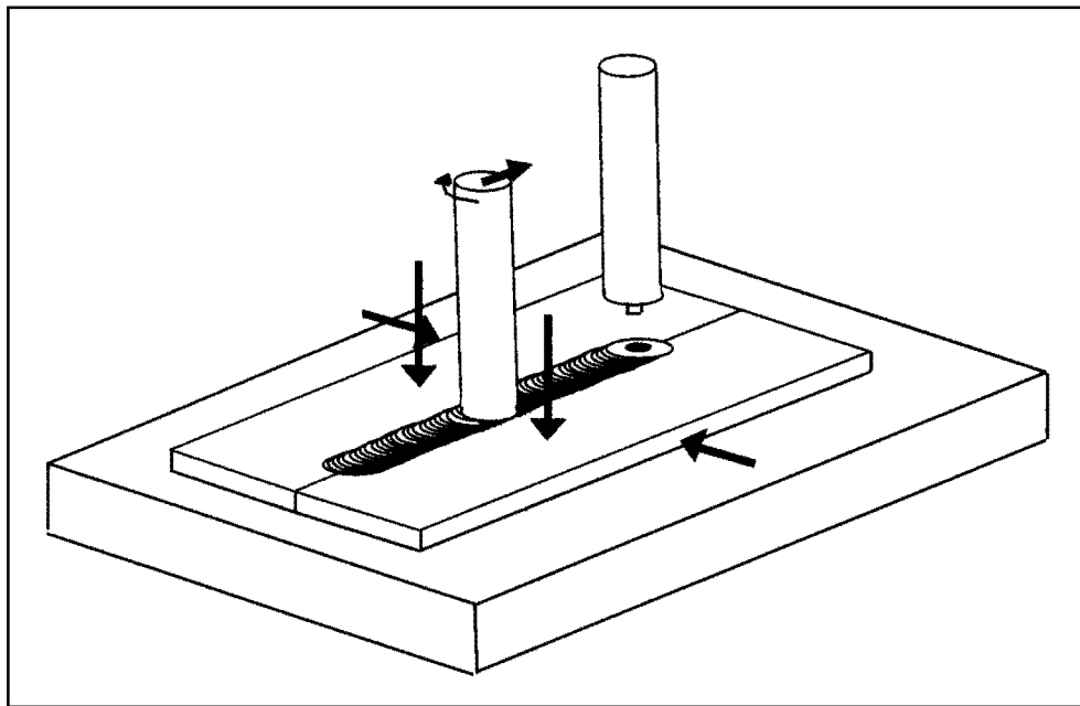
Figure 3-25 Schematic of Friction Stir Welding Operation
