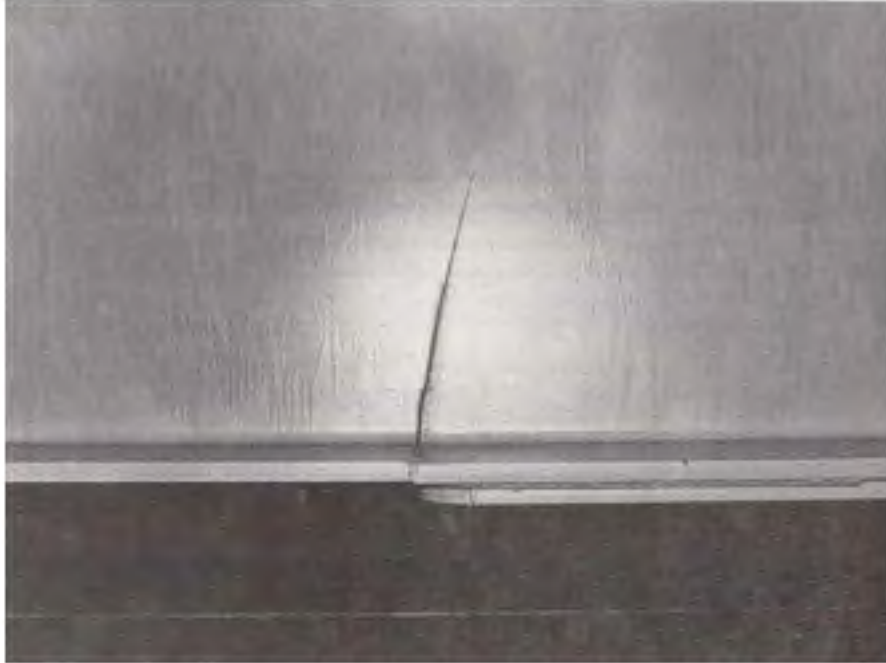
Figure 3-12 Fatigue Crack at Cover Plate Detail
