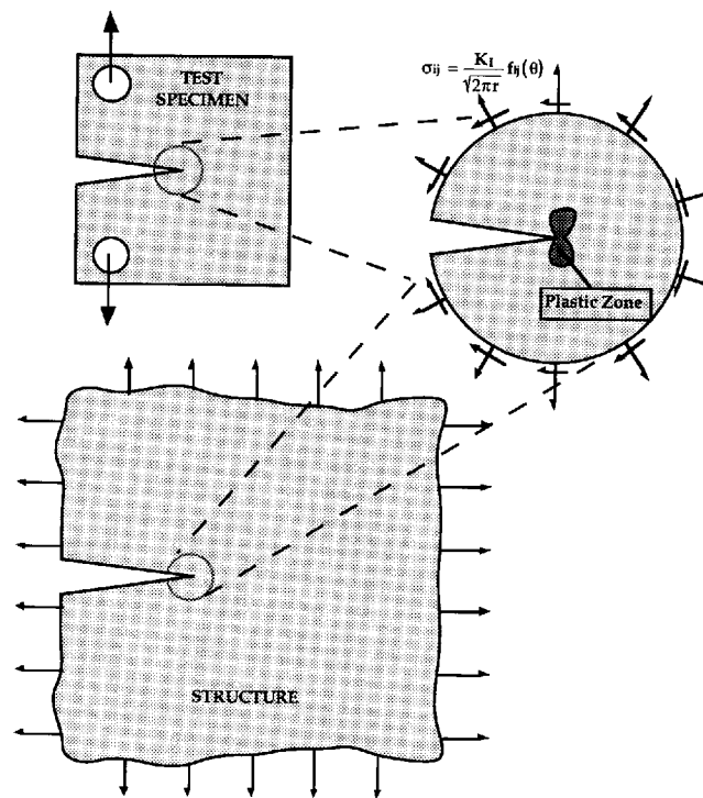
Figure 3-13 Schematic of crack-tip plasticity in test specimen and structure.
