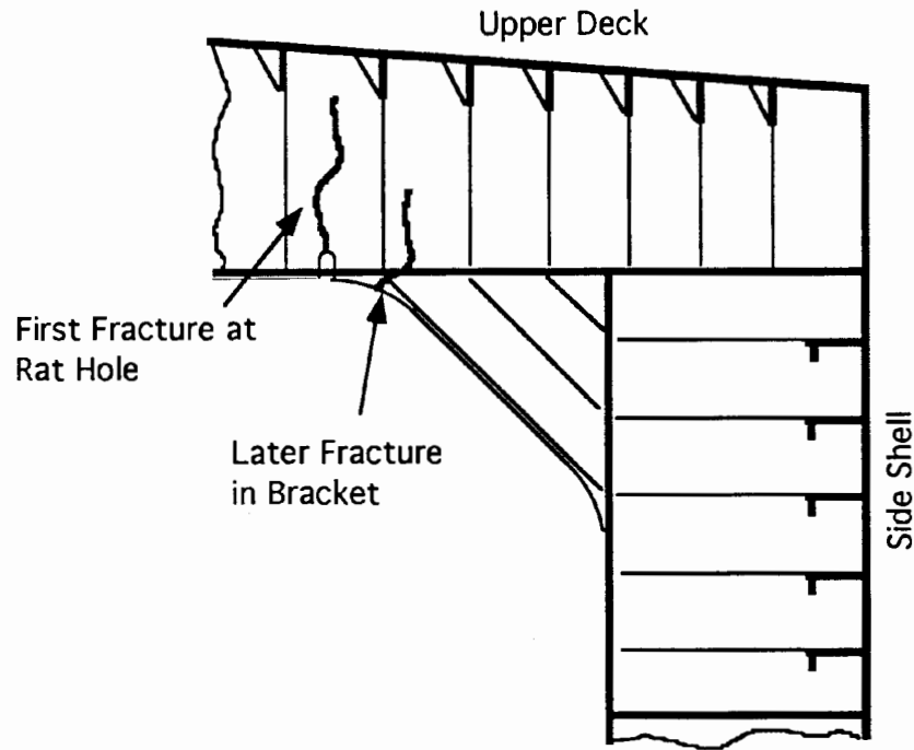
Figure 3-11 Typical Crack Initiation Sites
