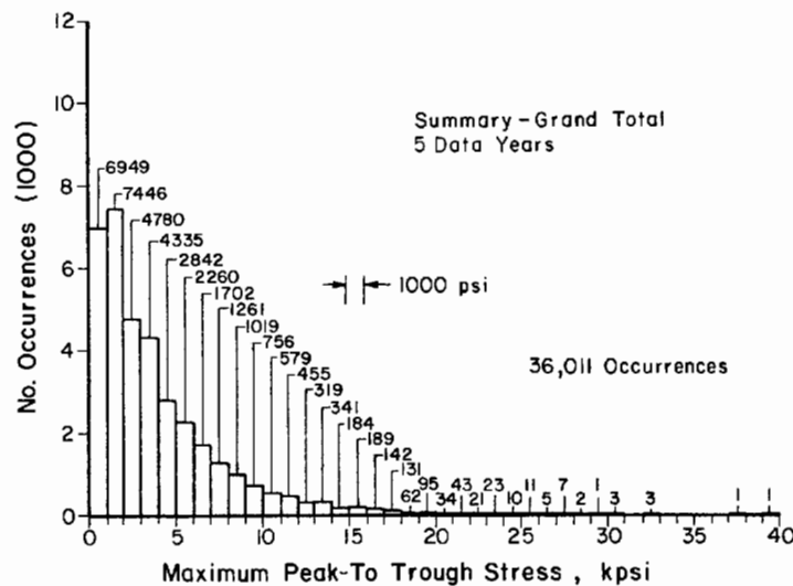
Figure 4-1 Stress histogram reproduced from Figure 6.7 of SSC 318 (Each occurrence is approximately 1920 cycles)
