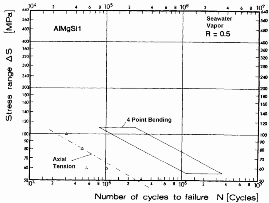
Figure E-2; Transversely welded plate subjected to both axial tension and 4 point bending; Alloy AlMgSi1; R-ratio = 0.5;
