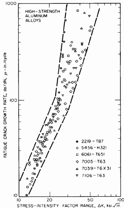
Figure 3-15 Actual FCGR data for various aluminum alloys in a benign environment.
