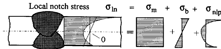
Figure 4-7 Local Stress Concentrations Due to Service and Residual Stresses
