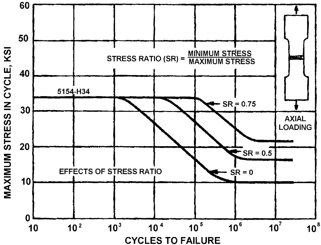
Figure 3-7 Effects of Stress Ratio on 5154-H34 Aluminum
