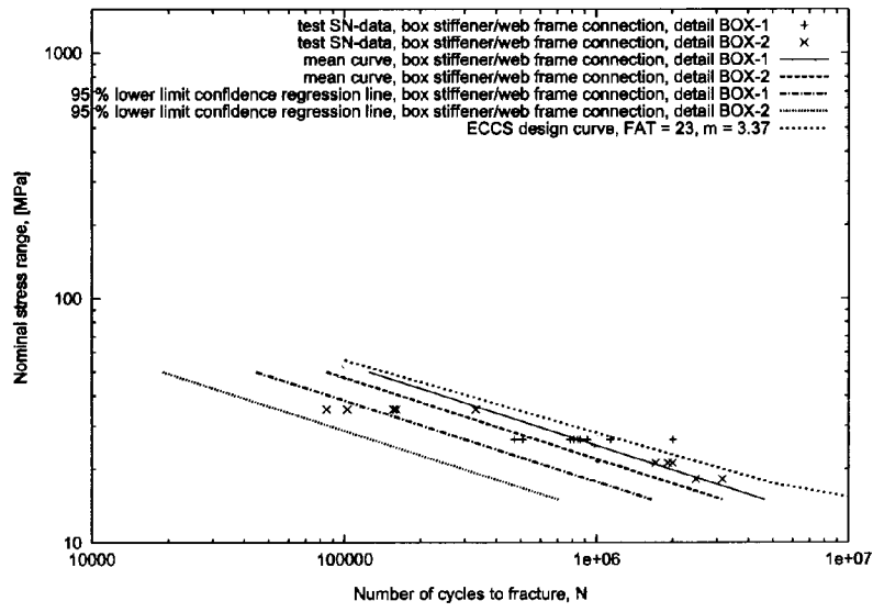
Figure E-19; Box 1 (Joint 27) and Box 2 (Joint 28); Alloy 5083; R = 0.44; Tension;
