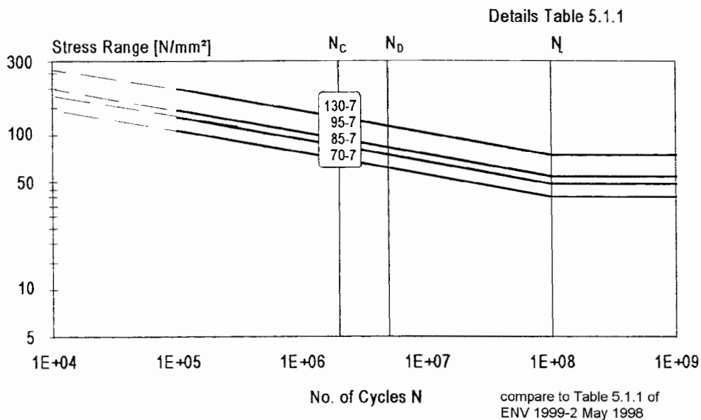
Fig. 5.2.1* Design Curves \Delta\sigma - N for plain material detail categories in Table 5.1.1*
