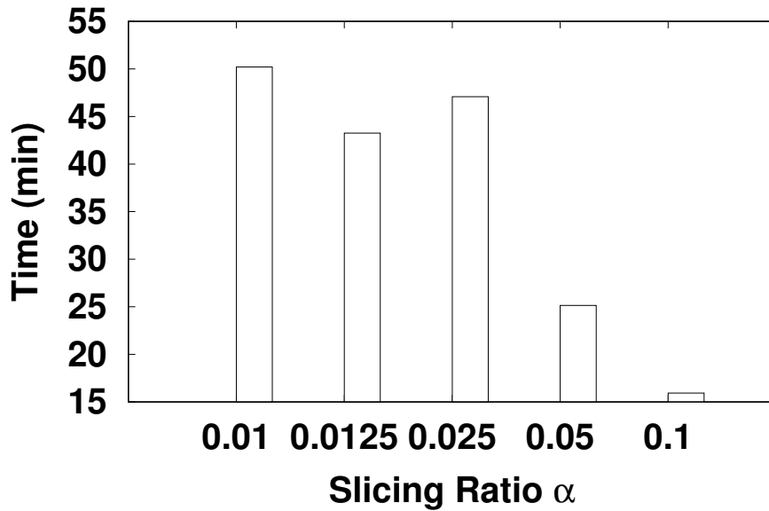
Fig. 15 Data-partition
