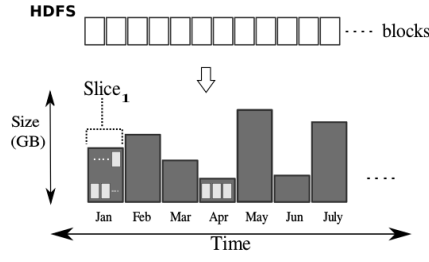
Fig. 6 Time-Slice
