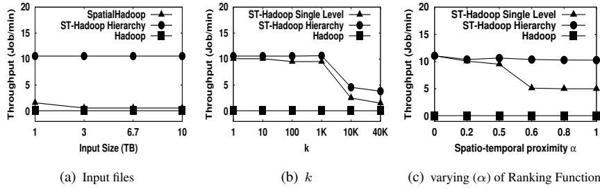
Fig. 17 Spatio-temporal K -Nearest-Neighbor Query
