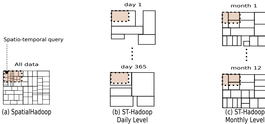
Fig. 3 HDFSS in ST-Hadoop VS SpatialHadoop
