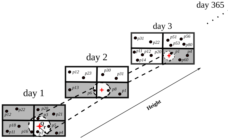
Fig. 9 Correctness Check when 0 \leq \alpha \leq 1
