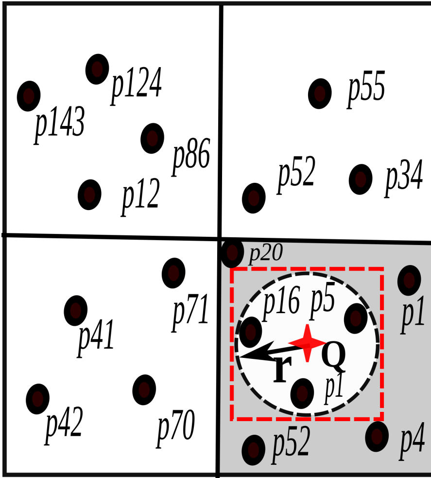
Fig. 8 Correctness check Final Answer
