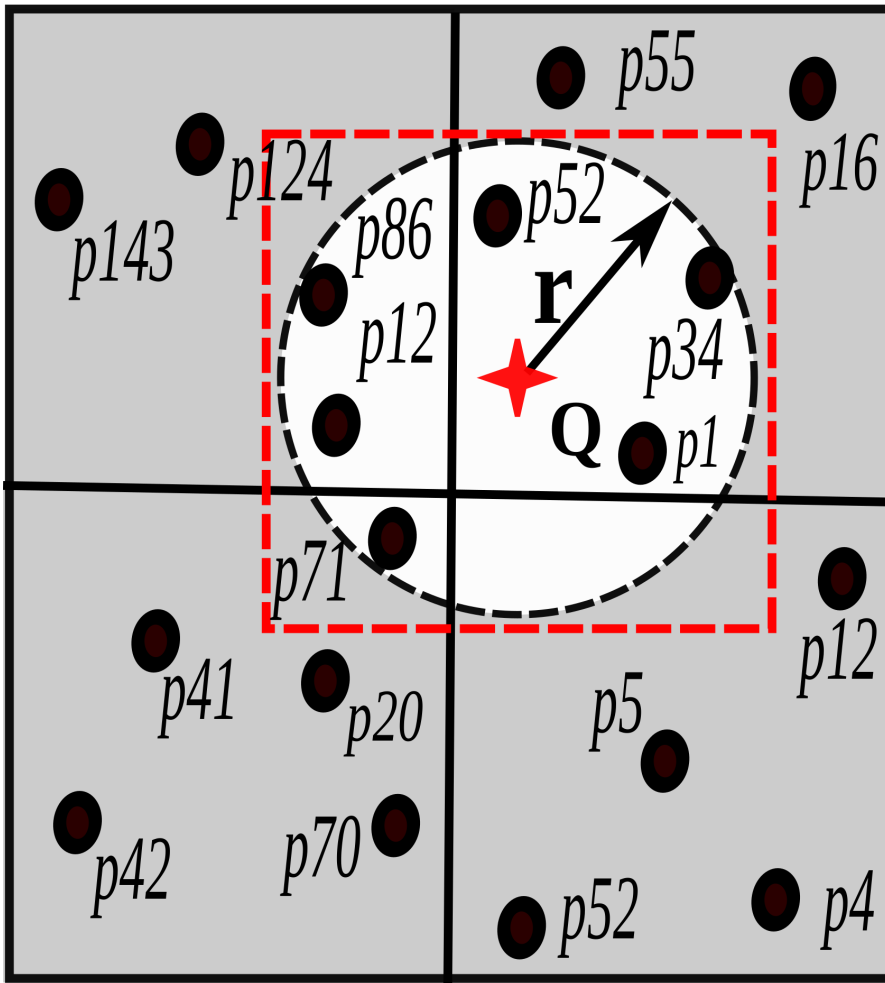
Fig. 10 Refinement Final Answer
