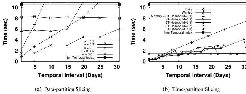
Fig. 19 Spatio-temporal Range Query Interval Window
