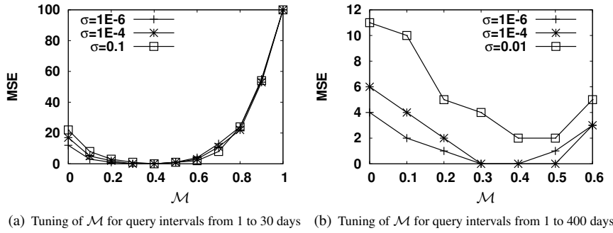
Fig. 20 The effect of the spatio-temporal query ranges on the best value of \mathcal{M}
