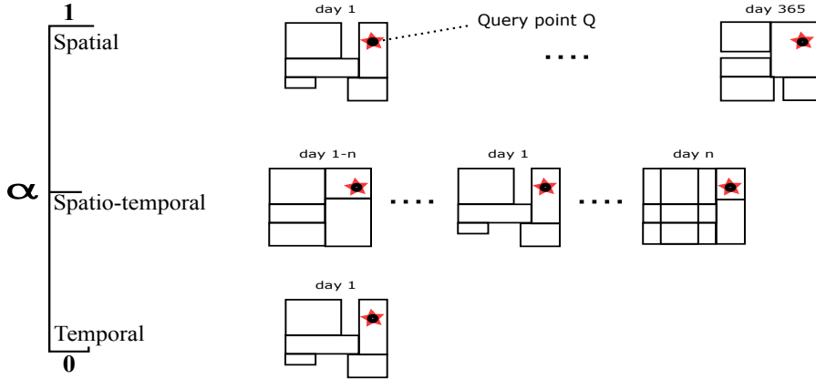
Fig. 7 Landscape of spatio-temporal k NN operation
