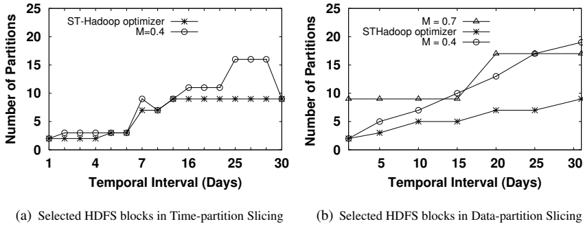
Fig. 21 ST-Hadoop Greedy query optimizer VS heuristic \mathcal{M}
