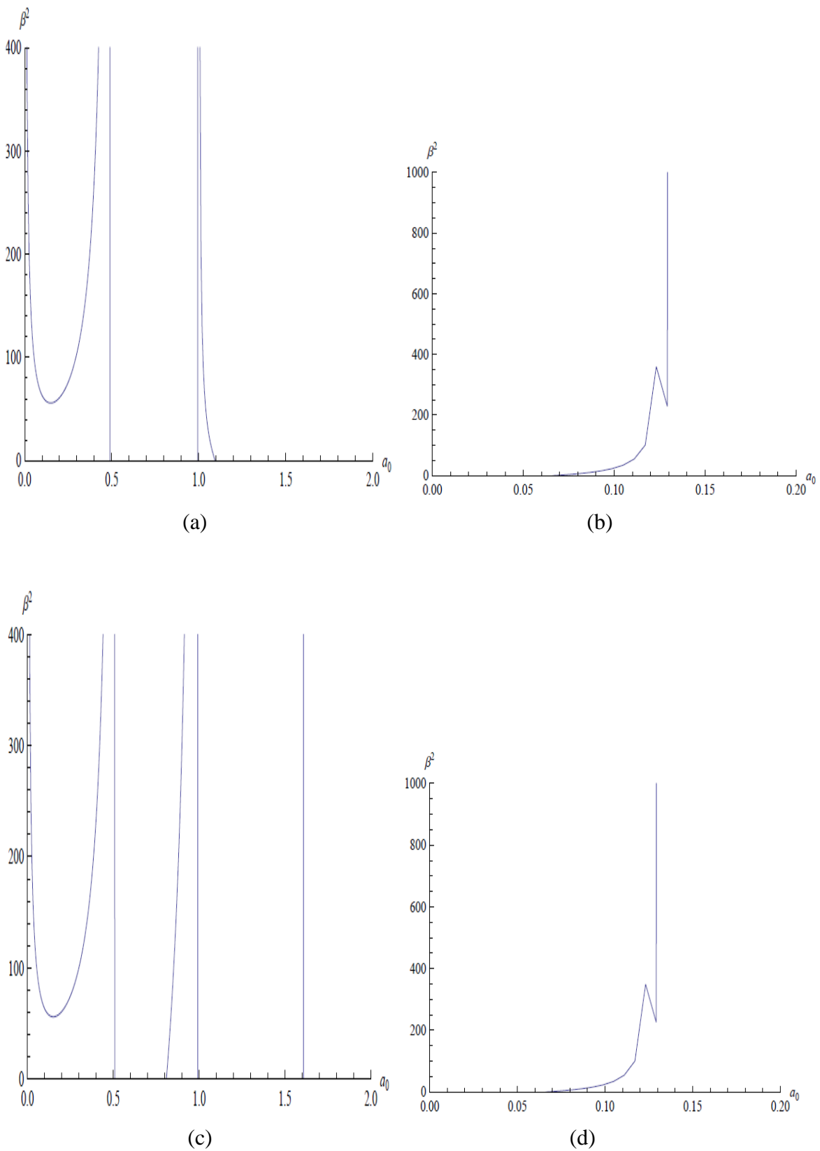
Figure 2. Stability regions TSW corresponding to \omega = 0.4 and the fixed value m = 1 :
