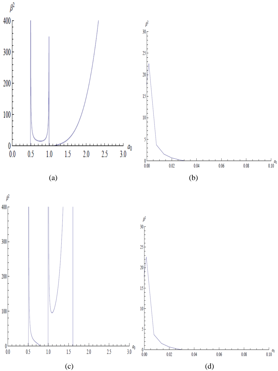
Figure 5. Stability regions TSW corresponding to \omega = 2 and the fixed value m = 1 :
