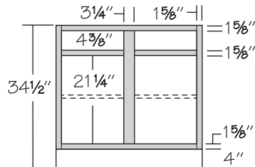
Standard Base Cabinet w/ Center Stile
