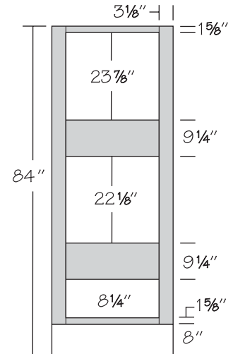
Universal Design Oven Cabinet
