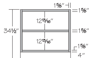
Furniture Drawer Cabinet 6" High
