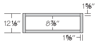
Wall Cabinet 12" High
