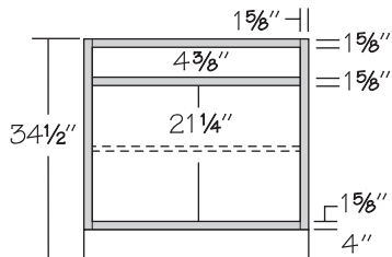
Standard Base Cabinet with Butt Doors
