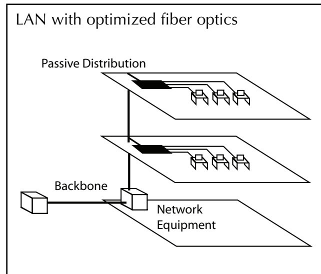
Figure 2. Cabling for centralized fiber architecture.
