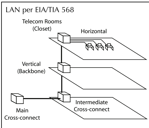
Figure 1. Structured cabling architecture per TIA/EIA 568.
