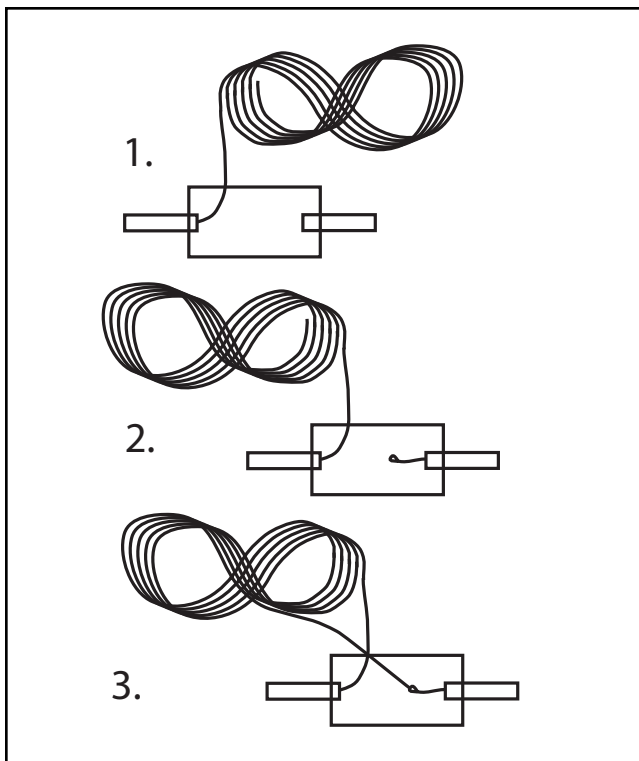
Figure 3. Use “figure 8” loops to protect the cable when pulling.
