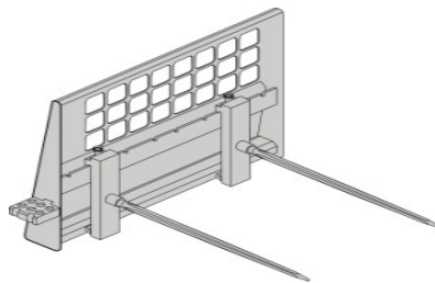
Bale Forks and Frame
