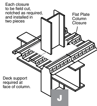
COLUMN CLOSURE DETAIL
