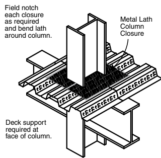
COLUMN CLOSURE DETAIL
