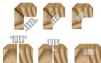
For mitre joint & butt joint
