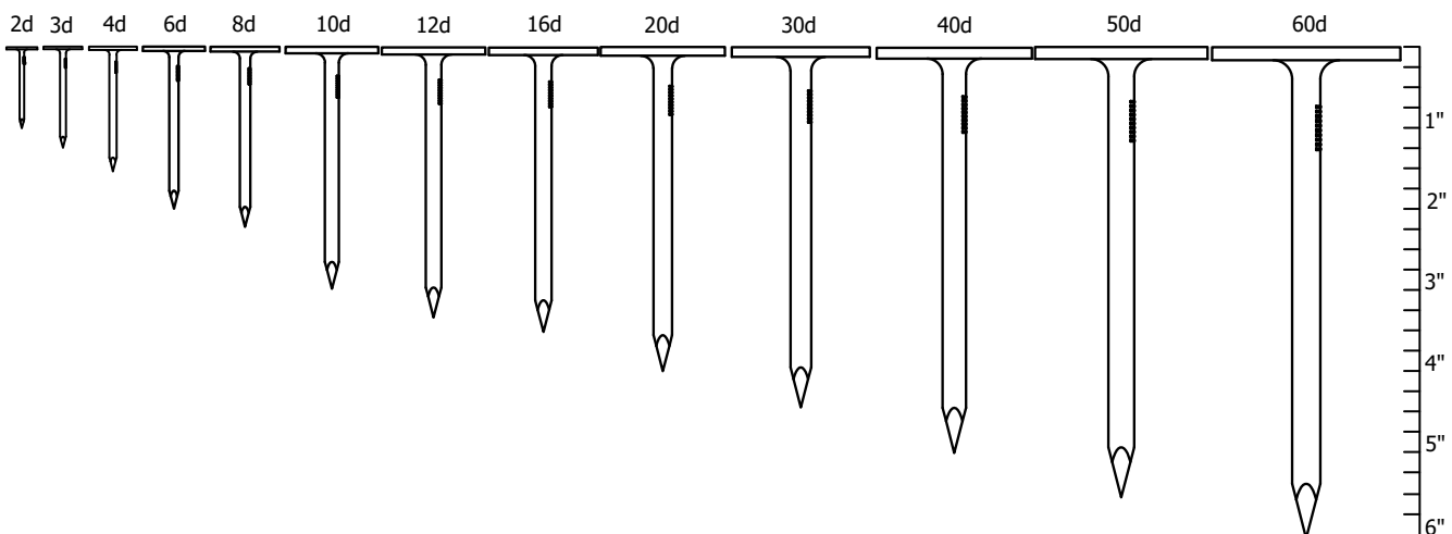
Clout nails — smooth shank
