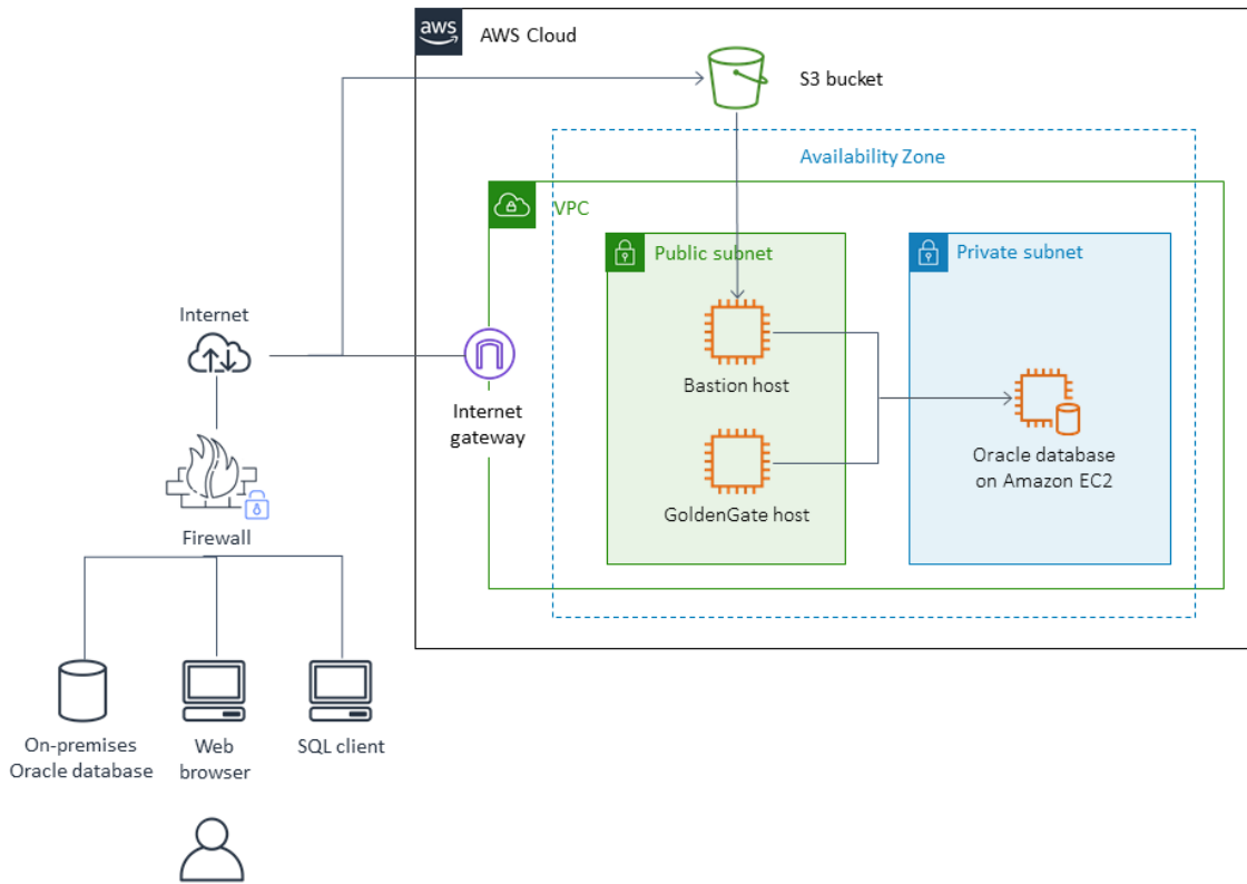
Oracle GoldenGate replication from on-premises to Oracle Database on Amazon EC2
