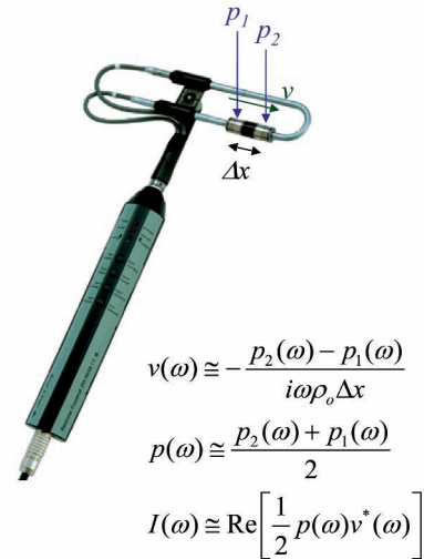
Fig. 16. Hand-held acoustic intensity probe. Two microphones are separated by a known distance \Delta x so that particle velocity may be computed using a finite difference approximation. The mean pressure and estimated particle velocity are combined to compute the active, or real part of acoustic intensity in the direction along the x -axis.
