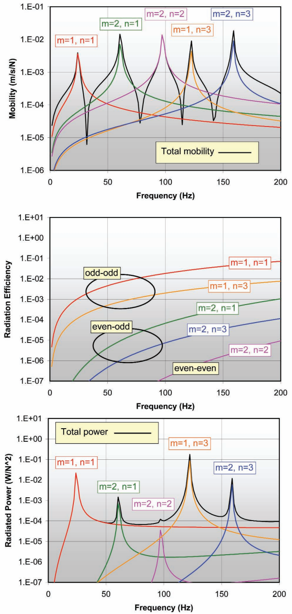
Fig. 9. Mobility magnitude (top), radiation efficiency (middle), and radiated sound power transfer function (bottom) of a simply supported 1m square 5 mm thick flat steel plate in water driven at its quarter point ( x=0.25 m, y=0.25 m).
