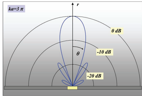
Fig. 3. Sound intensity distribution in the far-field of a radiating baffled piston, ka=3\pi .
