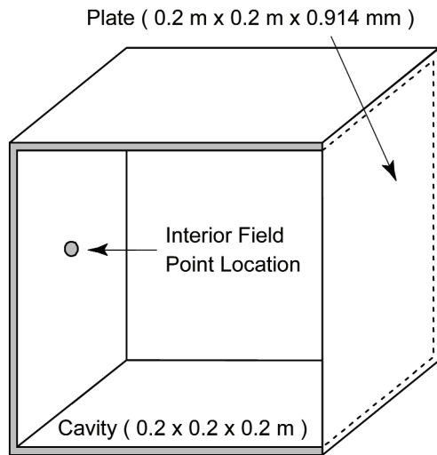
Fig. 19. Dimensions for the cavity-backed plate example problem.
