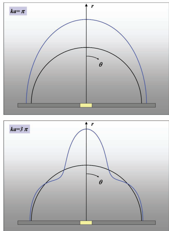
Fig. 2. Pressure distribution in the far-field of a radiating baffled piston. Top – ka = \pi ; Bottom – ka = 3\pi .
