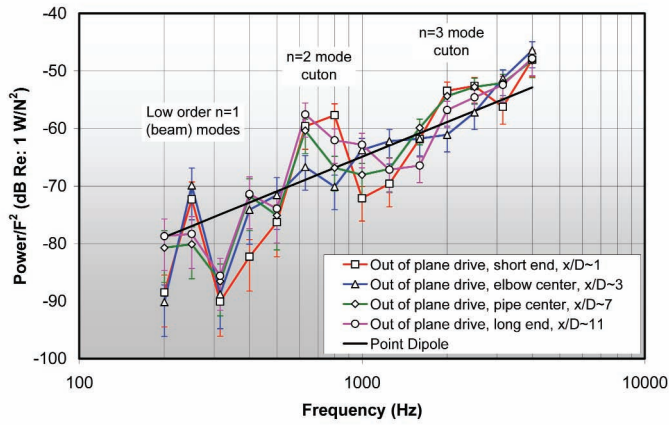
Fig. 14. Sound power radiated by Schedule 10 Steel 3 inch pipe with elbow, pipe length/diameter~12.
