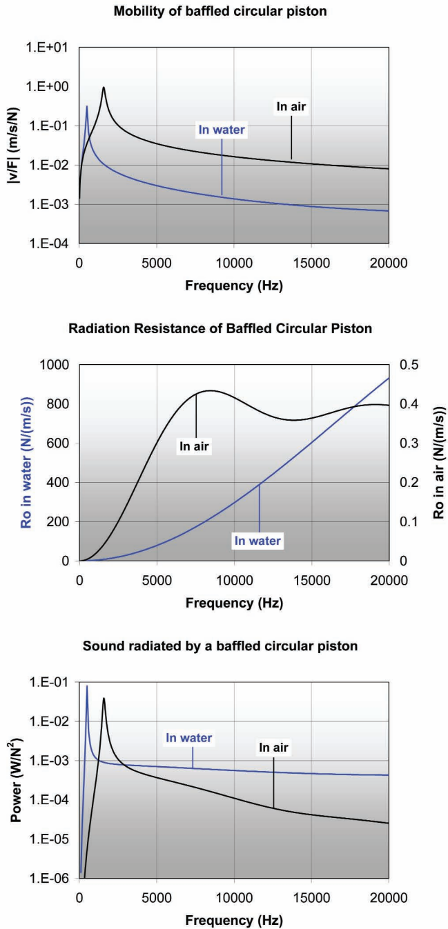
Fig. 5. Mobility magnitudes (top), radiation resistances (middle), and radiated sound power transfer functions (bottom) of a 16.6 mm radius circular baffled piston in air (black) and in water (blue).
