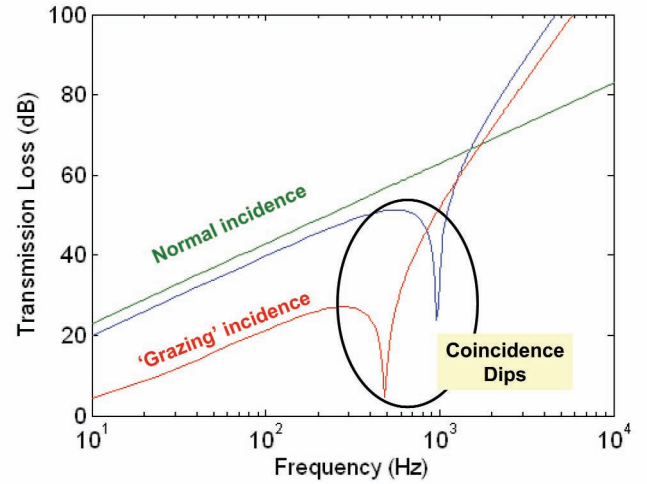
Fig. 11. Typical transmission loss plot for variable angles of incidence. Grazing incidence refers to acoustic waves that are nearly in the plane of the plate.
