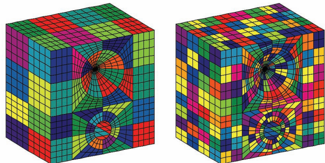
Fig. 17. A structural mesh for a speaker with two different acoustic meshes.
