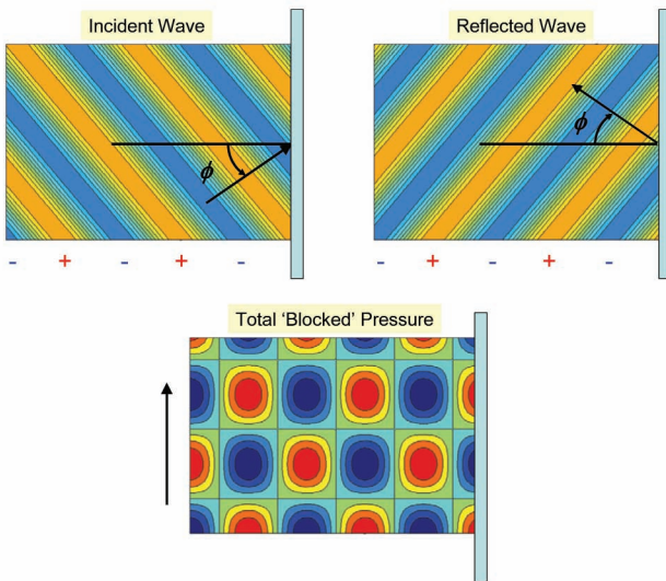
Fig. 10. Blocked pressure field acting on a plate (right side of images) at 30 degree angle of incidence. '+' and '-' signs indicate phase variations in the waves.
