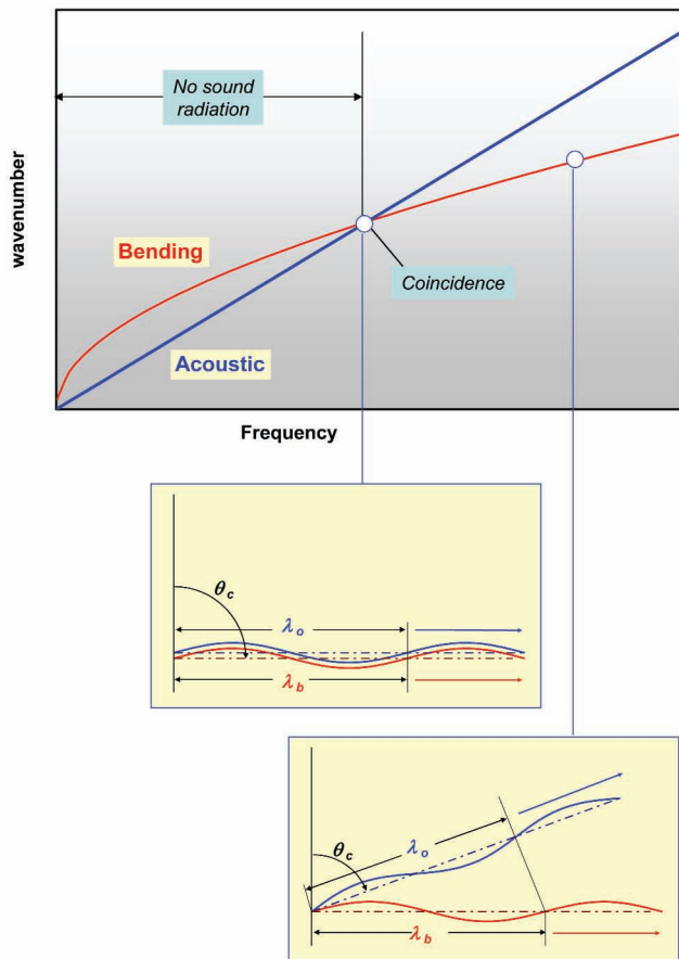
Fig. 6. Bending and acoustic wavenumber-frequency plot, with trace diagrams of bending and acoustic waves at and above coincidence. Below coincidence, an infinite bending wave radiates no sound!
