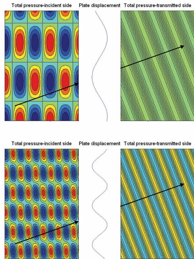
Fig. 12. Incident and transmitted sound fields around an infinite 25 mm thick steel plate, 30 degree angle of incidence. Top—at 50% of coincidence, Bottom—at coincidence. Dark blue and red indicate high pressures, and green indicates low pressures.
