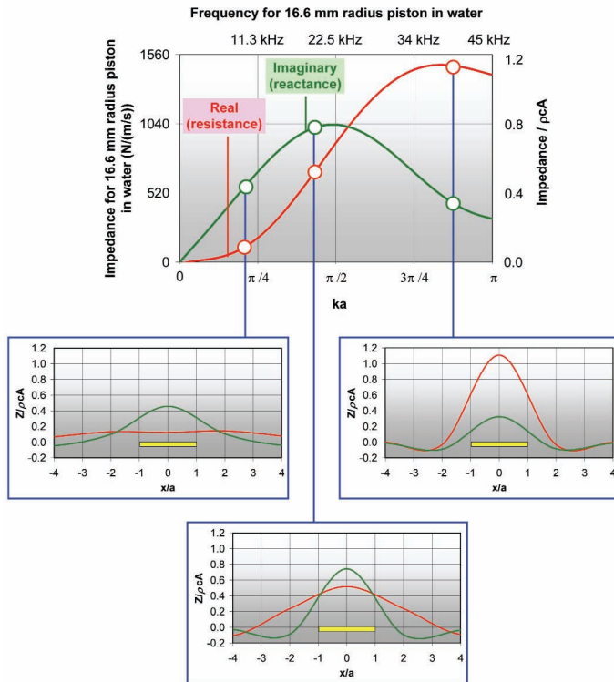
Fig. 4. Radiation impedance of baffled circular piston. Top—resistance and reactance as a function of frequency (and ka ); Bottom—spatial variability of resistance and reactance at three discrete frequencies.
