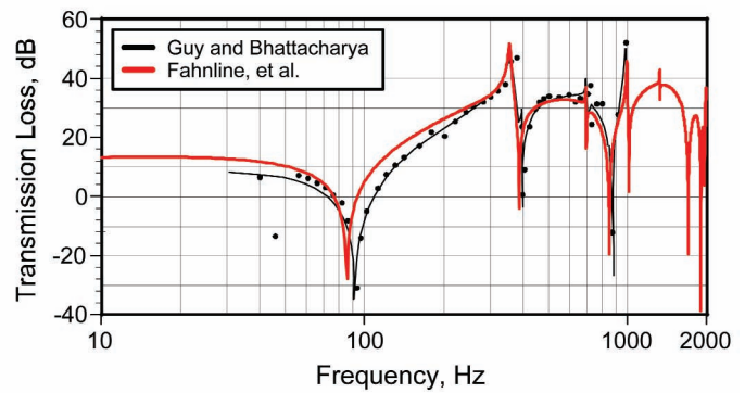
Fig. 20. Transmission loss as a function of frequency for a cavity-backed plate.
