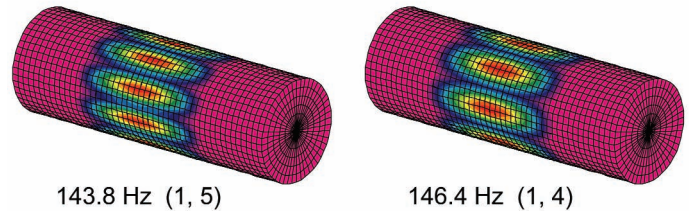
Fig. 18. Finite element predictions for the first two mode shapes and resonance frequencies of a thin shell. The rigid ends on both sides of the shell simulate semi-infinite rigid baffles.
