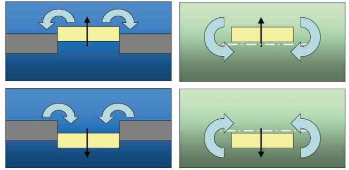
Fig. 1. Low frequency vibration and acoustic fluid motion of a piston. Left – baffled piston; Right – unbaffled piston.
