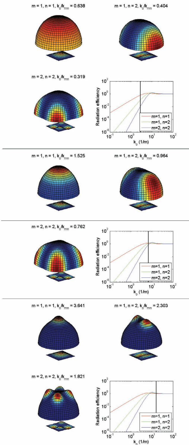
Fig. 8. Far-field sound intensity in air for various low-order simply supported 1 m square flat plate modes. Top—below coincidence, Middle—near coincidence, Bottom—above coincidence.
