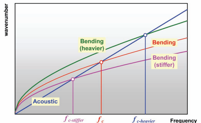
Fig. 7. Effects of stiffening and mass-loading on plate coincidence frequencies. Stiffening a plate reduces the coincidence frequency, and adding mass increases it.
