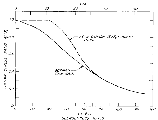
Figure 15.—Column allowable design stress as a function of slenderness ratio ( l/r ) in Germany and North America. (Curves based upon E/F_c = 268.5 .) (M149 820)
