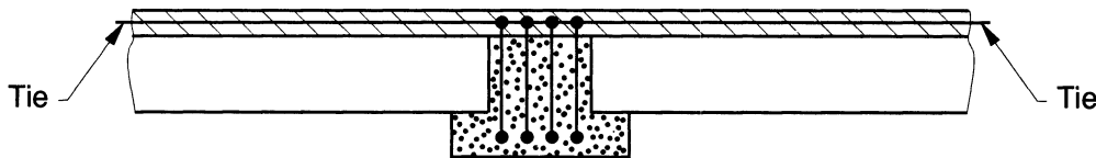
Figure 5.3 — Continuity of ties: bars lapped within in situ concrete
