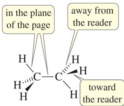
ethane
