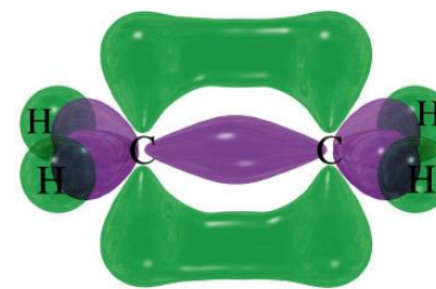
ethylene
