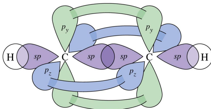
acetylene
