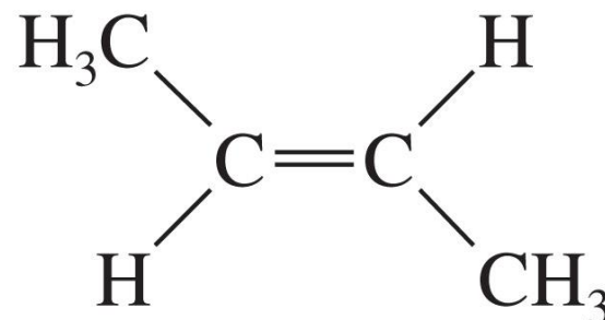
trans -but-2-ene
