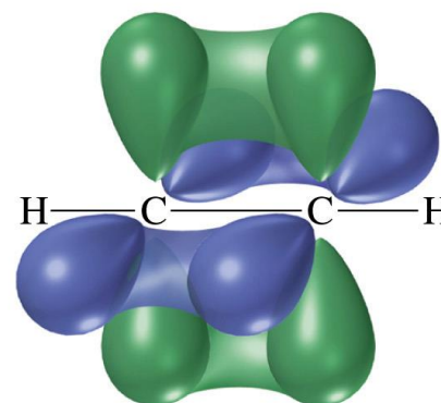
acetylene
