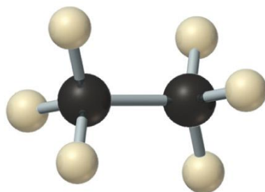
ethane
