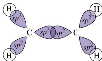
σ bond framework (viewed from above the plane)
