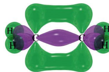
ethylene
