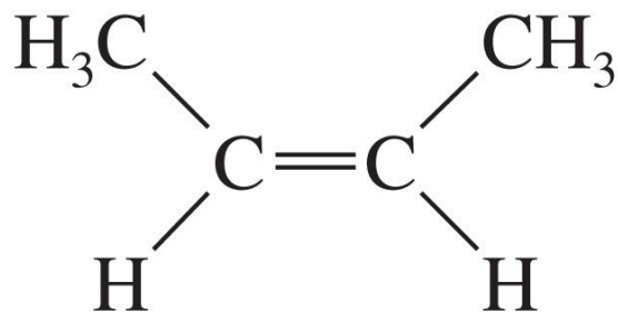
cis -but-2-ene
