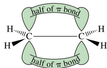
π bond (viewed from alongside the plane)
