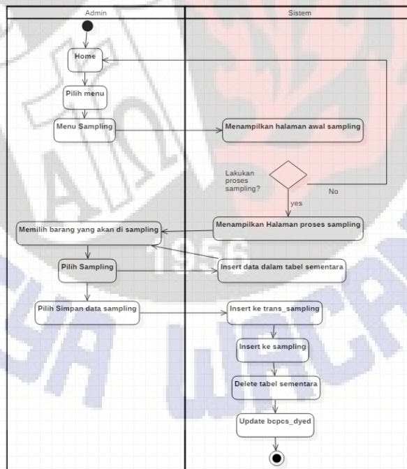
Activity diagram proses sampling kain
