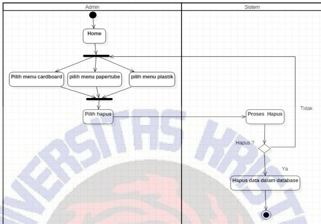
Activity diagram hapus data(cardboard,papertube,plastik)
