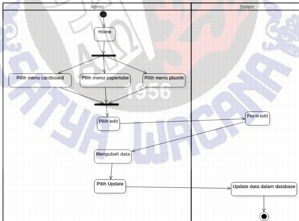
Activity diagram edit data (cardboard,papertube,plastik)
