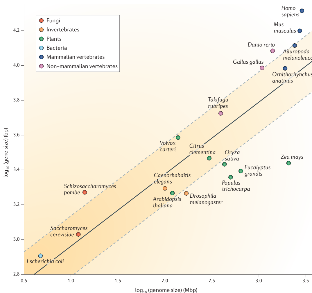
Figure 1 | Genome and gene sizes for a representative set of genomes. Gene size is plotted as a function of genome size for some representative bacteria, fungi, plants and animals. This figure illustrates a simple rule of thumb: in general, bigger genomes have bigger genes. Thus, accurate annotation of a larger genome requires a more contiguous genome assembly in order to avoid splitting genes across scaffolds. Note too that although the human and mouse genomes deviate from the simple linear model shown here, the trend still holds. Their unusually large genes are likely to be a consequence of the mature status of their annotations, which are much more complete as regards annotation of alternatively spliced transcripts and untranslated regions than those of most other genomes.
