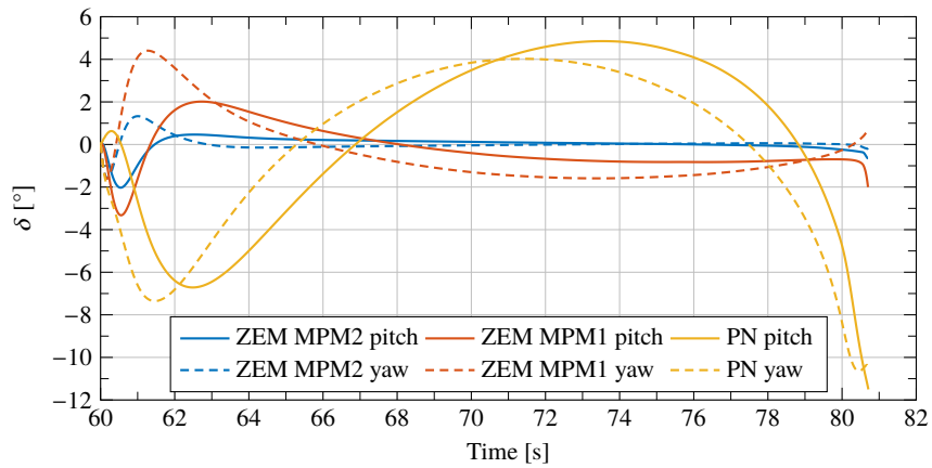
(c) Actuator deflection angle
