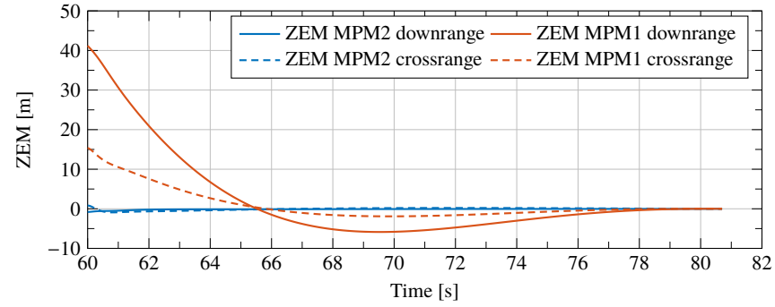
(a) ZEM offsets
