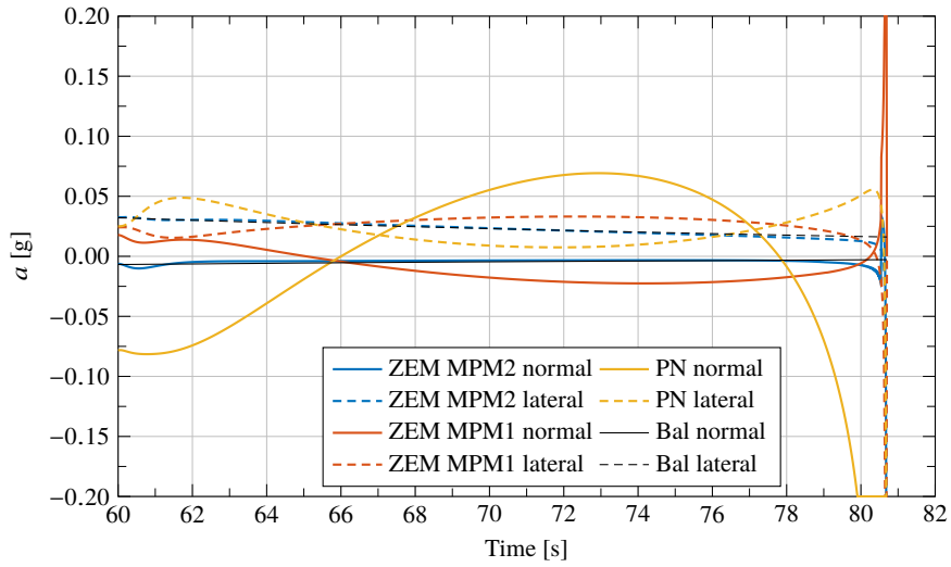
(b) ZEM and PN acceleration command and ballistic acceleration
