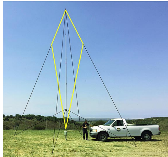
Figure 1: Loop vertical installed at my radio club's site. Loop wires (yellow), guys (black) highlighted for clarity.
