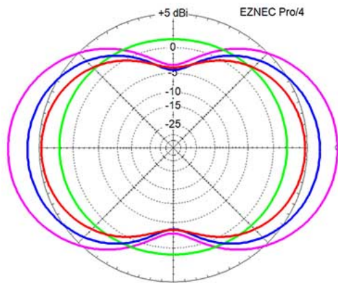
Figure 6: Azimuth patterns and gains. 20m: red, 15m: blue, 10m: green, 6m: violet
