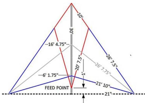
Figure 2: Dimensions of the kite-shaped wire-loop vertical (red) with a full set of guys (blue). Optional extra guys (gray)
