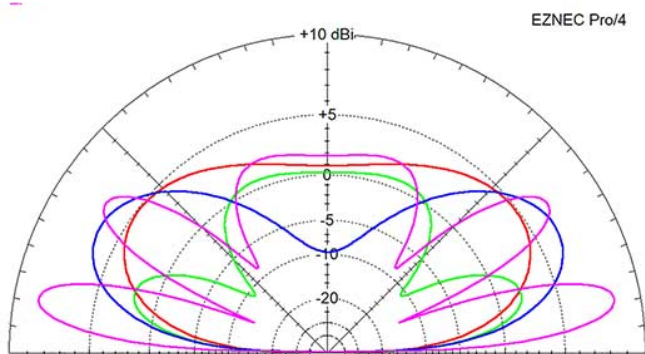
Figure 3: Elevation radiation patterns and gains on 20m: red, 15m: blue, 10m: green, 6m: violet
