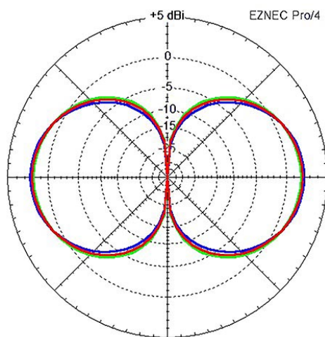
Figure 3: Radiation patterns and gains of a 40m dipole matched with a tuner and operated on 5 MHz (green), 7 MHz (red) and 9 MHz (blue).
