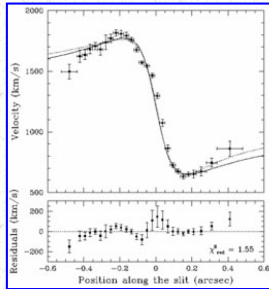
Figure 4. Optical emission-line rotation curve for the nuclear disk in M87 . The two curves in the upper panel correspond to Keplerian thin disk models, and the bottom panel shows the residuals for one of the models (see Macchetto et al. 1997 ).
