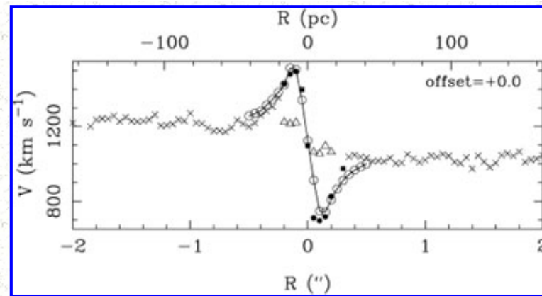
Figure 5. Optical emission-line rotation curve for the nuclear disk in M84 obtained with STIS on HST ( Bower et al. 1998 ). The kinematics can be well fitted with a thin Keplerian disk model, which is plotted as open circles connected by the solid line.
