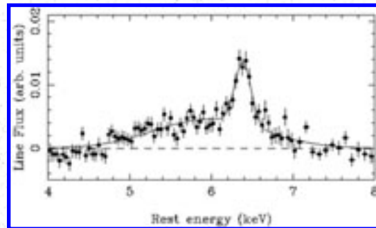
Figure 7. The Fe K\alpha line in the composite spectrum of Seyfert 1 nuclei ( Nandra et al. 1997 ). The solid line is a fit to the line profile using two Gaussians, a narrow component centered at 6.4 keV and a much broader, redshifted component.
