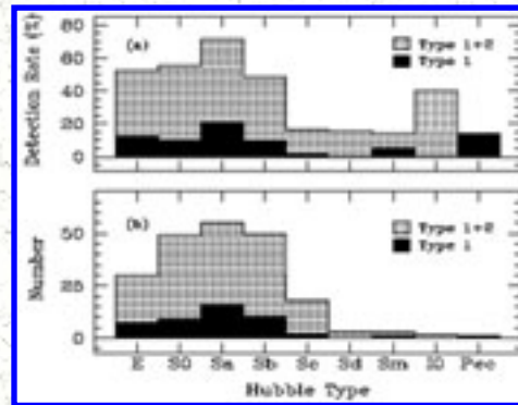
Figure 9. (a) Detection rate and (b) number distribution of AGNs as a function of Hubble type in the spectroscopic survey of Ho et al. ( 1995 , 1997 ). "Type 1" AGNs (those with broad H_{\alpha} ) are shown separately from the total population (types 1 and 2).
