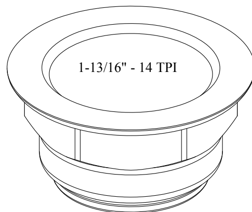
POLISHED CHROME DRAIN NUT FOR CRANE 122630-CP
