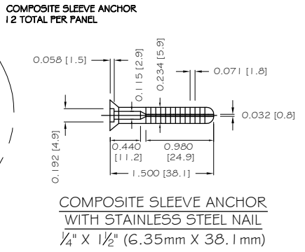
DETAIL B PANEL INSTALLATION
