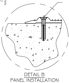
DETAIL B PANEL INSTALLATION
