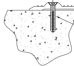
SECTION B-B PANEL INSTALLATION
