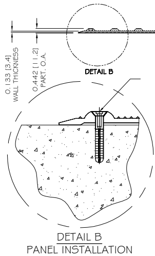
COMPOSITE SLEEVE ANCHOR WITH STAINLESS STEEL NAIL 1/4" X 1 1/2" (6.35mm X 38.1mm)
