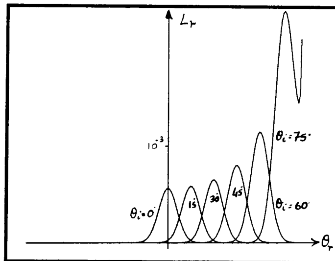
(f) \sigma_\alpha = 3.0
