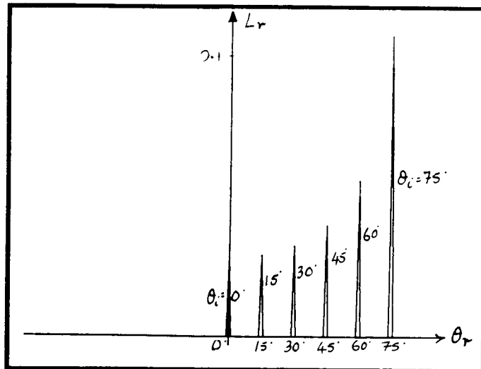
(b) \sigma_\alpha = 0.1
