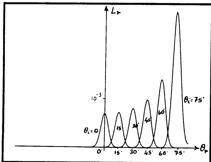
(e) \sigma_\alpha = 2.0
