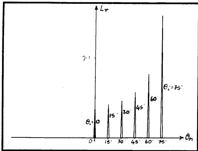
(a) \sigma_\alpha = 0.01
