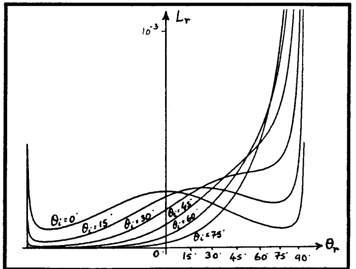
(f) \sigma_\alpha = 17.0
