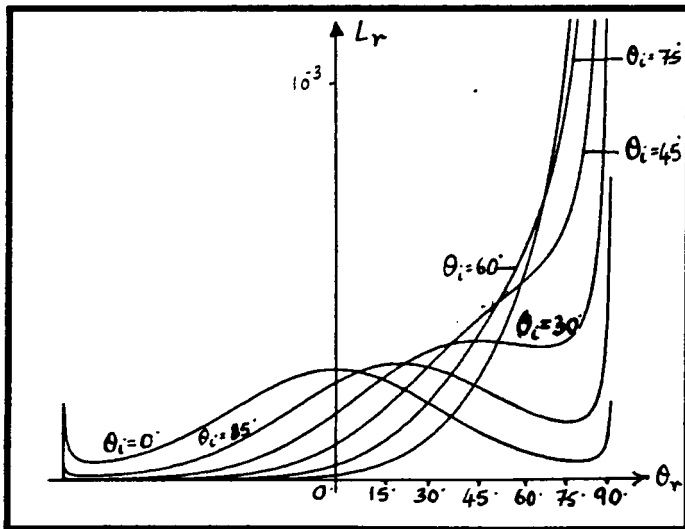
(e) \sigma_\alpha = 15.0
