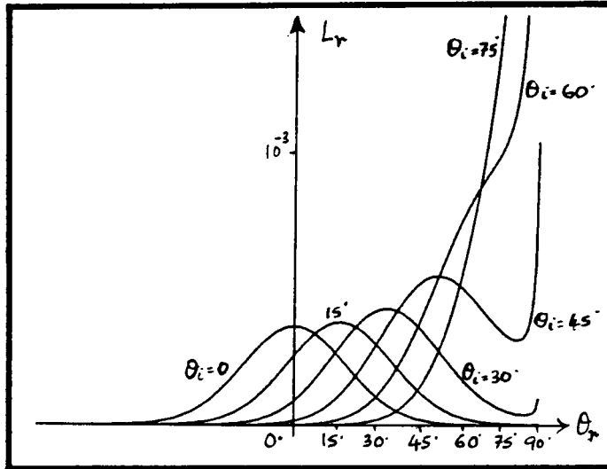
(c) \sigma_\alpha = 9.0
