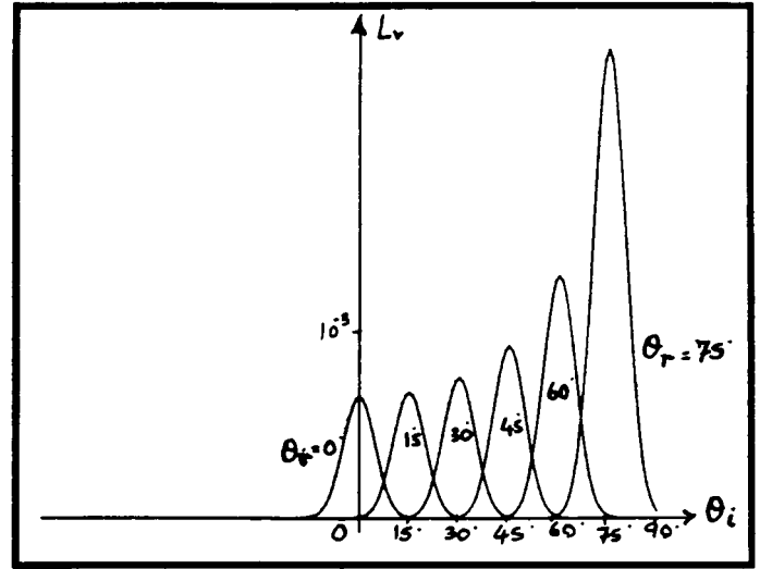
(b) \sigma_\alpha = 2.428
