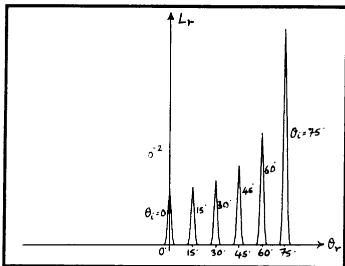
(c) \sigma_\alpha = 0.5
