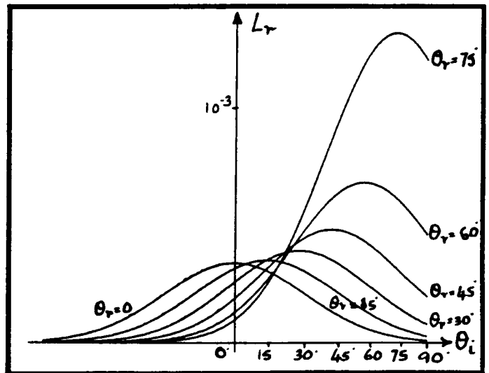
(f) \sigma_\alpha = 15.416
