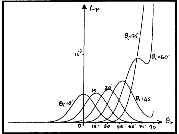
(b) \sigma_\alpha = 7.0
