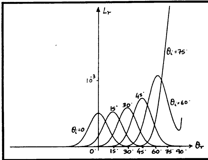
(a) \sigma_\alpha = 5.0
