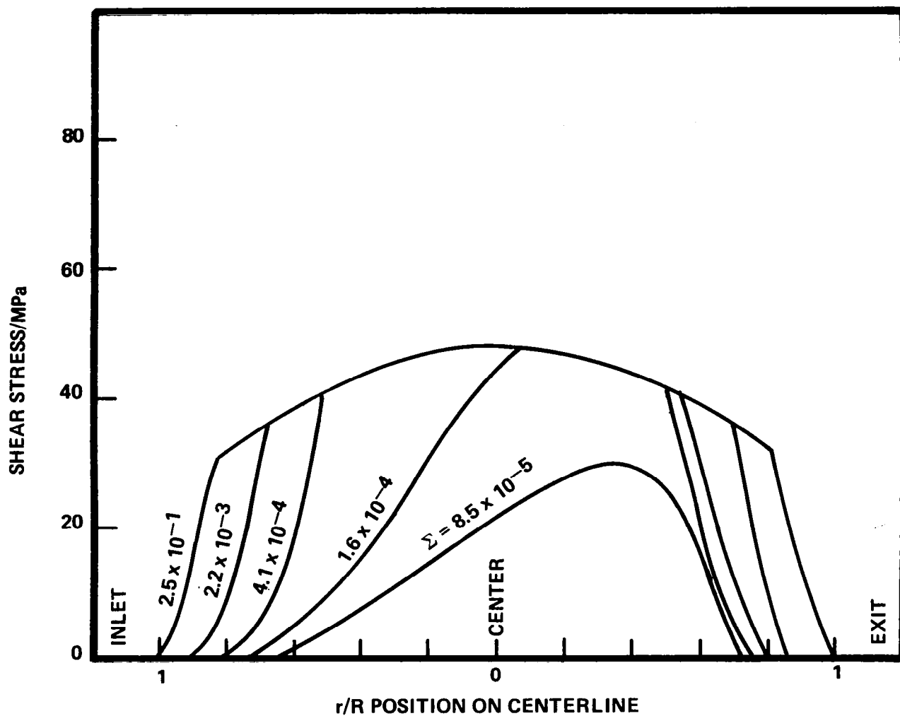
Figure 22. Predicted shear stress distribution in point contact for Santotrac 50 at 20°C, 0.5 GPa Hertz pressure, 0.22 m/s rolling speed and indicated slide roll ratios based on equation (5) and measured data
