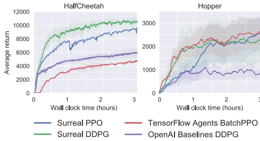
Figure 7: Training curves with 16 actors: our SURREAL algorithms and baselines on OpenAI Gym HalfCheetah and Hopper environments.
