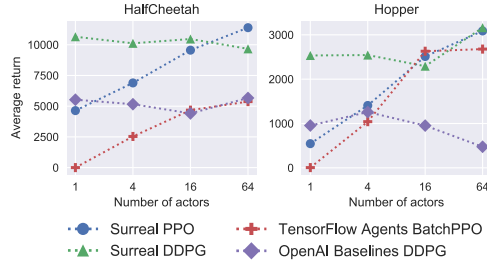
Figure 9: Scalability with respect to the number of actors: our methods v.s. baselines on gym HalfCheetah and Hopper environments.
