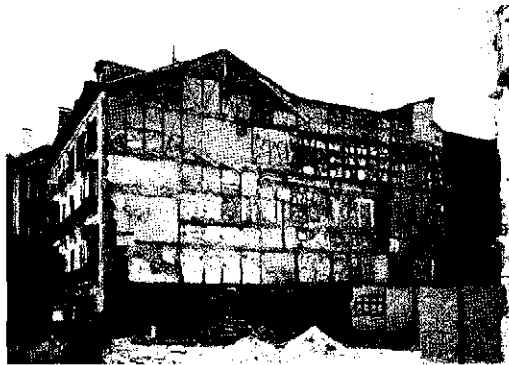
Figure 2 Timber and masonry infill-frame construction near the Plaza Mayor in Madrid
