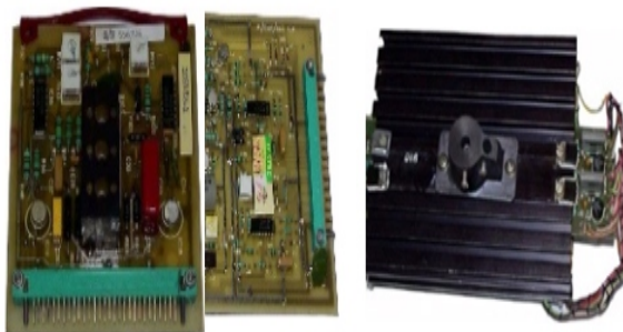
Main PCB board for SASAKURA ODM system
