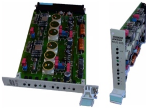
MUS925 Foxboro Eckardt cards for Power Supply Unit for Intelligent Transmitter
