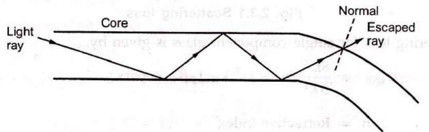
Fig. 2.4.1 Bending loss
