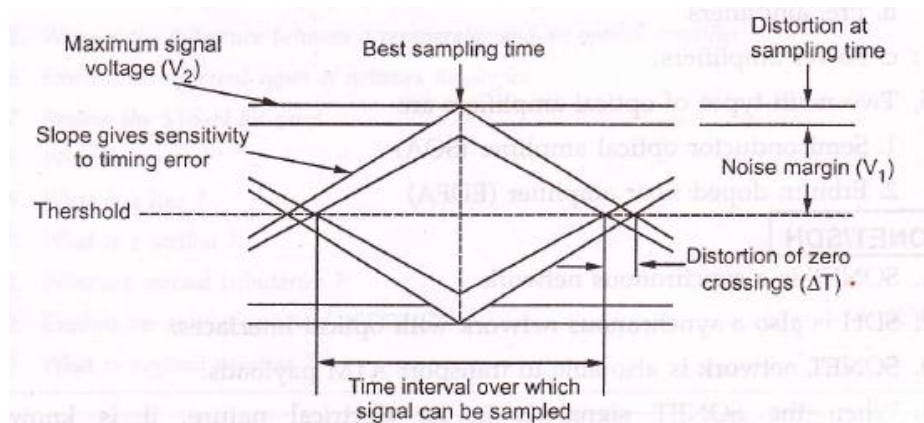
Fig. 8.7.4 Simplified Eye-diagram with key performance parameters
