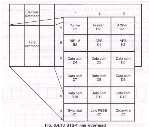
Fig. 8.4.13 STS-1 line overhead
