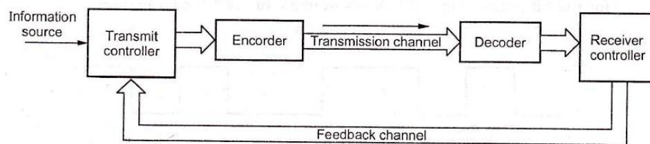
Fig. 6.2.6 ARQ scheme
