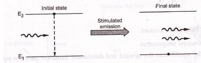
Fig. 3.1.9 Stimulated emission
