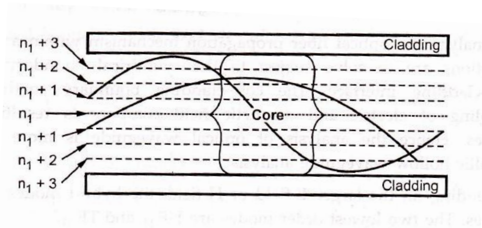
Fig. 1.6.19 Light trajectories in a graded index fiber
