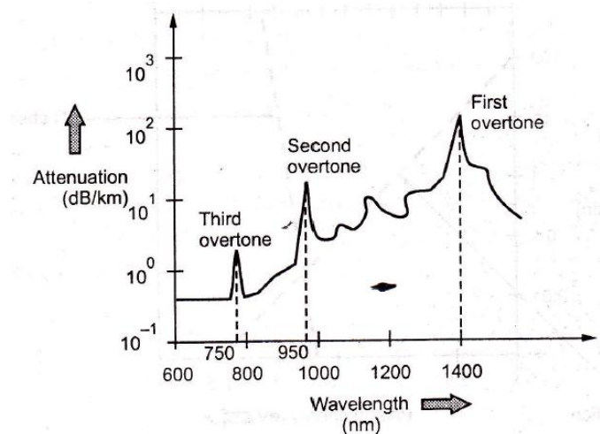
Fig. 2.2.2 Absorption spectra for OH group
