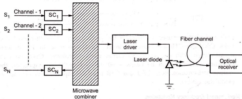
Fig. 6.1.5 Sub-carrier multiplexing
