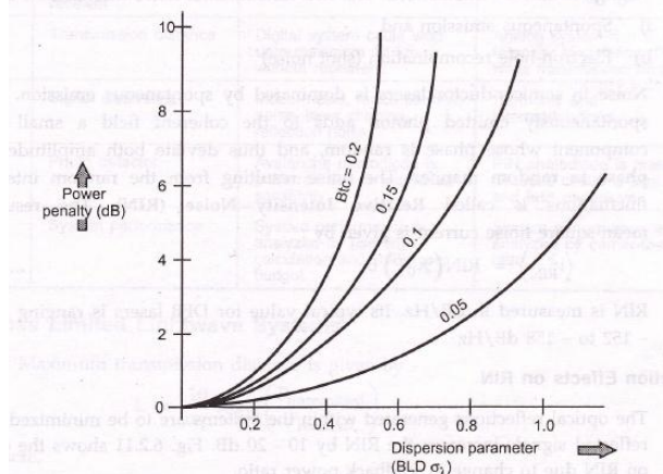
Fig. 6.2.10 Chirp induced power penalty
