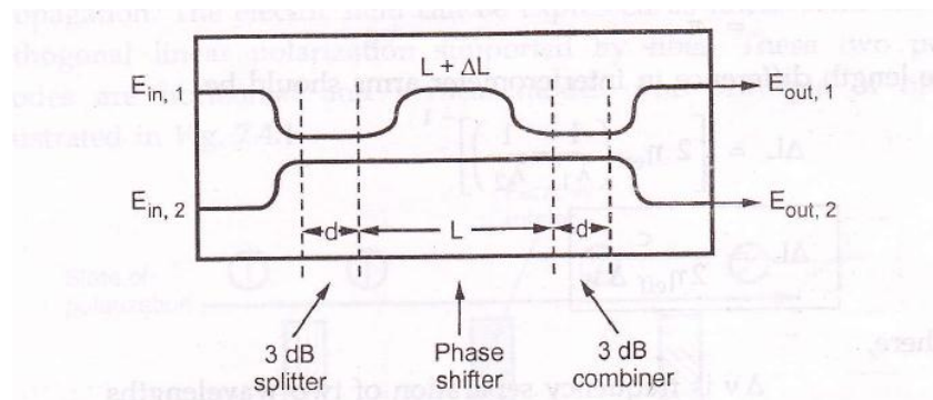
Fig. 7.3.1 Layout of 2 × 2 passive Mach-Zehnder Interferometer
