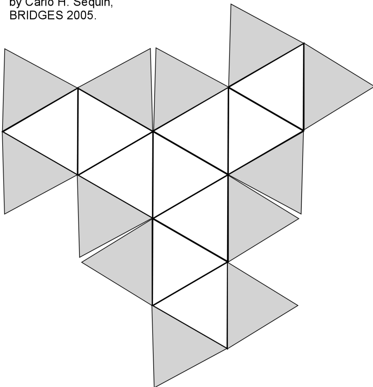
Net of the symmetrical dissection of the icosahedron (see Fig. 2d)
