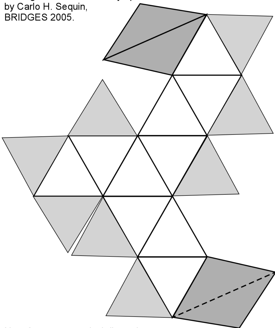
Net of an asymmetrical dissection of the icosahedron (see Fig. 2e)
