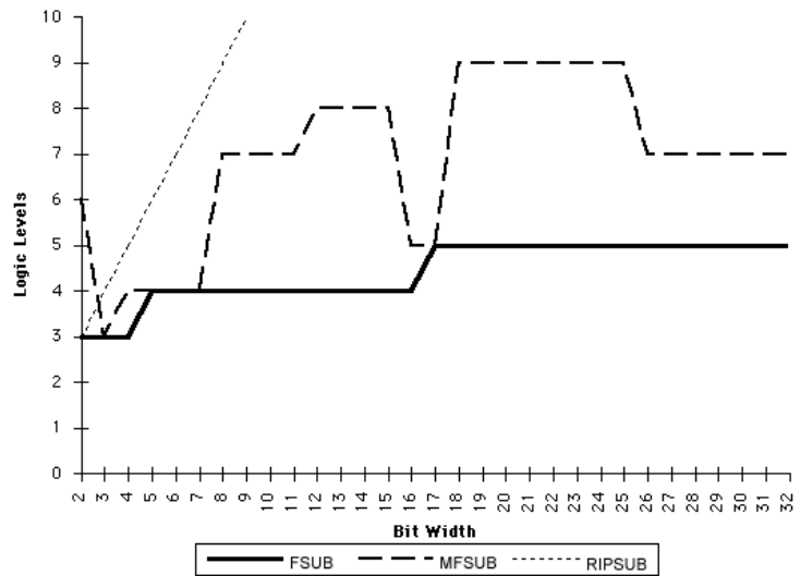
Figure B-13. Subtractor Logic Level
