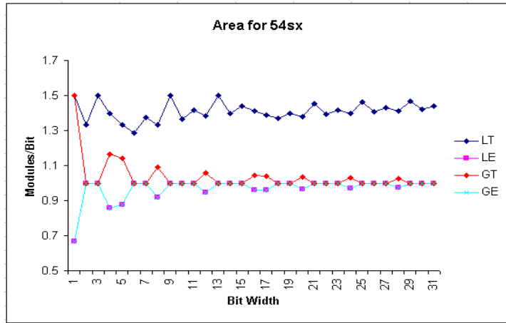
Figure B-18. Area and Module Count For 54SX/54SX-A/eX/A500K
