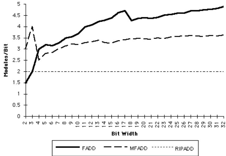
Figure B-8. Adder Module Count
