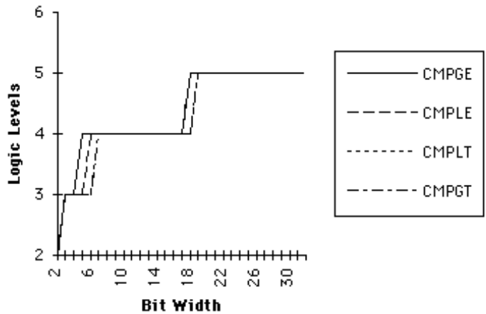
Figure B-17. Comparator Logic Levels
