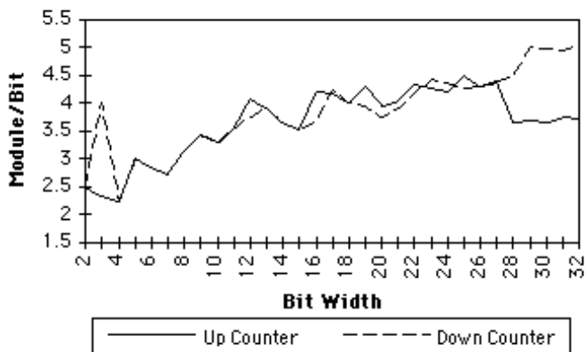
Figure B-20. Counter Module Count
