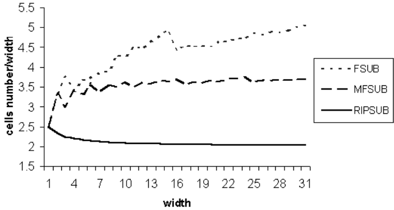
Figure B-14. 54SX/54SX-A/eX/A500K Subtractor Module Count
