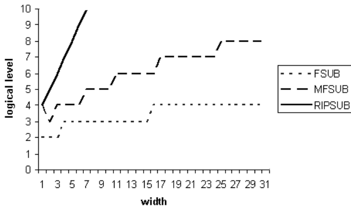
Figure B-15. 54SX/54SX-A/eX/A500K Subtractor Logic Level
