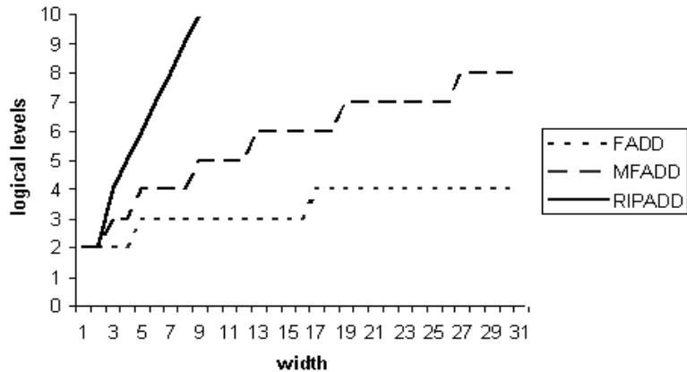
Figure B-11. 54SX/54SX-A/eX/A500K Adder Logic Level
