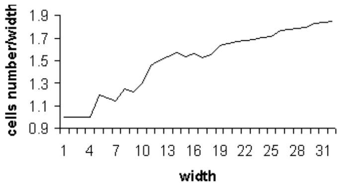
Figure B-22. Incrementer Module Count
