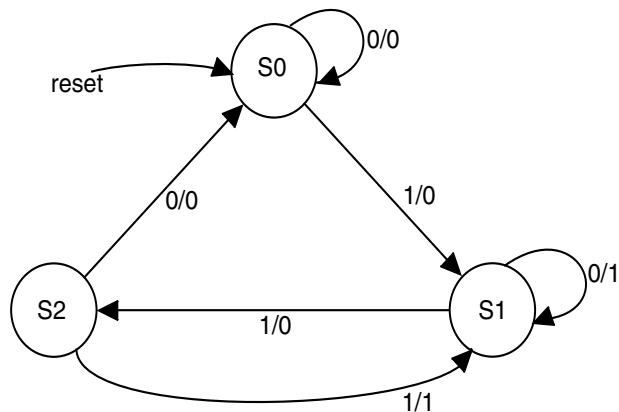
Figure 3-2. FSM Diagram
