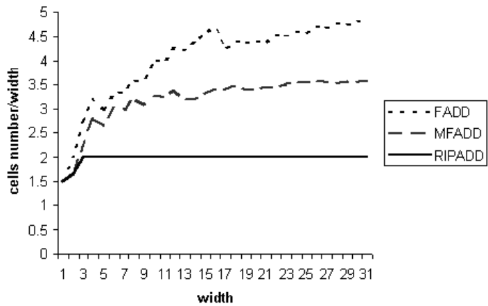
Figure B-10. 54SX/54SX-A/eX/A500K Adder Module Count
