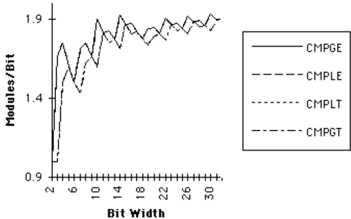
Figure B-16. Comparator Module Count
