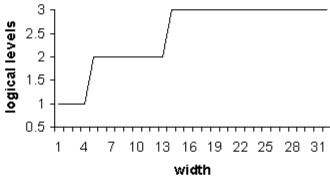
Figure B-23. Incrementer Logic Levels
