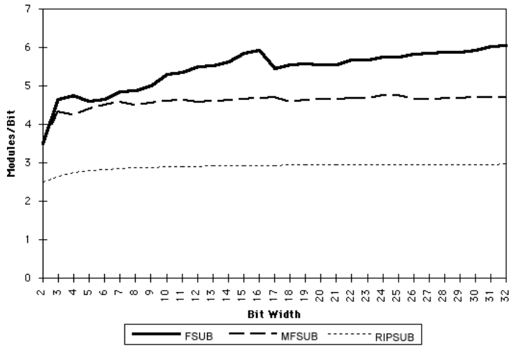
Figure B-12. Subtractor Module Count
