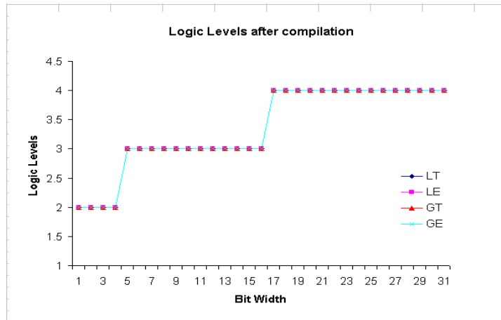
Figure B-19. Logic Levels for 54SX/54SX-A/eX/A500K
