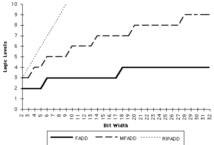
Figure B-9. Adder Logic Level
