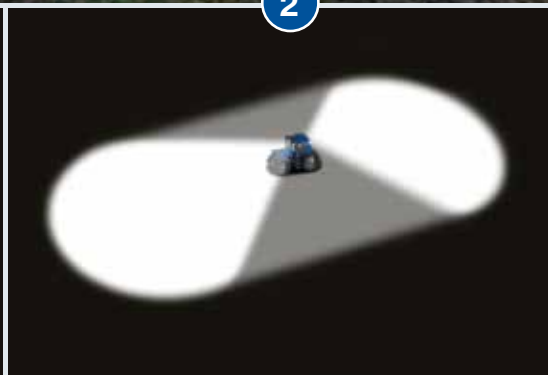
12 LED High-Intensity Work Light Package (12 x 1,950 lumens = 23,400 lumens total)
