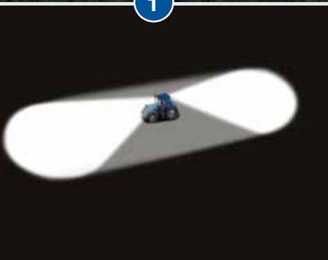
8 LED Work Light Package (8 x 1,125 lumens = 9,000 lumens total)
