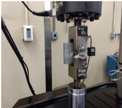
Fatigue crack testing
