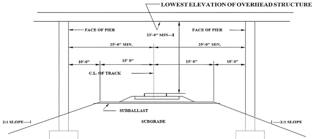
CLEARANCES REQUIRED FOR OVERHEAD STRUCTURES TYPICAL SECTION FOR ROADBED IN FILL (WHERE NO DEFINED DITCHES ARE NEEDED)
