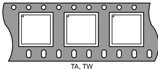
Figure 42. DFN/QFN (LPCC)/ WLCSP-4/XDFN2
