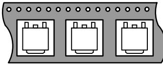
Figure 2. DPAK 16 mm
