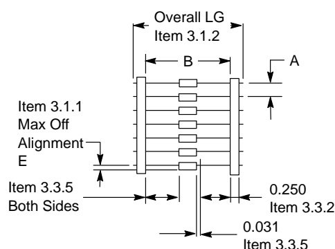
Figure 62. Component Spacing
