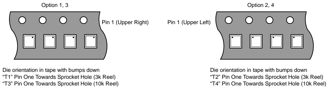
Figure 9. WLCSP, Flip-Chip/DCA
