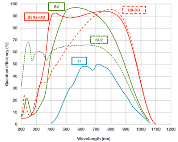
Figure 3: Quantum efficiency of the various models of the IKON L936 ANDOR cameras (courtesy ANDOR).
