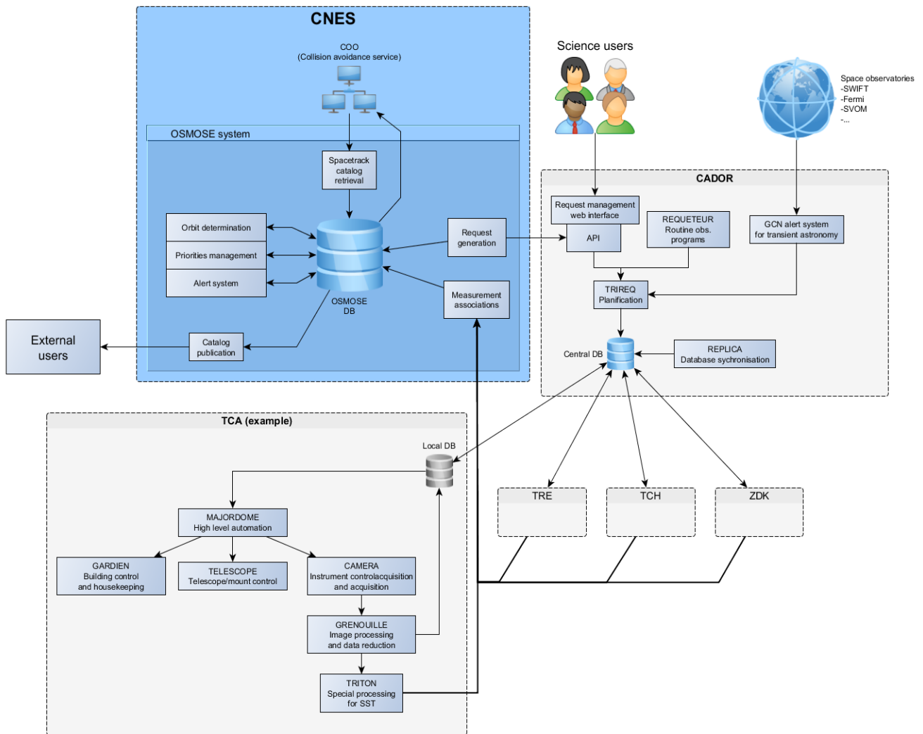
Figure 4: Overview of the software chain of the TAROT system.
