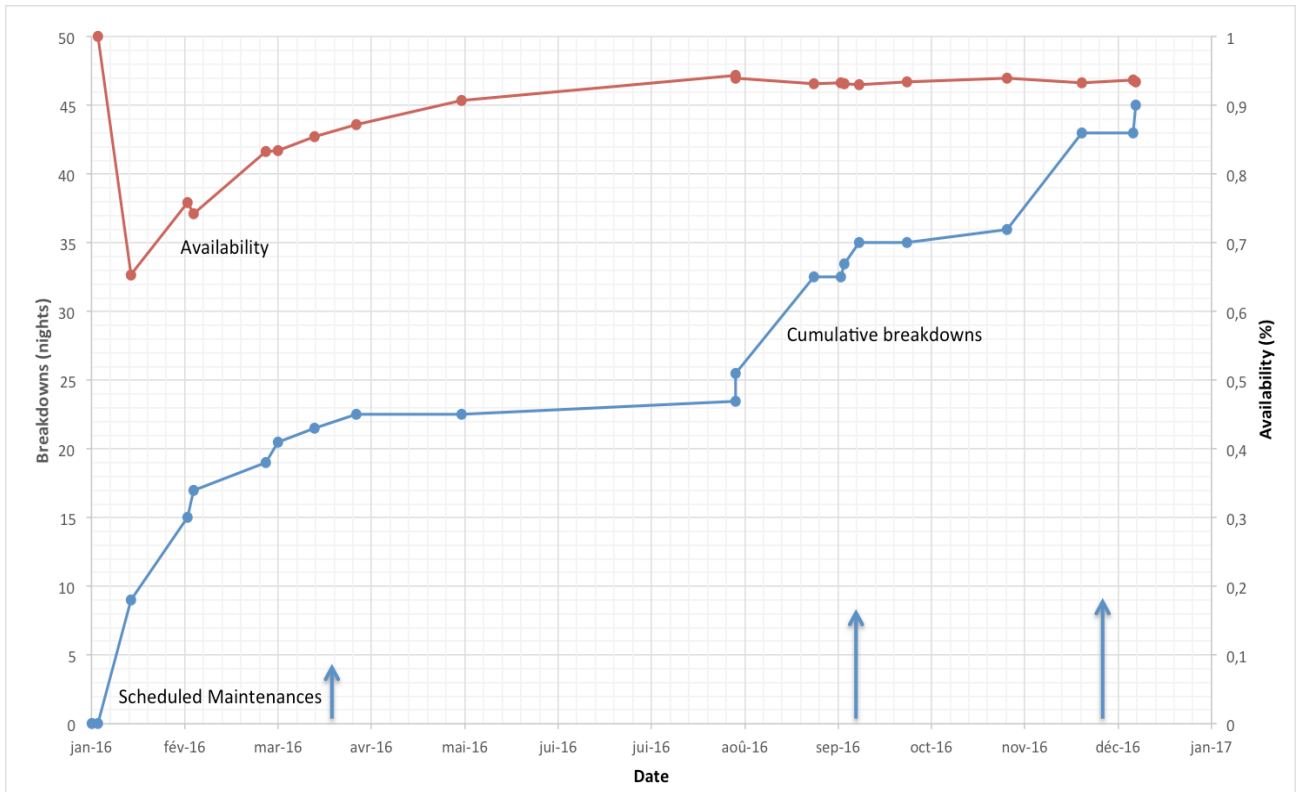
Figure 7: System efficiency statistics of TCA and TCH (see text): the overall efficiency increased to more than 90% after repair in January 2016. The various breakdown (instrumental, hardware or software), are shown together with their duration. The scheduled maintenance periods (March and September for TCA, November for TCH) are also shown with their duration (arrows), but are not taken into account for the computation of the system efficiency. Weather interruptions have not been taken into account.
