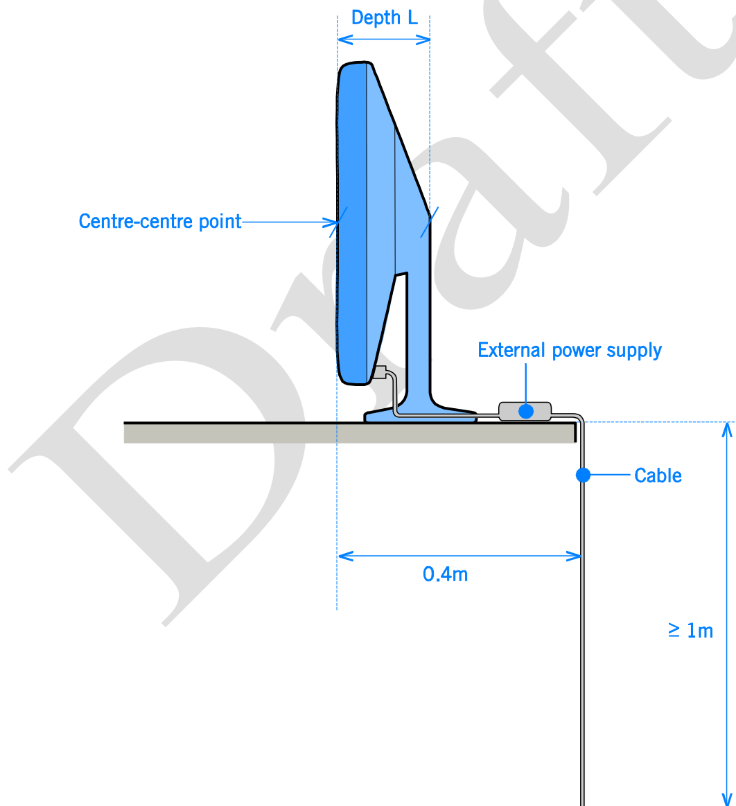
Figure B.4.0.2.2 All-in-one computer with external power supply units.
