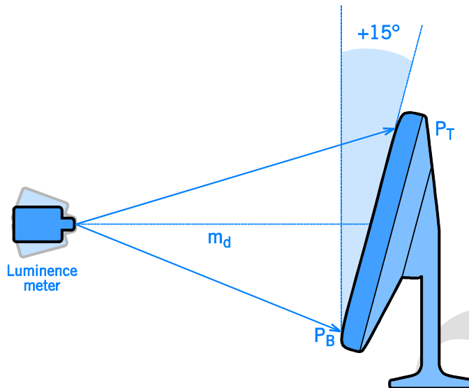
Figure B.2.2.4.3. Side view of the test set-up when the All-in-one computer is tilted \pm 15^\circ . The + rotation is defined as backwards.
