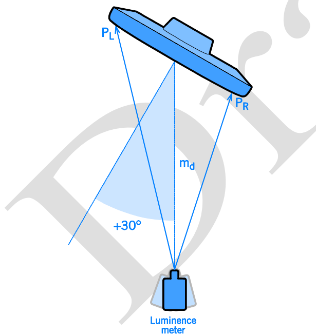
Figure B.2.2.4.2. Top view of test set-up when the All-in-one computer is rotated \pm 30 degrees. The + rotation is defined clockwise.
