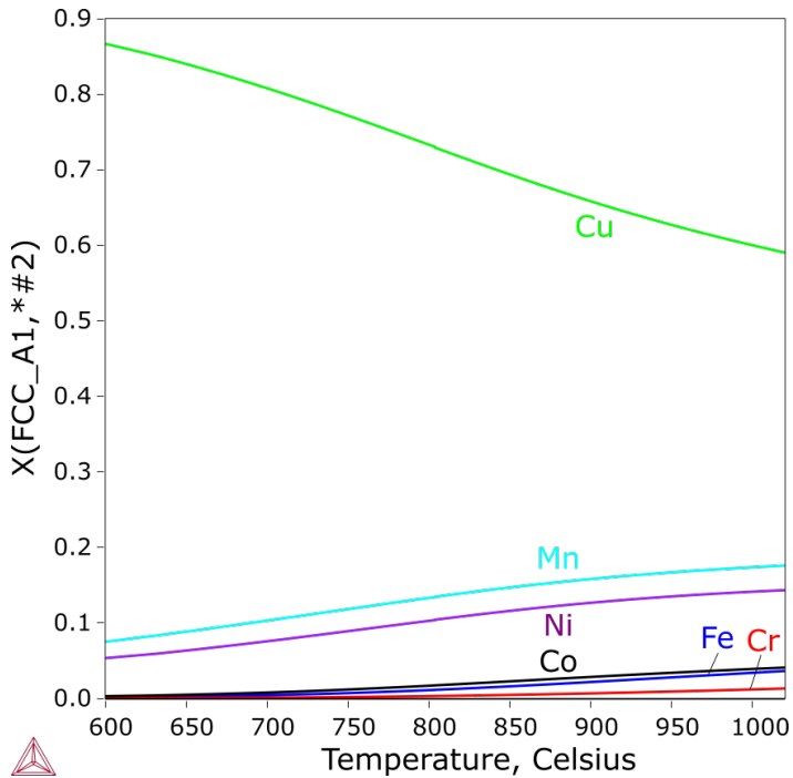
Figure 41: Scheil calculation of the CoCrCuFeMnNi alloy. The composition of the Cu-rich FCC_A1 interdendritic phase from the Scheil simulation of CoCrCuFeMnNi.
