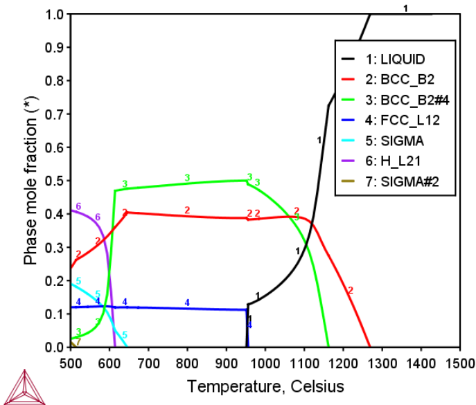
Figure 26: Calculated mole fraction of equilibrium phases at various temperatures in the AlCoCrCuFeMnNiTiV ennead alloy with equiatomic ratio [2017Mao].
