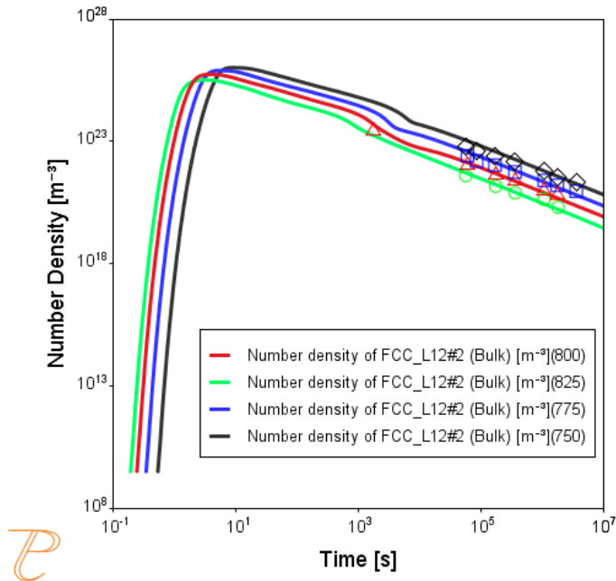
Figure 44: A Precipitation Module (TC-PRISMA) simulation of L1 2 precipitate from the (NiCoFeCr) 94 Ti 2 Al 4 HEA matrix at various temperatures. This shows the number of densities of the L1 2 precipitates. Curves are using the Precipitation Calculator simulation results and symbols are experimental data from [2018Zha].
