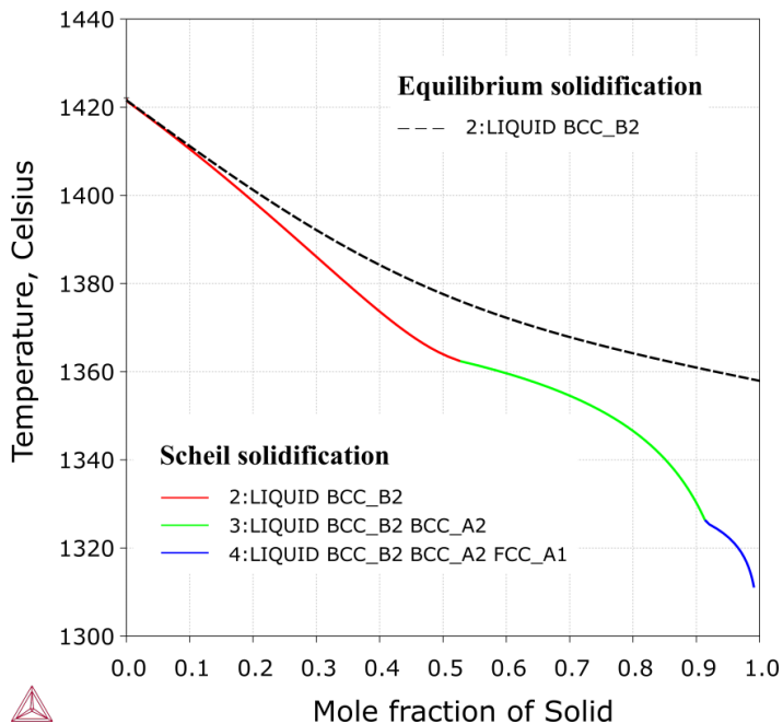
Figure 35: Equilibrium (in dashed line) and Scheil (in solid line) solidification simulations of the \text{CoCrFeNiAl}_{1.1} alloy (21.57 at.% Al) [2018Che].
