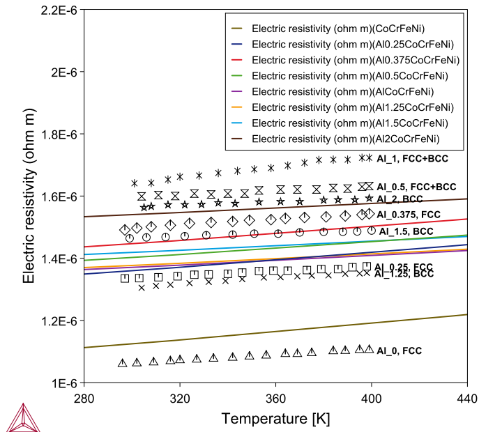
Figure 31: Electrical resistivity of Al_xCoCrFeNi high-entropy alloys at various temperatures. Curves represent (freeze-in) calculations while symbols for experimental data (of as-homogenized alloys at 1373 K) from the literature [2009Chou]. The notation e.g. “Al_0.375, FCC” implies the experimental data for the alloy Al_{0.375}CoCrFeNi with single FCC phase.
