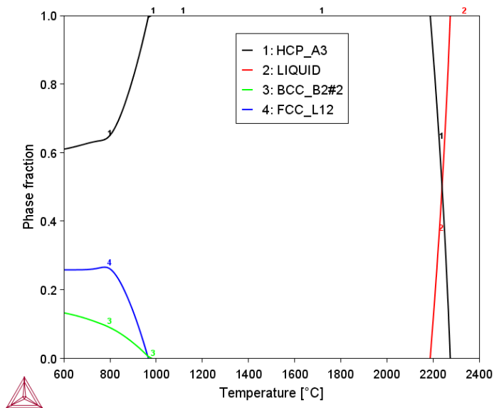
Figure 21: Mole fraction of equilibrium phases at various temperatures in the Ir_{26}Mo_{20}Rh_{22.5}Ru_{20}W_{11.5} high entropy alloy. The experimental validation is reported in [2019Tak].
