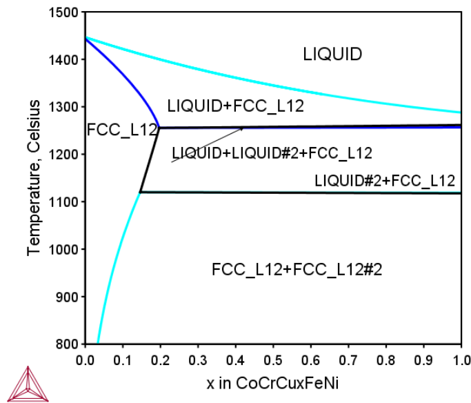
Figure 16: Calculated phase equilibria in the isopleth for the series of the CoCrCu x FeNi quinary alloys, where x=0-1 represents moles of Cu atoms [2017Mao].
