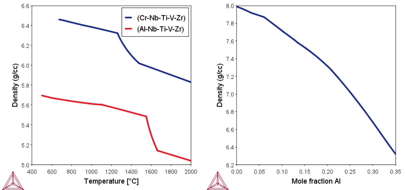
Figure 27: Calculated density of HEAs. (a) Density of CrNbTiVZr and AlNbTiVZr HEAs at various temperatures. The measured room temperature density is 6.57 g/cc for CrNbTiVZr [2013Sen] and 5.79 g/cc for AlNbTiVZr [2015Ste]. (b) Density of Al x CoCrFeNi HEAs at 400°C.
