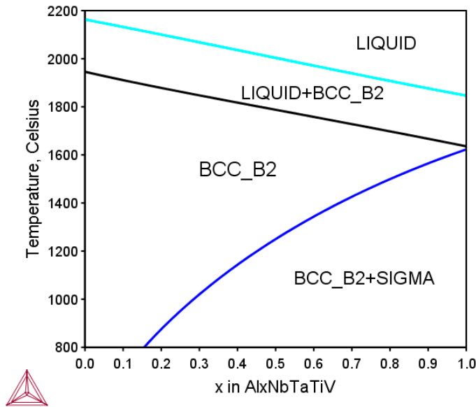
Figure 19: Calculated phase equilibria in the isopleth for the series of the Al x NbTaTiV quinary alloys, where x=0-1 represents moles of atoms of the element Al [2017Mao].
