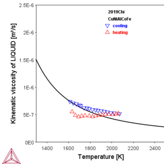
Figure 32: Calculated kinematic viscosity of equiatomic Cu-Ni-Al-Co-Fe alloy along with experimental data from [2019Chi].
