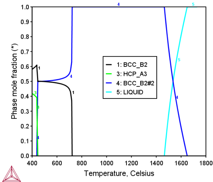
Figure 17: Mole fraction of equilibrium phases at various temperatures in the NbTiVZr equiatomic alloy [2017Mao].
