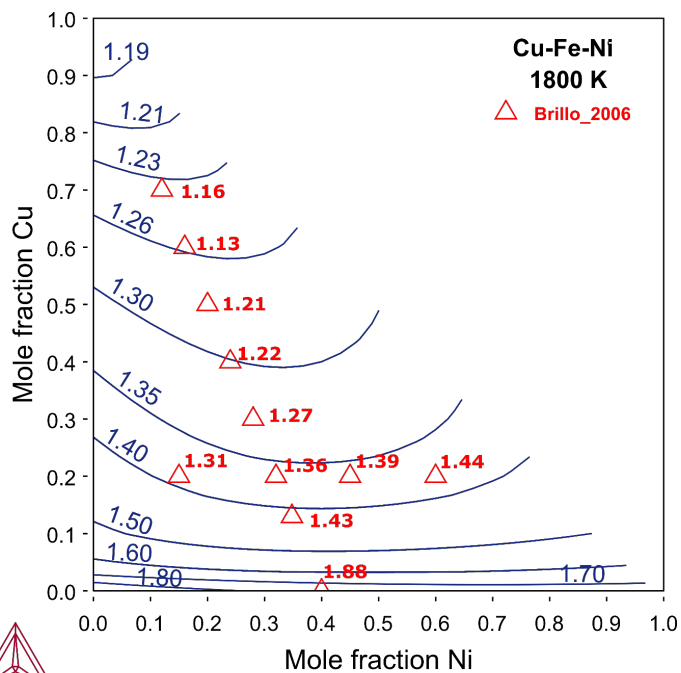
Figure 33: Calculated surface tension of ternary Cu-Fe-Ni liquid at 1800 K in comparison with experimental data of [2006Bri].
