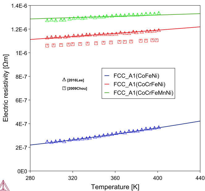
Figure 30: Electrical resistivity of equiatomic FCC medium- and high-entropy alloys at various temperatures. Curves represent calculations while symbols for experimental data from different literature. Each alloy (composition) is assigned a specific color.
