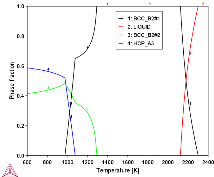
Figure 18: Mole fraction of equilibrium phases at various temperatures in the HfNbTaTiZr equiatomic alloy. The pioneering work of this type of refractory HEA was reported in [2011Sen].
