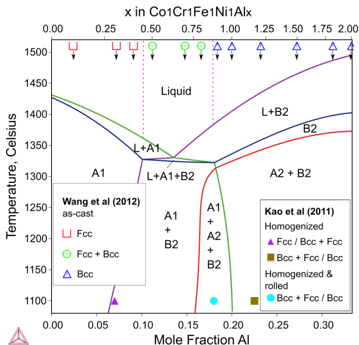
Figure 22: Phase equilibria in the vertical section for \text{CoCrFeNiAl}_x ( 0 < x < 2 ) alloys [2018Che].
