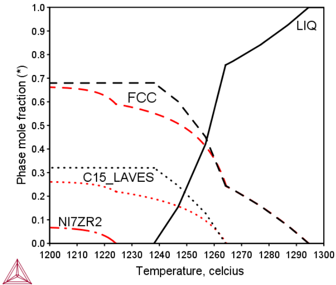
Figure 36: Predicted solid phase mole fractions by equilibrium (black curves) and Scheil simulation (red curves) of the CoCrFeNiZr 0.4 alloy [2017Mao].
