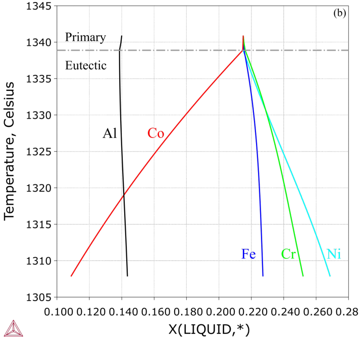
Figure 38: Solidification simulation of the eutectic alloy CoCrFeNiAl 0.65 (13.98 at.% Al): Liquid phase composition from a Scheil simulation [2018Che].
