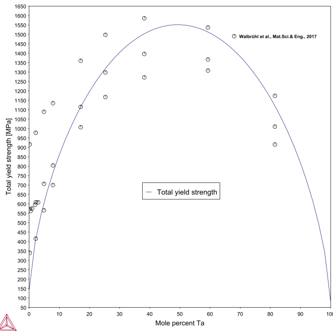
Figure 34: Total yield strength of the Mo-Ta BCC binary alloy in comparison with the experimental data from [2017Wal]. This example is included with Thermo-Calc as a Property Model example named PM_G_06_Yield_Strength_HEA .
