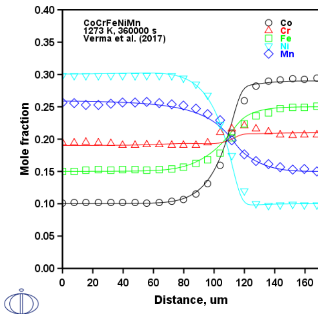
Figure 42: A Diffusion Module (DICTRA) simulated concentration profile of FCC HEA diffusion couple annealed at 1000 °C for 100 hours. Experimental data from [2017Ver].
