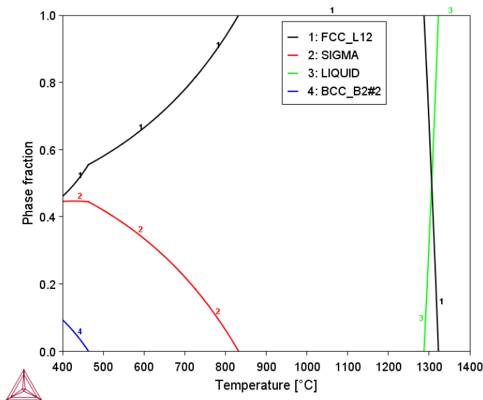
Figure 15: Mole fraction of equilibrium phases at various temperatures in the CoCrFeMnNi equiatomic alloy, a.k.a. the Cantor alloy [2004Can].
