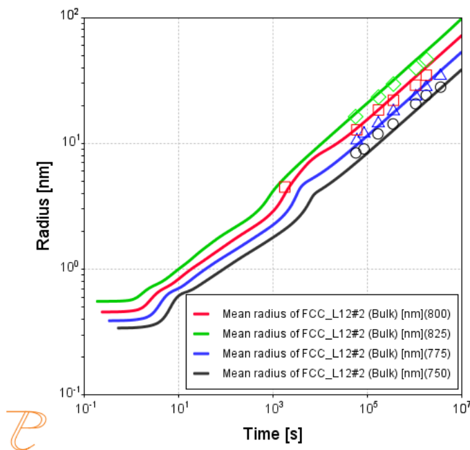
Figure 43: A Precipitation Module (TC-PRISMA) simulation of L1_2 precipitate from the (\text{NiCoFeCr})_{94}\text{Ti}_2\text{Al}_4 HEA matrix at various temperatures. This plot shows the mean radius of the L1_2 precipitates.
