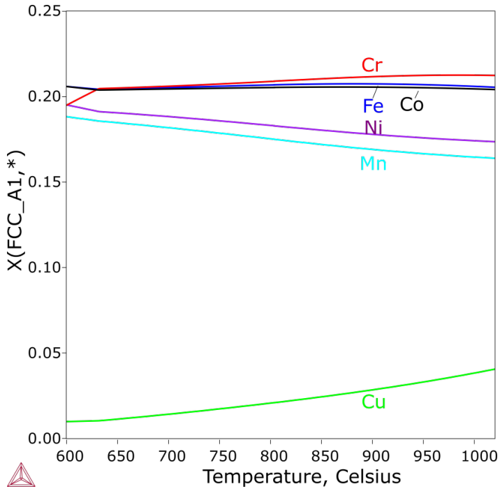
Figure 40: Scheil calculation of the CoCrCuFeMnNi alloy. The composition of the Cu-lean FCC_A1 dendritic phase from the Scheil simulation of CoCrCuFeMnNi.
