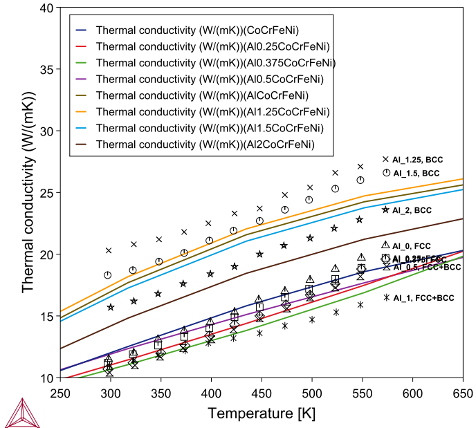
Figure 29: Thermal conductivity of Al_xCoCrFeNi high-entropy alloys at various temperatures. Curves represent (freeze-in) calculations while symbols for experimental data (of as-homogenized alloys at 1373 K) from the literature [2009Chou]. The notation e.g. “Al_1.25, BCC” implies the experimental series for the alloy Al_{1.25}CoCrFeNi with BCC structure.
