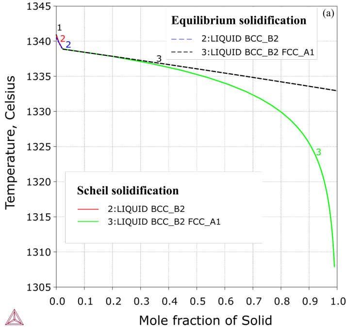
Figure 37: Solidification simulation of the eutectic alloy CoCrFeNiAl 0.65 (13.98 at.% Al): Phase formation sequence and solid phase fractions from equilibrium (in dashed line) and Scheil simulation (solid line) [2018Che].
