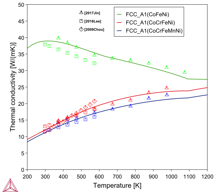
Figure 28: Thermal conductivity of equiatomic FCC medium- and high-entropy alloys at various temperatures. Curves represent calculations while symbols for experimental data from different literature. Each alloy (composition) is assigned a specific color.
